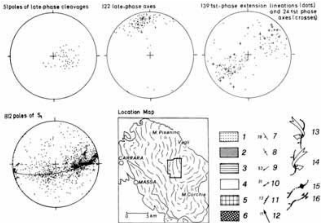
Figure 23 - Stereograms and legend for the geological map of Fig. 24. 1: Metasandstones (Upper Oligocene); 2: Calcschists, cherts, phyllites, (Dogger-Eocene); 3: Cherty Limestones (Middle-Upper Liassic); 4: Marble (Lower Liassic); 5: Dolomite (Upper Triassic); 6: Paleozoic Phyllites; 7: S1 foliation; 8: S1 foliation vertical; 9: D1 stretching lineation; 10: D1 minor fold axes attitude and D1 intersection lineations; 11: S2 foliation; 12: D2 minor fold axes attitude and D2 intersection lineations; 13: axial plane trace of the Arni synform; 14: axial plane trace of the Arni antiform; 15: Minor D2 antiform axial plane traces; 16: Minor D2 sinform axial plane traces.
