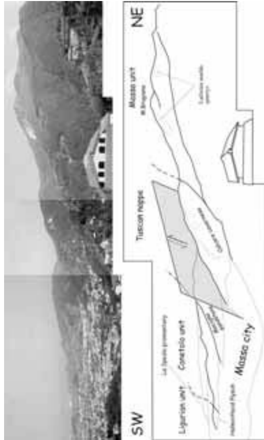
Figure 14 - Panoramic view from San Carlo near Massa. Stop 2.1.
