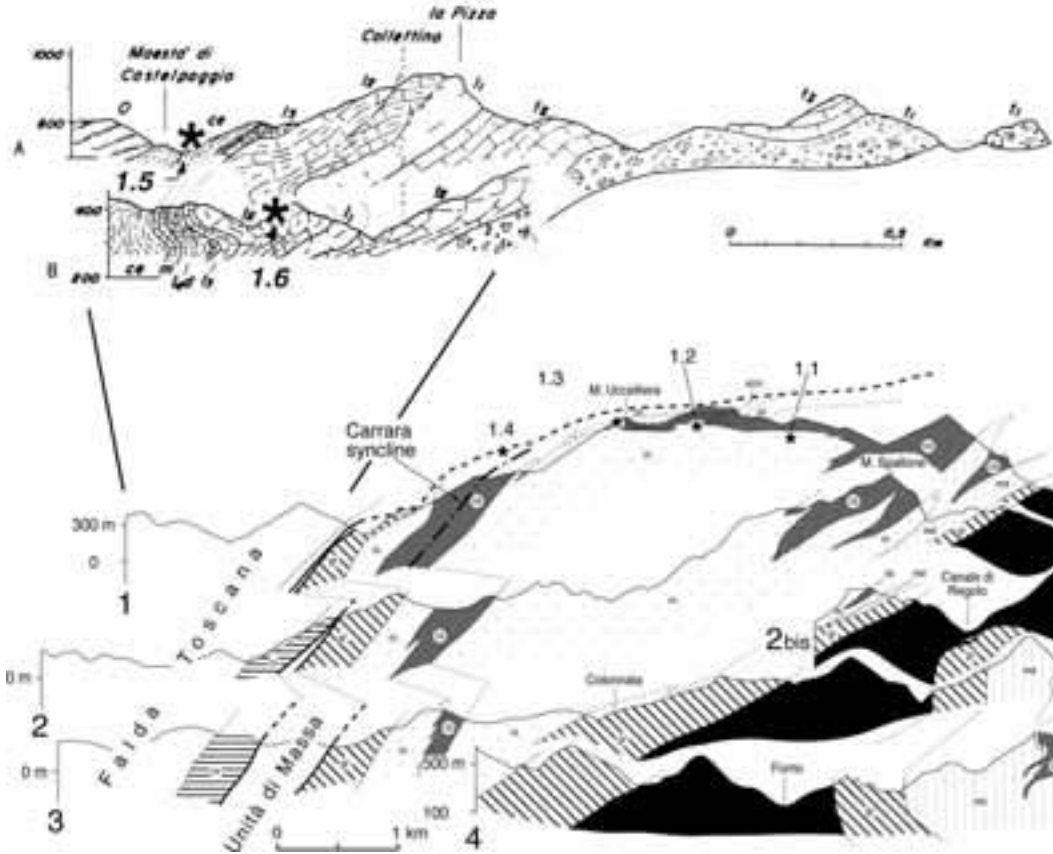
Figure 10 - Geological cross section in the area of Fig. 9. A and B sections after Decandia et al., 1968. t1: "Calcare cavernoso", t2: Rhaetavicula contorta limestones, l1: "Calcare massiccio", l2: Angulati limestone, l3: "Rosso Ammonitico", Posidonia marls, m: cherts, ce: Scaglia, o: "Macigno" flysch. Legend for sections 1-3: B: Paleozoic basement, gr: dolomites (Norian-Rhetian), md: dolomitic limestones (Lower Liassic), m: marbles (Lower Liassic), cs: cherty limestones (Liassic), sc: "Scisti sericitici", scm: nummulite limestones, cv: "Calcare cavernoso".
