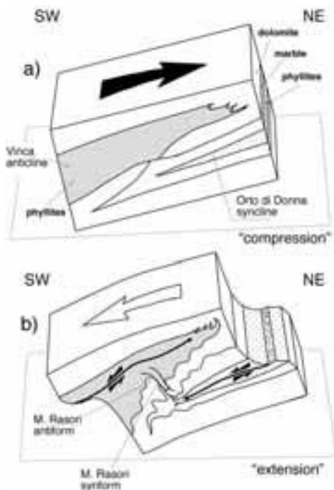
Figure 19 - D1 and D2 deformation interference in the Frigido valley. Late structures in the inverted limb of the D1 Vinca anticline are interpreted as “transfer folds” between two ductile shear zones.
