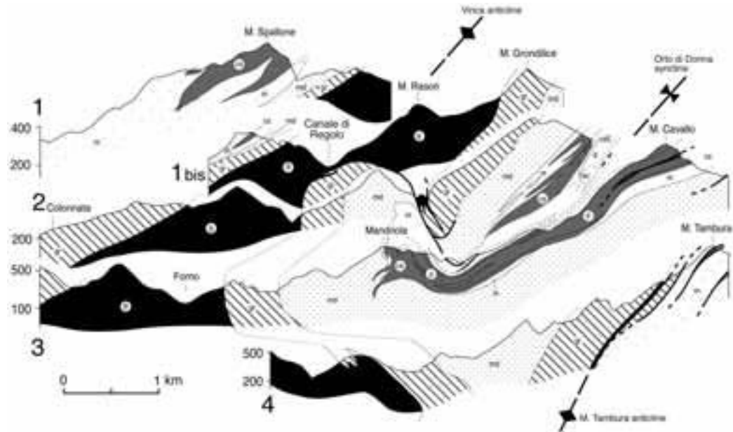
Figure 17 - Geological cross section in the Frigido valley, central Alpi Apuane. See Fig. 15 for section traces. Legend as in Fig. 10.
