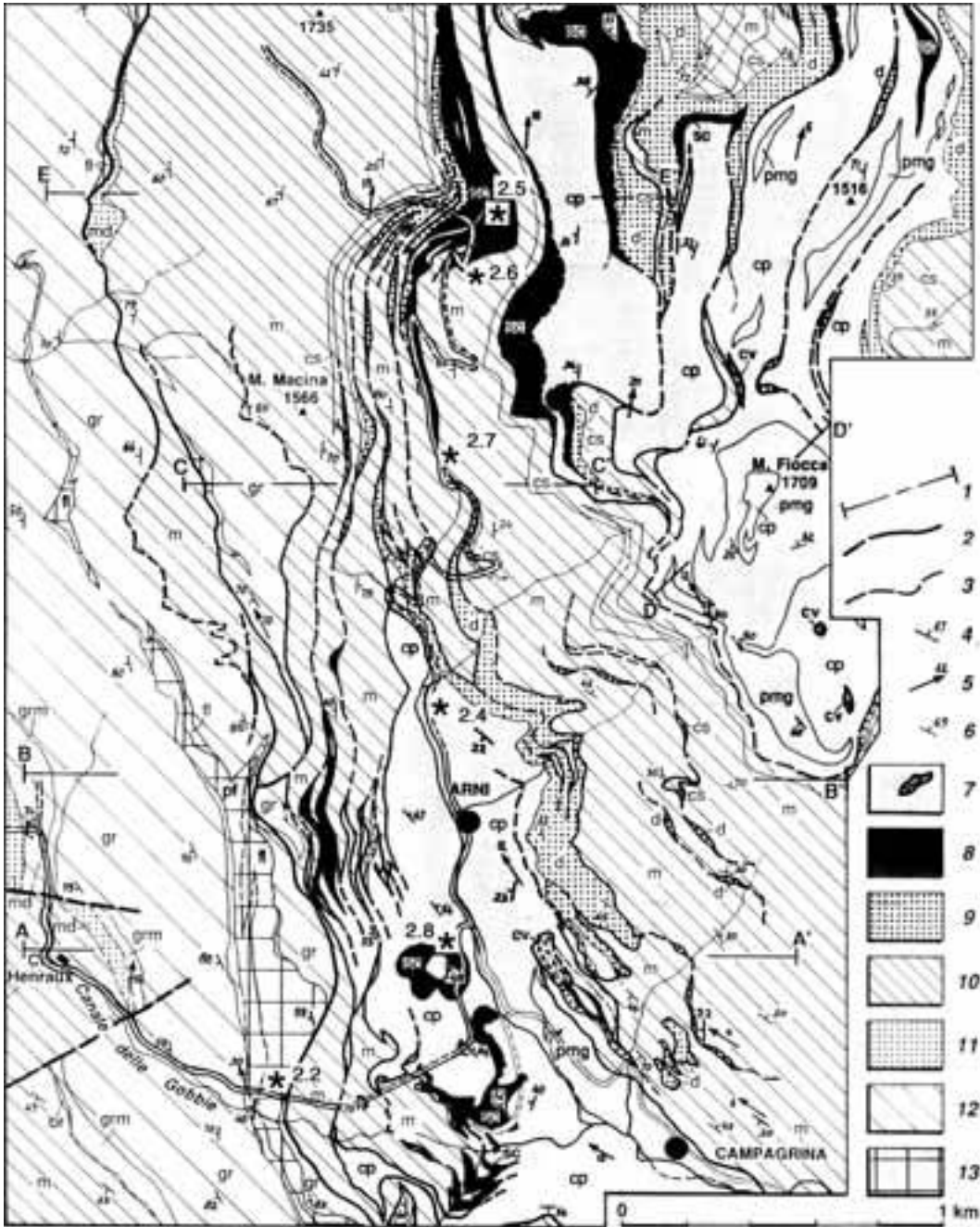
Figure 21 - Geological map in the Arni valley. 1: traces of sections of Fig. 22; 2: faults; 3: tectonic contacts; 4: D2 foliation; 4: D2 fold axis; 6: D1 foliation; 7: "Pseudomacigno" metasandstones (pmg), calcschists (cp), "Calcarea cavernoso" (cv); 8: "Scisti sericitici" phyllites (sc); 9: Cherts (d); 10: Calcschists (csc), cherty limestone (cs), marble (m); 11: Dolomitic marble (md); 12: Seravezza Breccia (br), "Grezzoni" dolomite (gr), "Verrucano (fV+Vr); Paleozoic phyllites (pf+fl).
