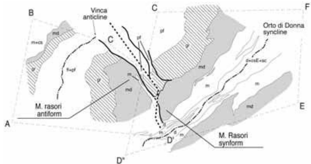
Figure 18 - Profile in the Frigido valley for the detail area indicated in Fig. 15.
