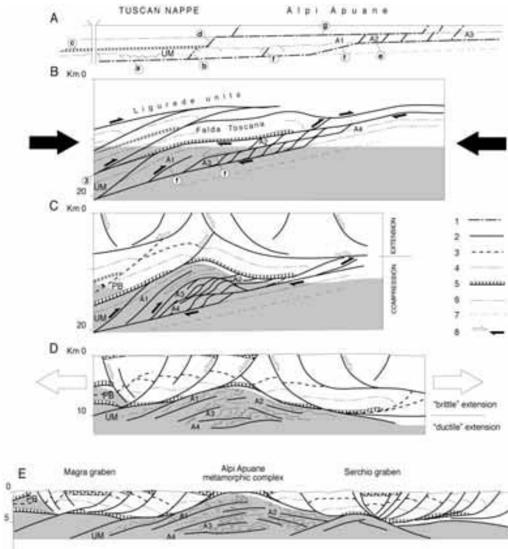
Figure 7 - Tectonic evolution of the Alpi Apuane region.
