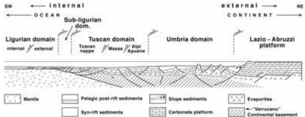
Figure 3 - Palinspastic reconstruction of the western continental margin of Apulia during the late Jurassic (after Bernoulli, 2001, modified). Internal and external is referred to the top-the-NE transport direction of the Tertiary tectonics. Location of this section is approximately located in Fig. 1a.
