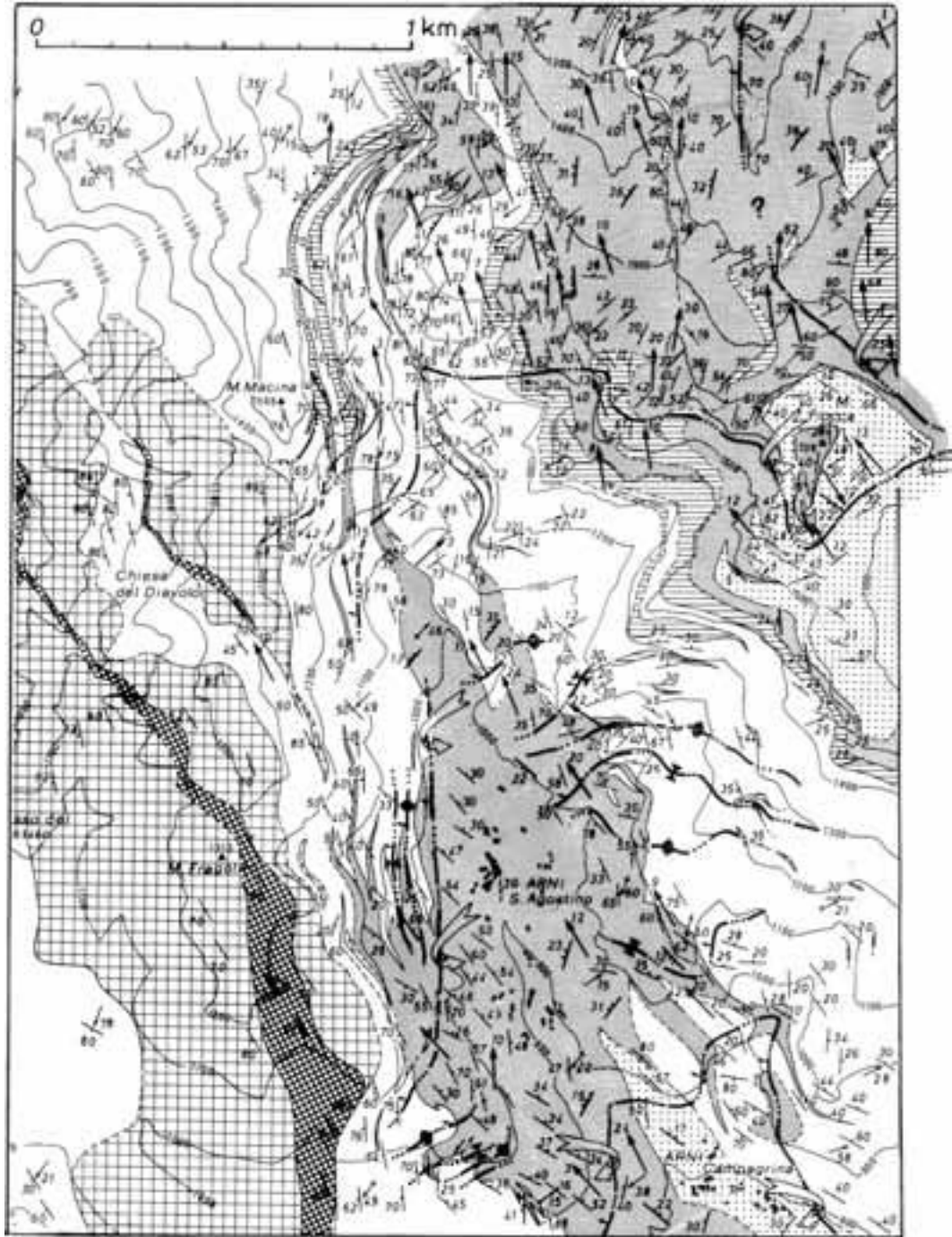
Figure 24 - Structural map of the Arni valley. See Fig. 23 for legend.
