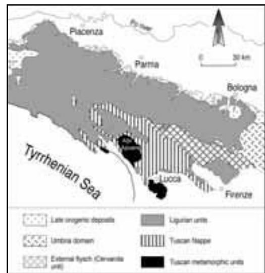
Figure 4 - Tectonic units in the Italian northern Apennines.
