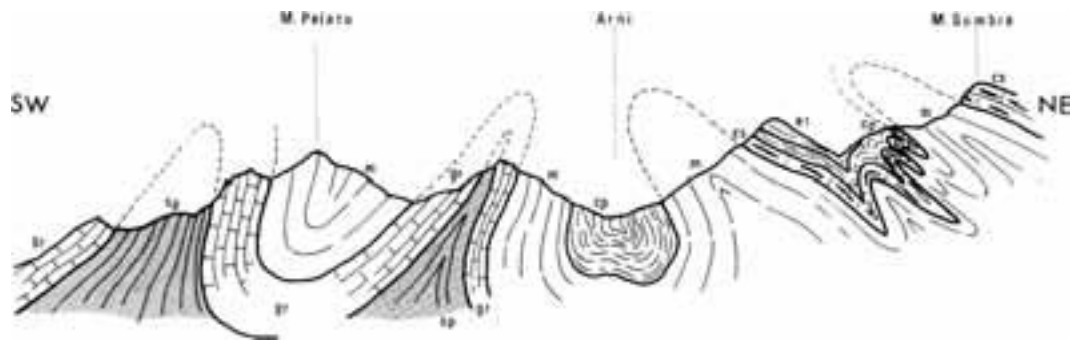
Figure 20 - The structure of the Arni valley after Lotti (1881a, b). sp: Paleozoic phyllites, gr: Triassic dolomites, m: marbles, cs: certy limestones, cp: calcschists, ar: metasandstones flysch.
