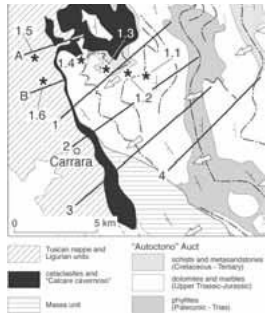
Figure 9 - Tectonic sketch map of the area north of Carrara. First day stops and traces of Fig. 10 sections are located.
