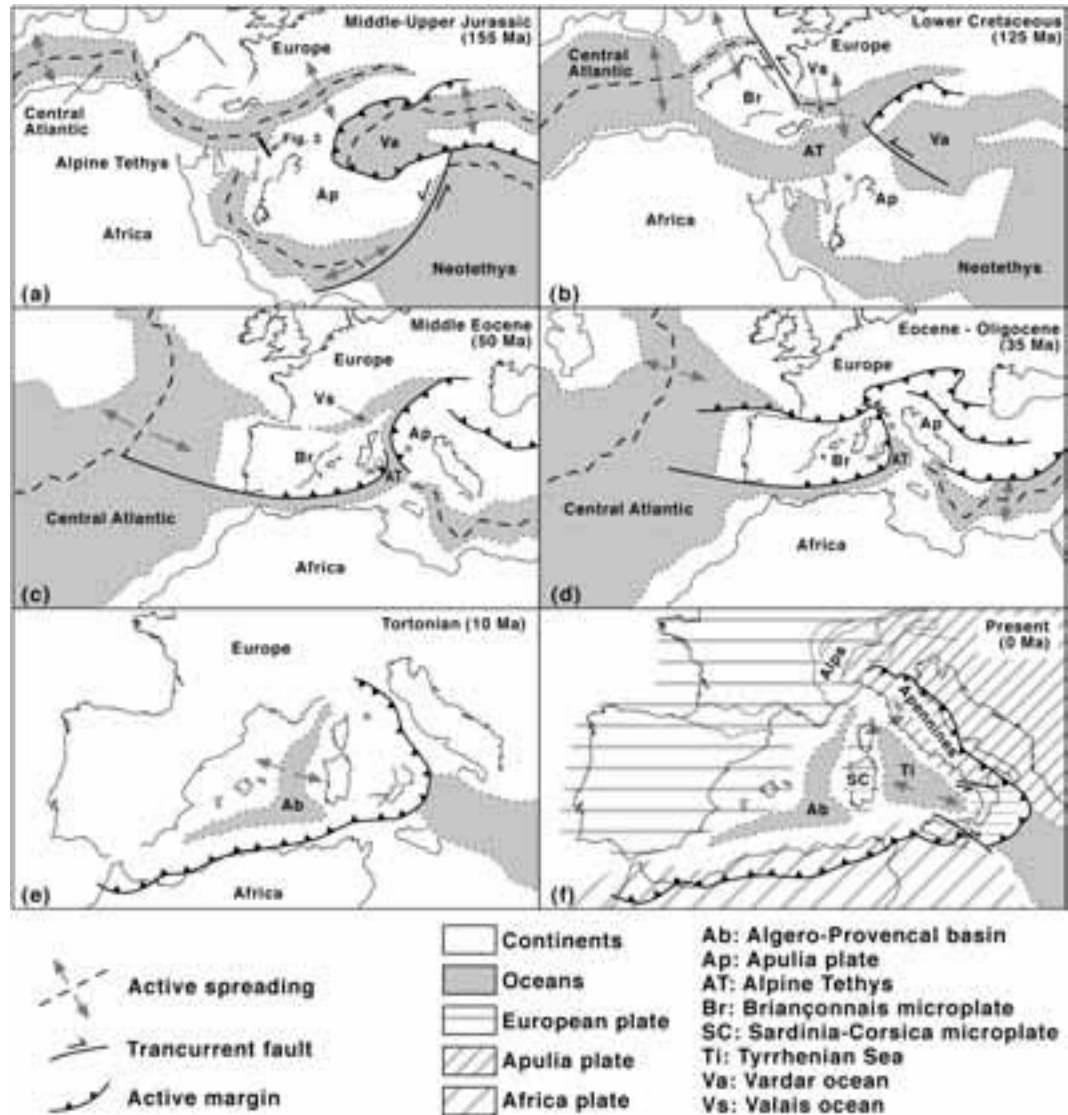
Figure 1 - Plate reconstruction for the western Mediterranean area, after Stampfli et al. (2001), modified.
