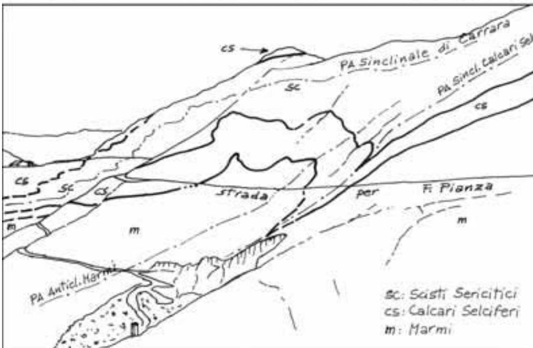
Figure 11 - View of the Murlungo-Zucco del Latte area. Parasitic folds of the normal limb of the D1 Carrara syncline are deformed by the D2 Murlungo synform and antiform.
