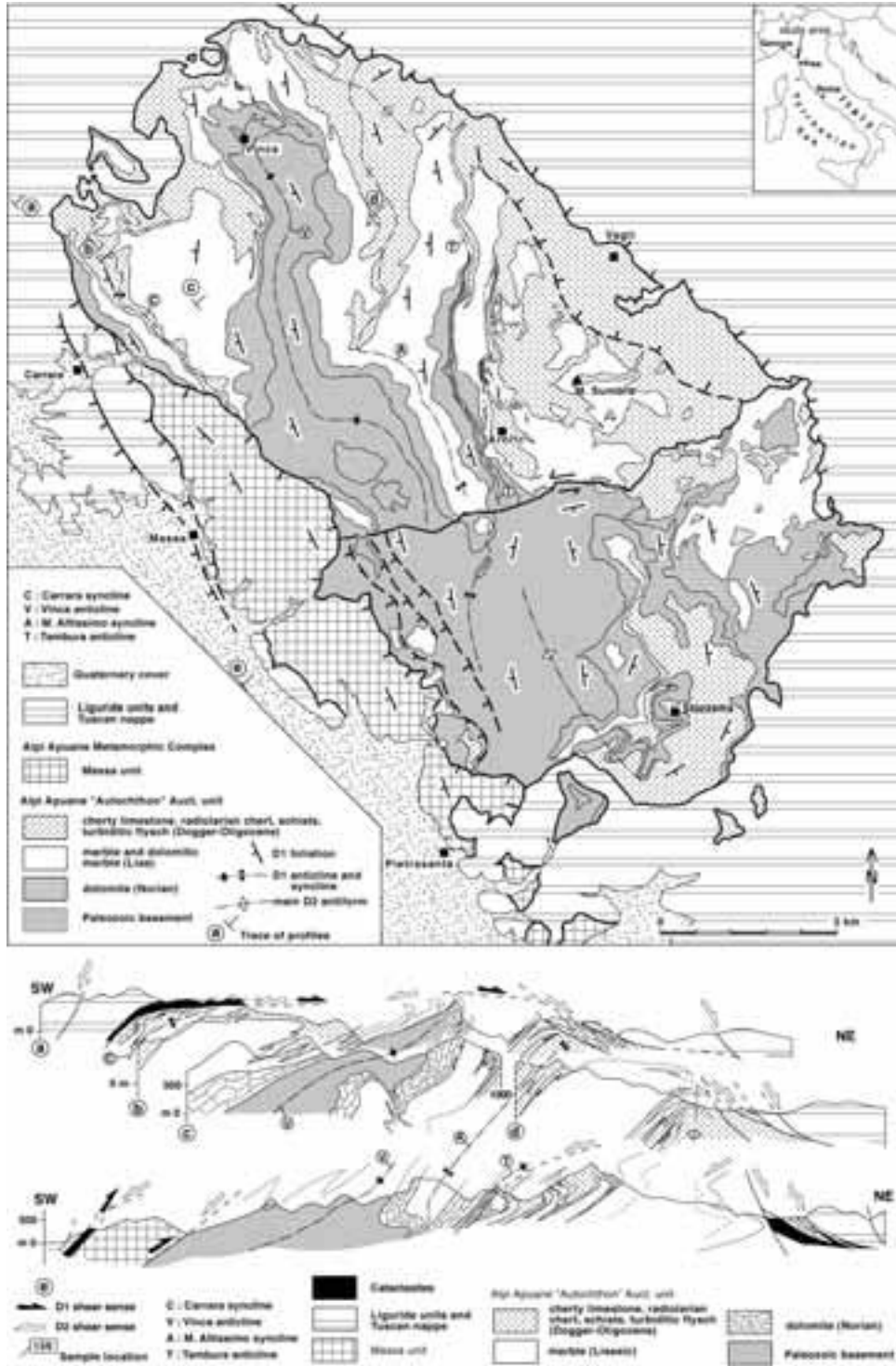
Figure 6 - Tectonic map of the Alpi Apuane area.
