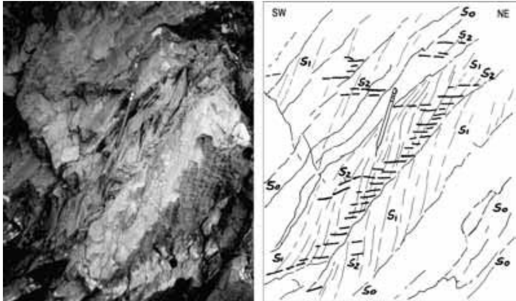
Figure 12 - S 0 , S 1 and S 2 interference in the road cut at La Maestà di Castelpoggio. S 0 -S 1 relationships indicate a top-NE facing for D 1 fold, S 0 -S 2 relationships indicate top-SW facing for D 2 fold.
