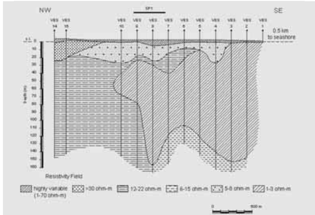
Figure 12 - Resistivity section and seismic profile SPI locations (Balìa et al., 2003).
