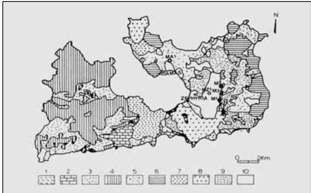
Figure 2 - Simplified geological map of the island: (1) Metamorphic basement (Middle-Upper Pliocene), (2) Transgressive marine sediments (Upper Miocene - Lower Pliocene), (3) Basal pyroclastic series (Middle-Upper Pliocene), (4) Complex domes and lava flows, (5) Pyroclastic series (lower Pleistocene). (6), (7) Lava domes. (8) Rhyolitic complexes (Upper Pleistocene), (9) Products of phreatic activity, (10) Alluvium. The locations of the deep boreholes are marked (Fytikas, 1977; 1989).
