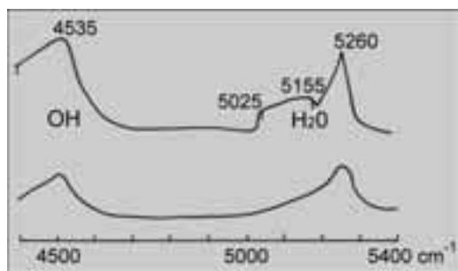
Figure 3.7 - Near infra-red spectra of Golobradovo perlite (sample G73) before (top, according to Yanev and Zotov (1996) and after expanding at 1300°C (bottom).
