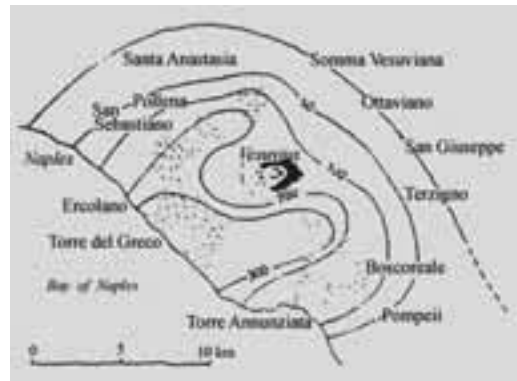
Figure 22 - The thickness of the total surge deposits (in meters) with isopachous lines. Distribution of pyroclastic flows (dotted lines) is also shown (from Sigurdsson et al., 1985).
