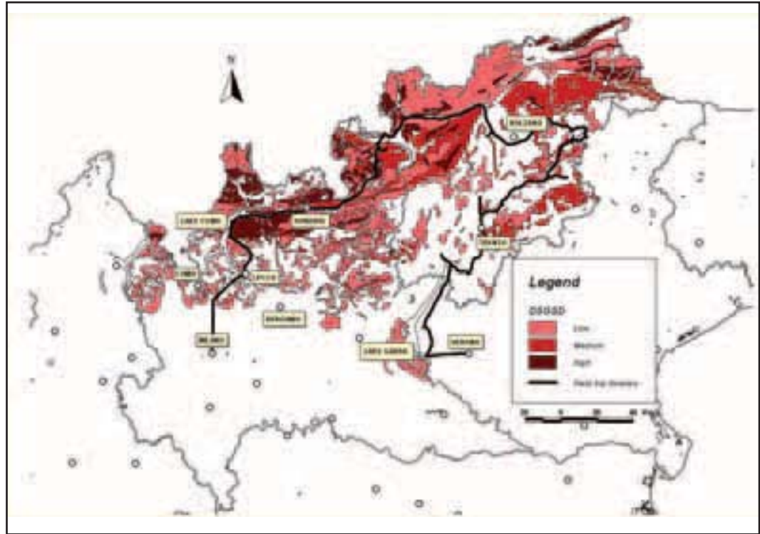
Figure 2 - Map of the field trip area showing the DSGSD index (n. of DSGSD per km 2 , per each geological unit), calculated for a total of 129 events existing in the IFFI database. The index of the different units ranges from 0.000 to 0.046
