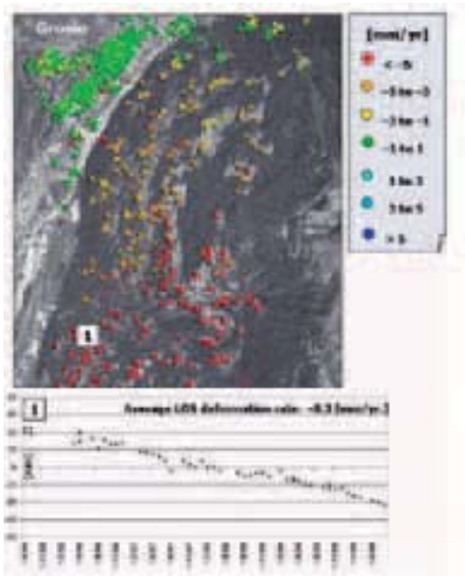
Figure 26 - Padrio-Varadega DSGSD. PS average deformation rates depicted on orthorectified photography. Displacement time series of an individual PS.
