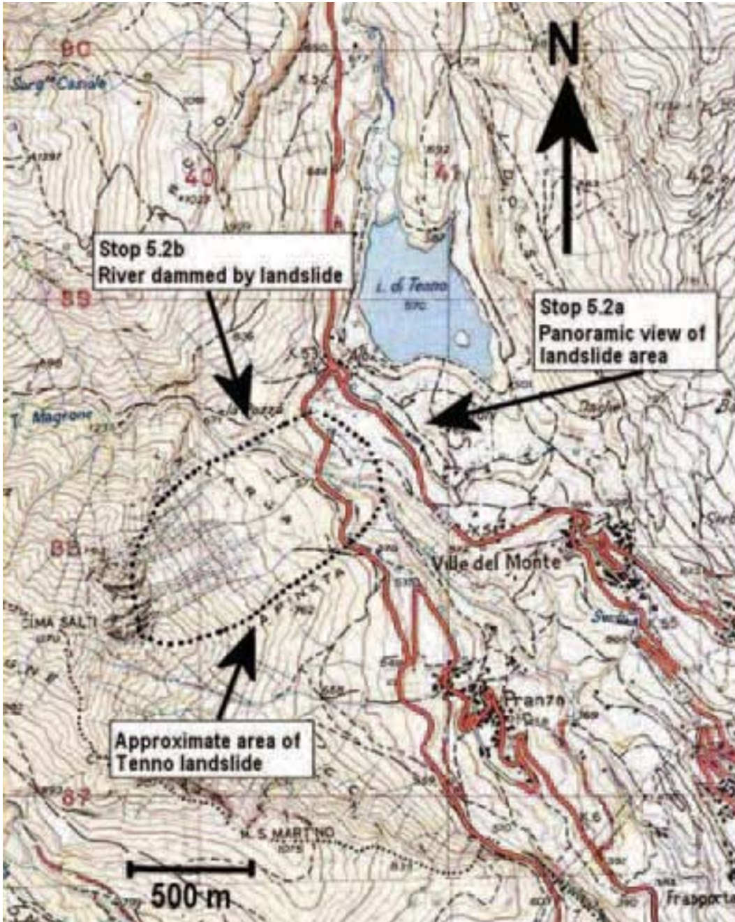
Figure 67 - Excerpt of the Tenno area topographic map. Approximate area affected by the landslide (dotted line) and field trip stops are indicated.
