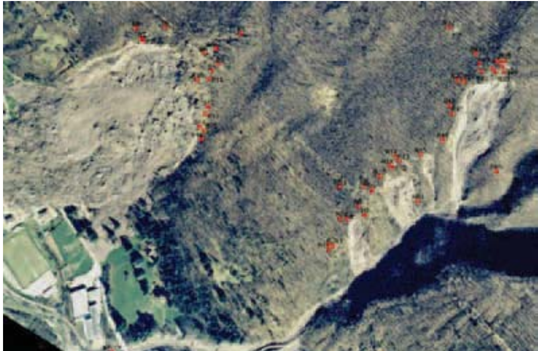
Figure 15 - Digital ortophotograph of the slope, showing the position of the optical benchmarks used to monitor movements.
