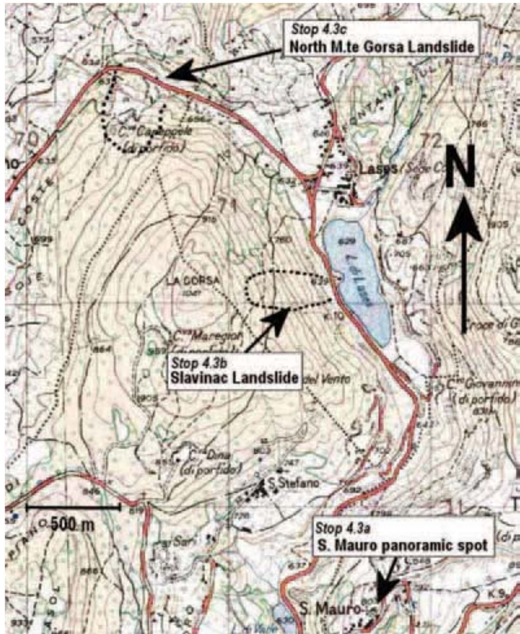
Figure 58 - Excerpt of the Lases area topographic map. Approximative extent of the visited landslides and field trip stops are indicated
