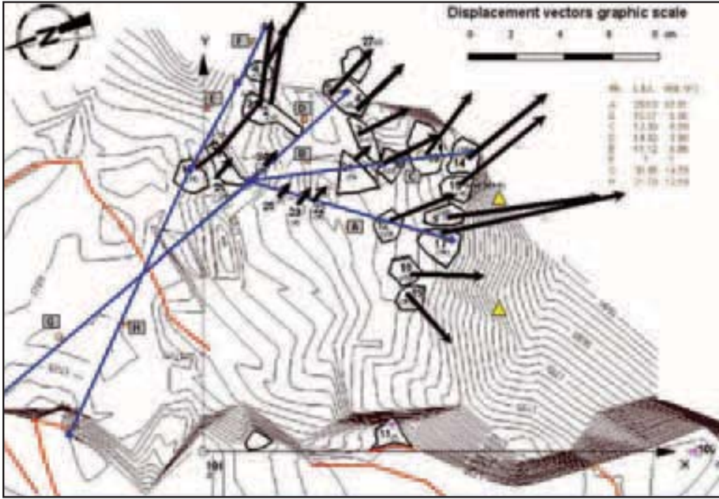
Figure 56 - Monitoring network on Forte Buso Landslide. Letters from A to H are referred to extensometers. Polygons with numbers represent rock blocks under topographic control: arrows are cumulative displacements on horizontal plane and Triangles are inclinometers.
