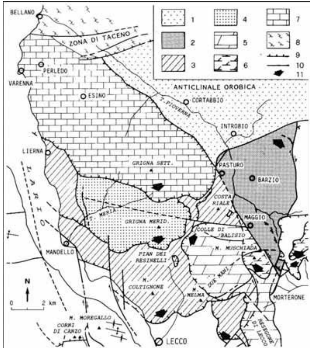
Figure 8 - Structural map of the Grigne group and the Valsassina 1) Orobic anticline Paleozoic. 2) Barzio zone medium and upper Trias. 3) Coltignone Slab. 4) Southern Grigna slab. 5) Resegone-Muschiada Slab. 6) Due Mani slab. 7) Northern Grigna Slab. 8) Orobic basement. 9) Thrusts. 10) Faults. 11) Direction of the overlapped slabs.
