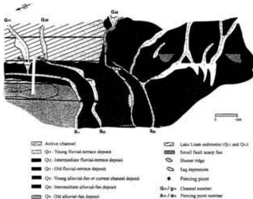
Fig. 19 - Detailed geologic map showing offset gullies in the vicinity of Trench 2. Piercing points used to calculate slip are marked as solid dots on the map. We use uppercase "G" for upstream gullies east of the fault and lowercase "g" for downstream channels west of the fault trace. Likewise, projected piercing points are uppercase letters east of the fault and lowercase letters west of the fault. The gullies are numbered from north to south. See Figures 3 and 4 for location of map.
