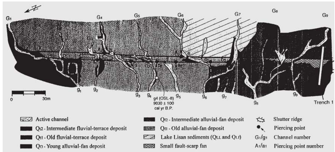
Figure 18 - Detailed geologic map showing offset gullies developed on the Q_2 alluvial fan surface. Piercing points used to calculate slip are marked as solid dots on the map. We use uppercase "G" for upstream gullies east of the fault and lowercase "g" for downstream channels west of the fault trace. Likewise, projected piercing points are uppercase letters east of the fault and lowercase letters west of the fault. The gullies are numbered from north to south. See Figures 3 and 4 for location of map.
