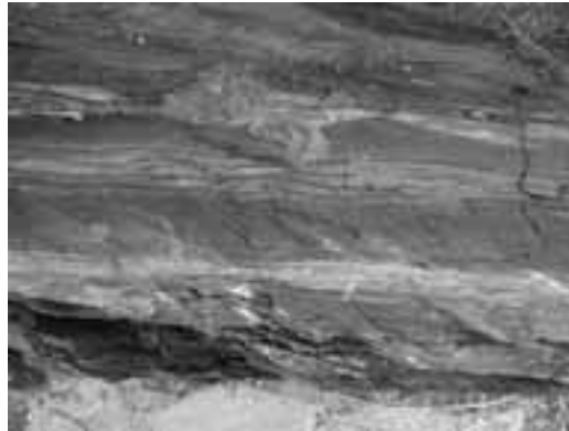
Figure 10 - Banded sandstone lithofacies (arenarie zonate) of the Macigno: centimetric arenaceous layers (the whitish ones) pass fastly to pelites (dark). Cross, piano-parallel and ripple laminations or ripple laminations are present. The ar/pe rate is always in favor of the last one. In some cases a marly or carbonate component is present.
