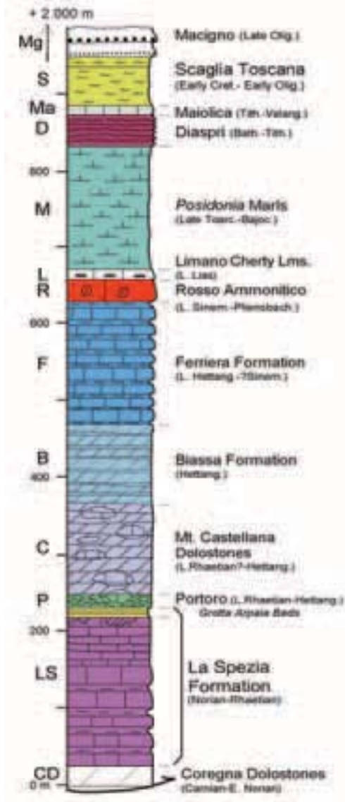
Figure 8 - Columnar section of the Tuscan Nappe in the La Spezia area. CD – dolostones and dolomitic limestones; LS – dark grey calcareous beds with marly or dolomitic interbeds; P - dark grey calcilutites with whitish-yellowish dolostone; C – whitish massive saccharoid dolostone of late diagenetic origin on dark grey bedded calcilutites; B – whitish grey bedded limestone with more dark and pinkish alternance; F – well bedded dark grey marly limestones and calcareous marls; R – red limestones, sometime nodular, ammonitic limestones and marls; L – whitish grey limestone with rare grey cherts; M – grey-green, yellowish marls and whitish limestones; D – red and grey-green radiolarites; Ma – whitish well bedded calcilutites with nodules and layer of gray cherts; MG – turbidite sandstones and pelites.
