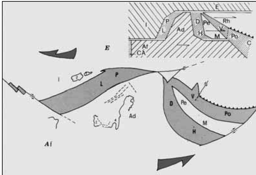
Figure 2 - Continental blocks and oceanic basins in the Mediterranean area at about 160 Ma. Scheme of plate kinematics and paleogeographic reconstruction: Continental areas Ad - Adria; Af - Africa; CA - Central Atlantic; E - Europe; I - Iberia; M - Menderes; NA - North Atlantic; Pe - Pelagonian massif; Rh - Rhodope. Ophiolite basins LP - Ligurian-Piedmont; DH - Dinaric-Hellenic; C Po - Caucasian-Pontic (Abbate et al. 1986)
