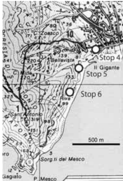
Figure 13 - Stop location map from Monterosso to P. Mesco
