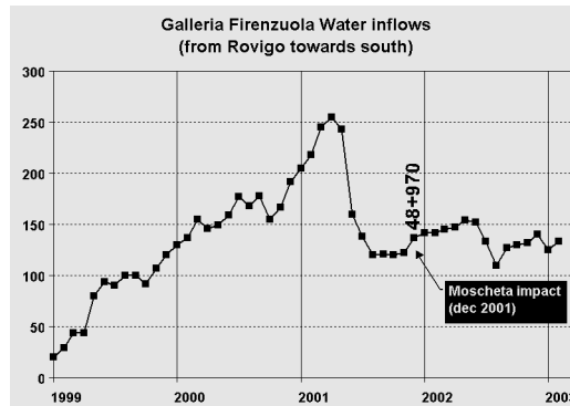
Figure 14 - seepage flow rate in northern side of Firenzuola tunnel (based on CAVET data)
