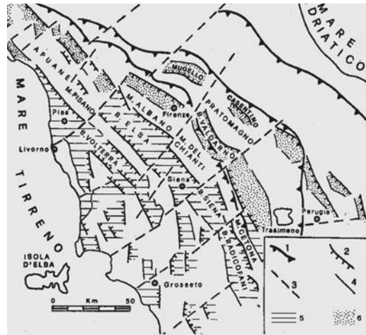
Figure 2 - Main Neogenic and Quaternary basins in the Northern Apennines. 1=thrusts; 2=master faults on basin borders; 3=transversal tectonic lines; 4=minor faults; 5=Mio-pliocene basins filled by continental and marine deposits; 6=Plio-Pleistocene basins filled by fluvio-lacustrine deposits (after Bossio et alii, 1992, in Bortolotti V., 1992, modified)
