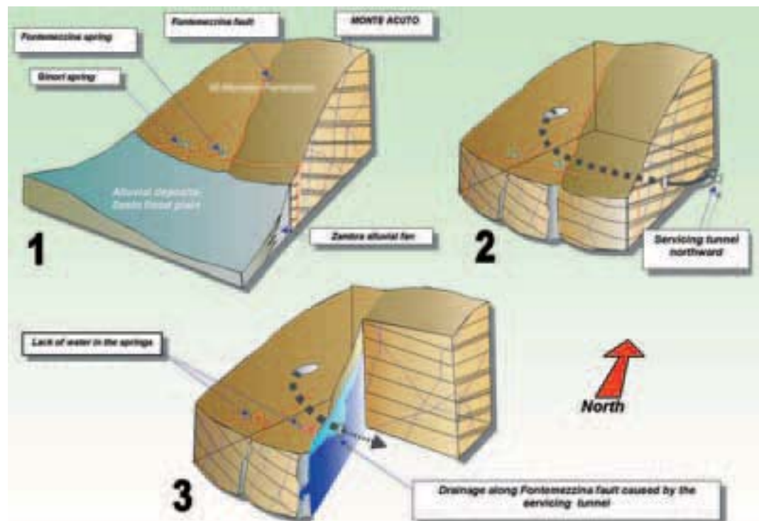
Figure 7 - Block-diagram showing the drainage caused by the boring of the servicing tunnel.
