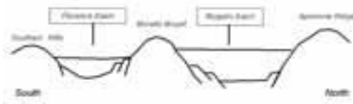
Figure 4 - Schematic cross-section SSW-NNE showing the Florence and Mugello basins
