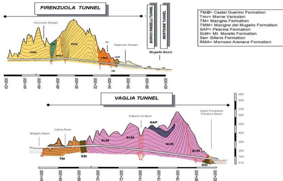
Figure 3 - Cross section along a part of the Tuscan stretch of the new railway (after Gambelli 2002, modified)
