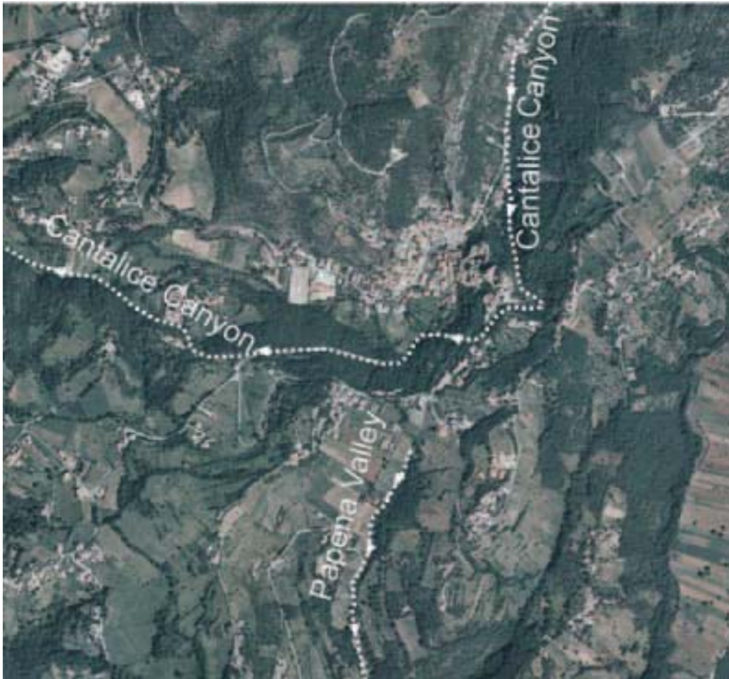
Figure 7 - The Cantallice and Papena Canyons
