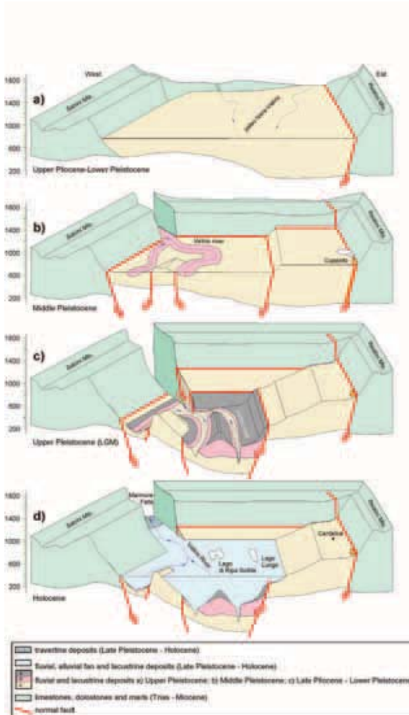
Figure 2 - Landscape evolution of the Rieti basin in four scenarios (a, b, c and d) since the Late Pliocene.
