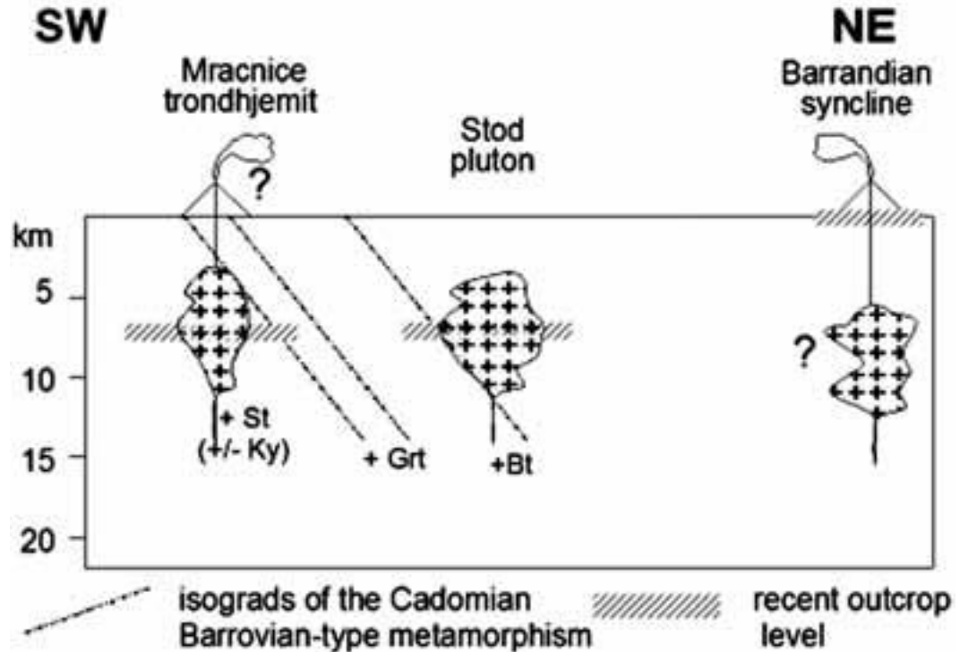
Figure 14 - Cambrian plutons intruded into a tilted crustal profile (between the West Bohemian shear zone and the Barrandian syncline) as is indicated by the tilted metamorphic isograd planes (after Zulauf, 1997).
