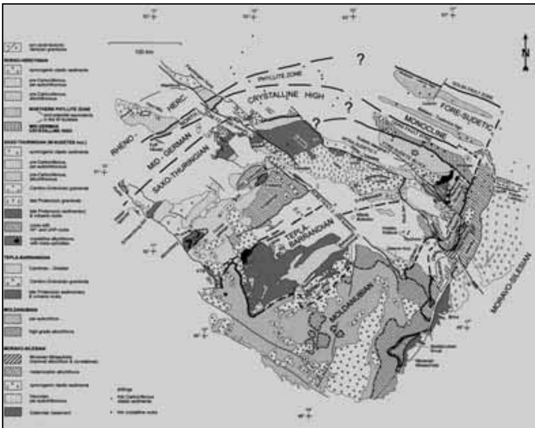
Figure 1 - Geological map of the Bohemian Massif (after Franke and Zelazniewicz, 2002)
