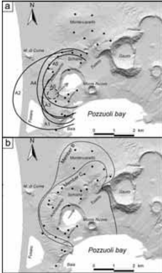
Figure 43 - Distribution of the Averno 2 Tephra. a: isopachs of the fallout deposits of Member A, arrow indicates direction of vent migration; b: pyroclastic-currents deposits of Member B and C.
