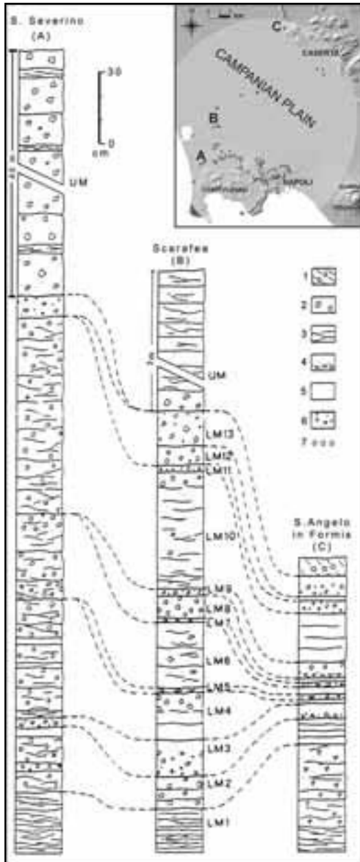
Figure 29 - Outcrop area and stratigraphic sections of the proximal (St. Severino), intermediate (Scarafesa), and distal (Sant'Angelo in Formis) facies of the Neapolitan Yellow Tuff. 1: reworked deposits; 2: pyroclastic flow deposits; 3: pyroclastic surge deposits; 4: pumice-and-ash fallout deposits; 5: ash fallout deposits; 6: debris flow; and 7: accretionary lapilli. (after Orsi et al., 1992)
