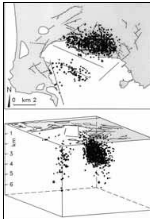
Figure 45 - Plan and 3D view from south-east of the hypocentres of earthquakes occurred in the 1982-84 unrest episode.
