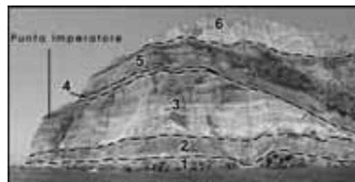
Figure 54 - Punta Imperatore promontory. 1: lava flows older than 75 ka; 2: breccia deposit at the base of the sequence aged between 75 and 55 ka; 3: pyroclastic sequence aged between 75 and 55 ka; 4: Mt. Epomeo Green Tuff sequence; 5: deposit of the Scarrupo di Panza volcano; 6: pyroclastic deposit of the 28-18 ka period of activity.
