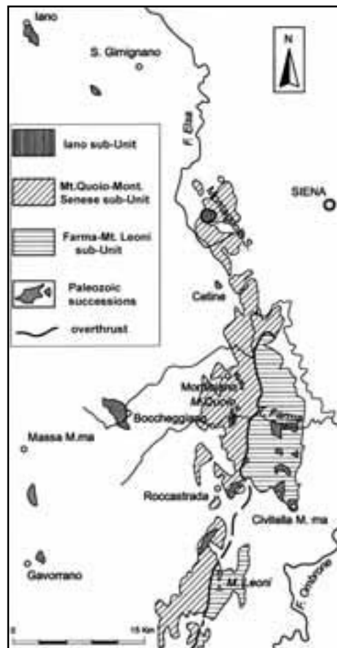
Figure 15 - Tectonic sketch map of the Iano-Monticiano-Roccastrada-Mt. Leoni structural high (Monticiano Roccastrada Unit)(redrawn from Lazzarotto et alii , 2003).
