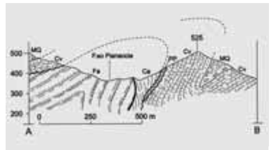
Figure 19 - Geological cross-section in Figure 18.
