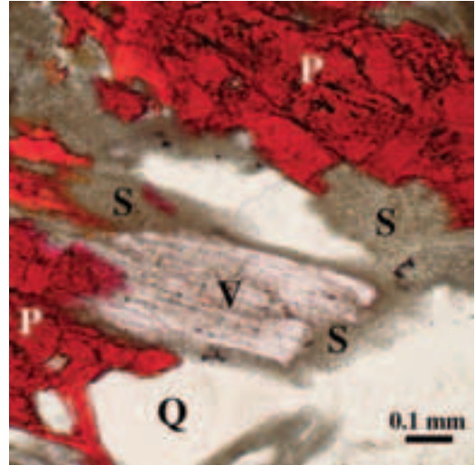
Figure 32 - Praborna; rock with piemontite (P), quartz (Q) and violan (V) partly transformed into a Cpx+albite symplectite (S) during retrogression. Plane-polarized light.
