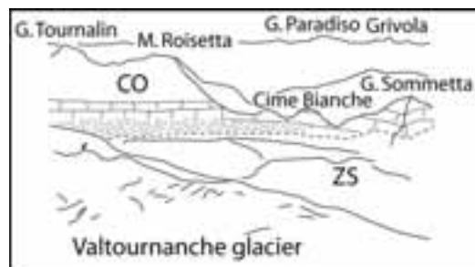
Figure 58 - Panorama from Testa Grigia towards the Sommette-Grand Tournalin ridge (SW) (from Dal Piaz, 1992, vol. 1, Fig. 7.15). CO – Combin greenschist ophiolites; ZS – Zermatt-Saas eclogitized ophiolites.
