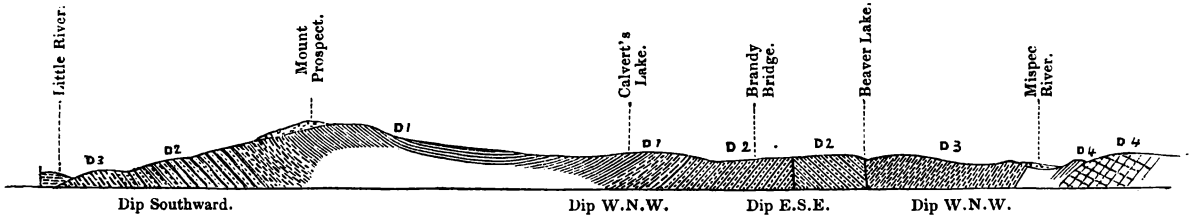
Fig. 2.—Section from the Valley of Little River to Mispec River, New Brunswick.
