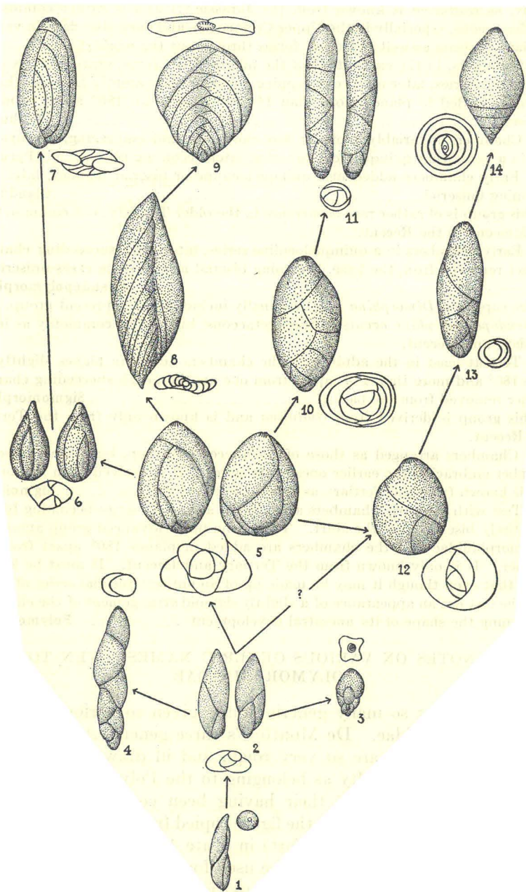
FIGURE 2.—DEVELOPMENT AND RELATIONSHIPS OF THE GENERA OF THE POLY MORPHINIDÆ. 1, 2. EOGUTTULINA. 3. QUADRULINA. 4. PALEOPOLY MORPHINA. 5. GUTTULINA. 6, 7. SIGMOIDELLA. 8. SIGMOMORPHINA. 9. POLY MORPHINA. 10, 11. PSEUDOPOLY MORPHINA. 12. GLOBULINA. 13. PYRULINA. 14. GLANDULINA
