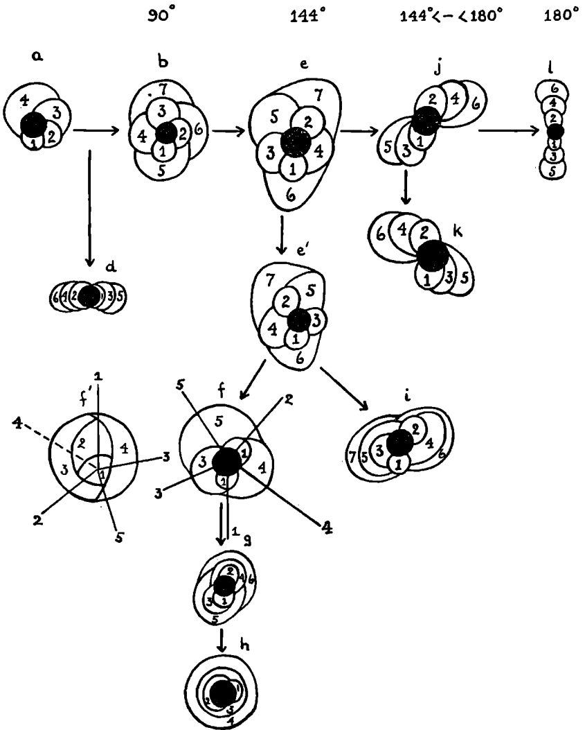
FIGURE 1.—IDEALIZED BASAL VIEWS OF VARIOUS GENERA OF THE POLYMORPHINIDAE TO SHOW THE ARRANGEMENT OF CHAMBERS. a. EOGUTTULINA (SPIRAL). b. QUADRULINA (TETRALOCULINE). d. PALEOPOLYMORPHINA (SPIRAL-BISERIAL). e, e'. GUTTULINA; e, CLOCKWISE QUINQUELOCULINE; e', CONTRACLOCKWISE QUINQUELOCULINE. f, f'. GLOBULINA; f, MICROSPHERIC FORM; f', MEGALOSPHERIC FORM. g. PYRULINA (QUINQUELOCULINE-BISERIAL). h. GLANDULINA (BISERIAL-UNISERIAL). i. PSEUDOPOLYMORPHINA (QUINQUELOCULINE-BISERIAL). j, k. SIGMOMORPHINA, SIGMOIDELLA (SIGMOIDAL); j, CLOCKWISE; k, CONTRACLOCKWISE. l. POLYMORPHINA (BISERIAL)
