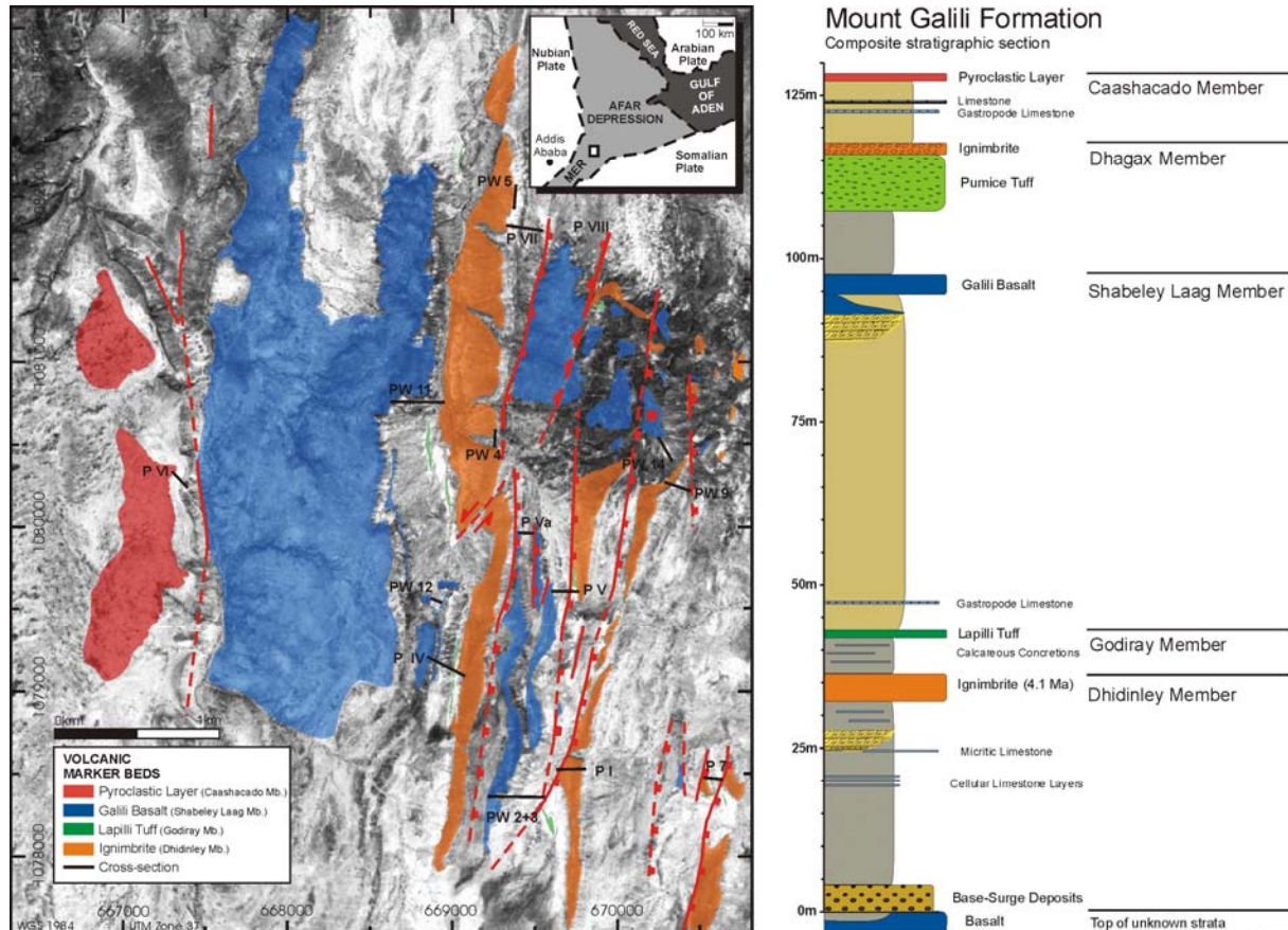
Fig.1: Geological sketch map of Galili research area and composite lithostratigraphy of the Mount Galili Formation.
