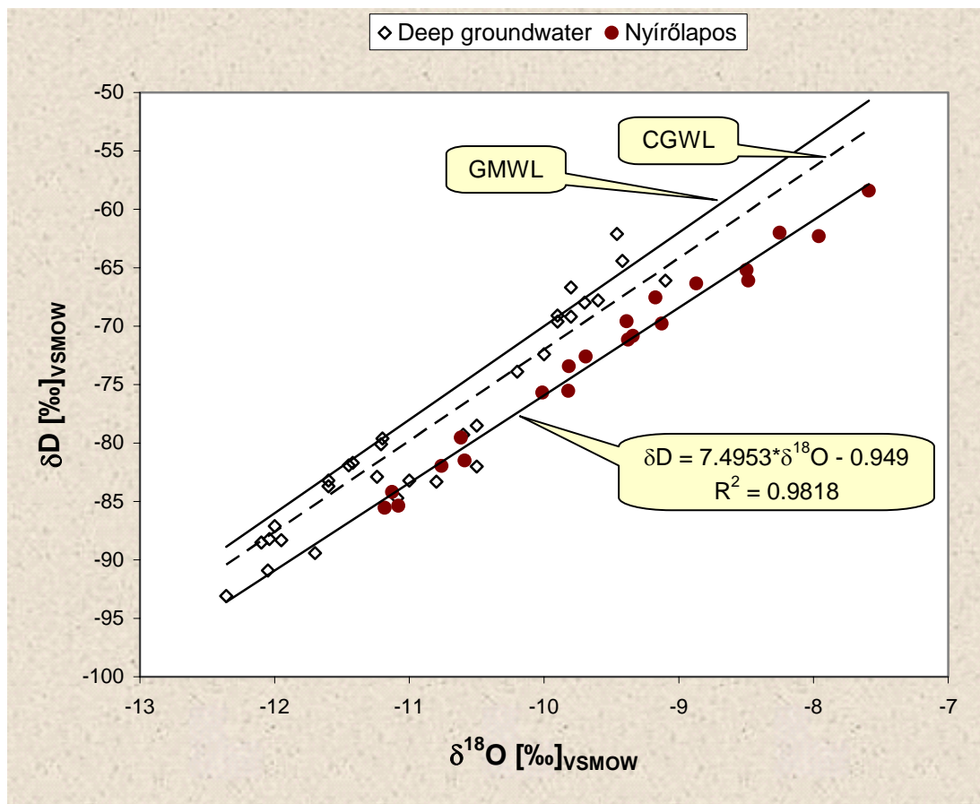
Fig. 2. The \delta D - \delta^{18}O plot of the water samples from Nyírőlapos (solid symbols), and of deep groundwaters from different part of the Great Hungarian Plain (open symbols, Stute & Deák 1989). GMWL = Global Meteoric Water Line \delta D = 8 * \delta^{18}O + 10 ; CGWL = Groundwater Line of the Carpathian Basin \delta D = 7.8 * \delta^{18}O + 6 , Deák 1995).
