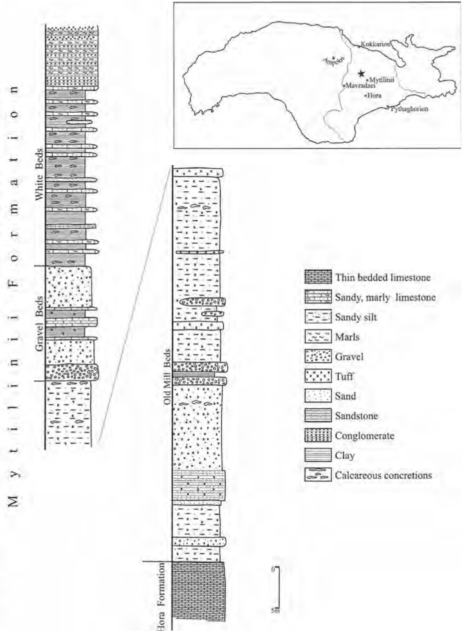
Figure 8: “Mylos” stratigraphic column of the upper Neogene deposits of the Mytilinii Basin, Samos, indicating the basal-medial part of Mytilinii Fm in contact with Hora Fm.
