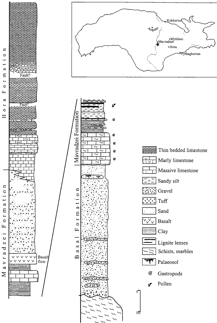
(Fig. 6). Several authors suggested that the presence of pebbles originating from the Hora Fm in the Mytilinii Fm indicates an erosional phase before the deposition of Mytilinii Fm and thus, a hiatus between these two units. However, the pebbles from the Hora Fm occur in the middle part of the Mytilinii Fm (the White Beds member of WEIDMANN et al., 1984) interrupting its lithological continuum. Hence, the erosional phase cannot be correlated to the boundary between Hora Fm and Mytilinii Fm, which is dated to 8.6 My (KOSTOPOULOS et al., 2003). It is quite possible that during the deposition of Mytilinii Fm, at ~7.5 My (which is more or less the age of the White Beds; see KOSTOPOULOS et al., 2003; KOUFOS et al., this volume)
