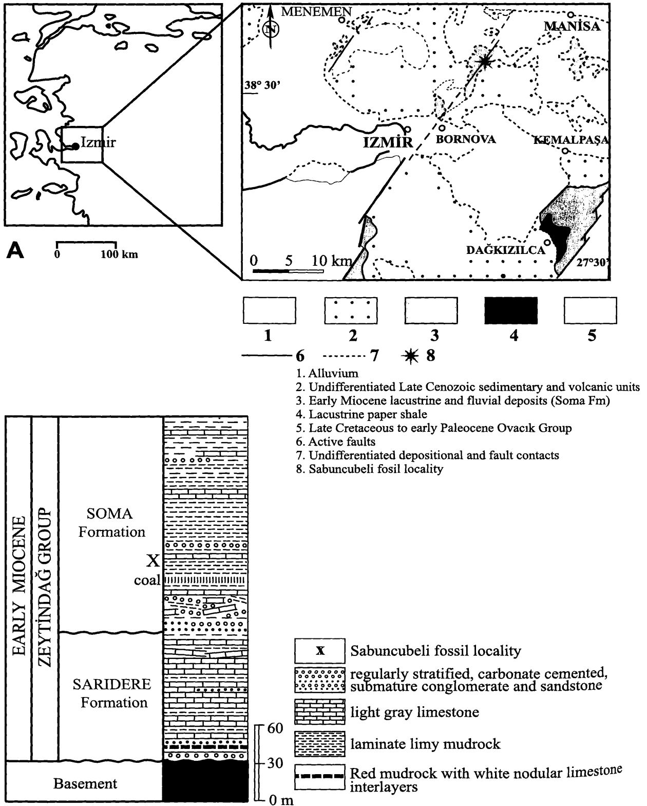
Fig. 1: A. Location and geological map (enlarged) of the study area. The locality Sabuncubeli is indicated by an asterisk. B. Schematic lithological succession of the continental Early Miocene in the study area. Figs. A and B are modified after KAYA et al. (in press).
