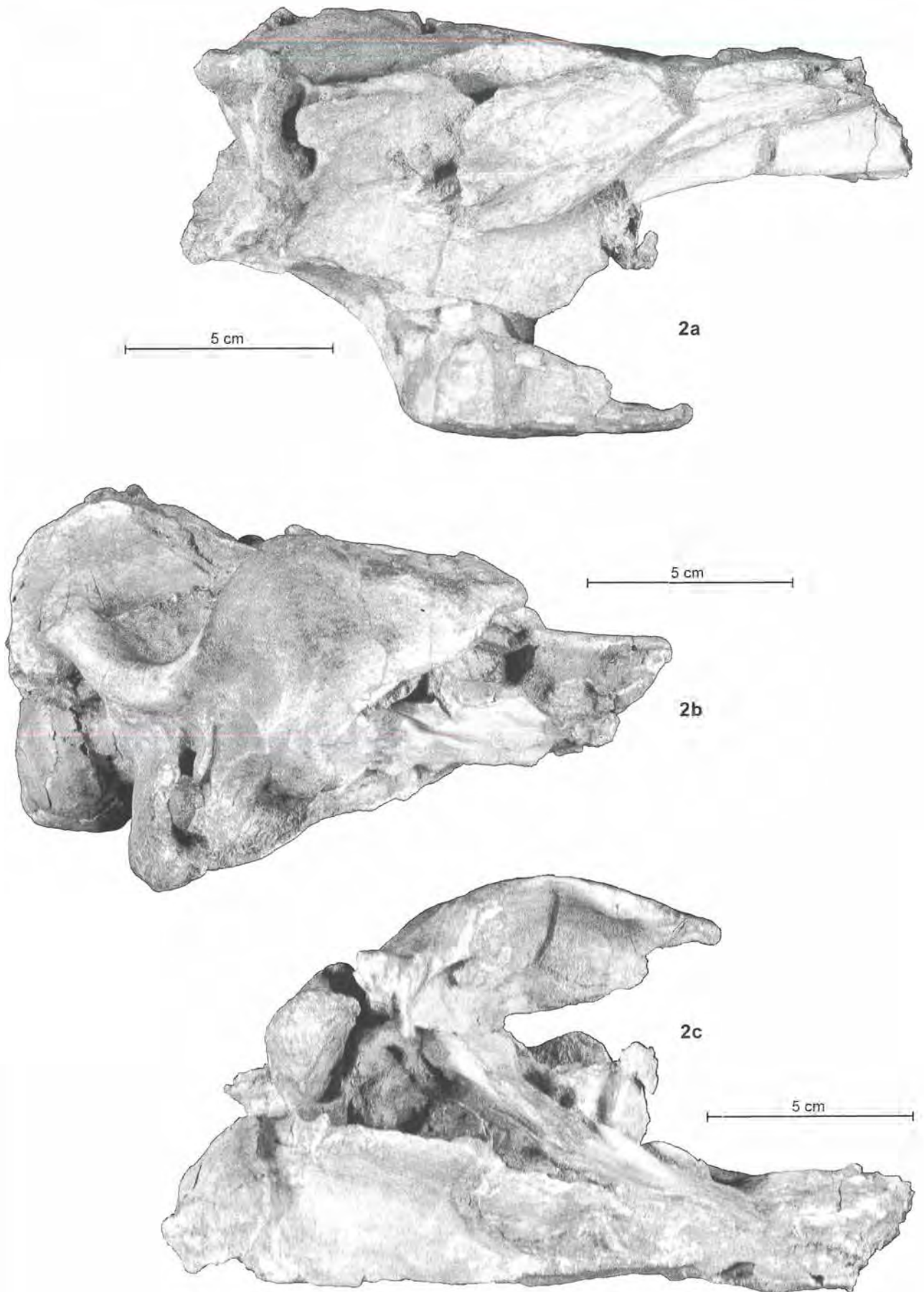
Fig. 2: Prepotatodelphis korneuburgensis , new genus and species, enlarged views of the braincase of the holotype, NHMW 2002z0001/0000; 2a: dorsal view; 2b: right lateral view; 2c: ventral view.
