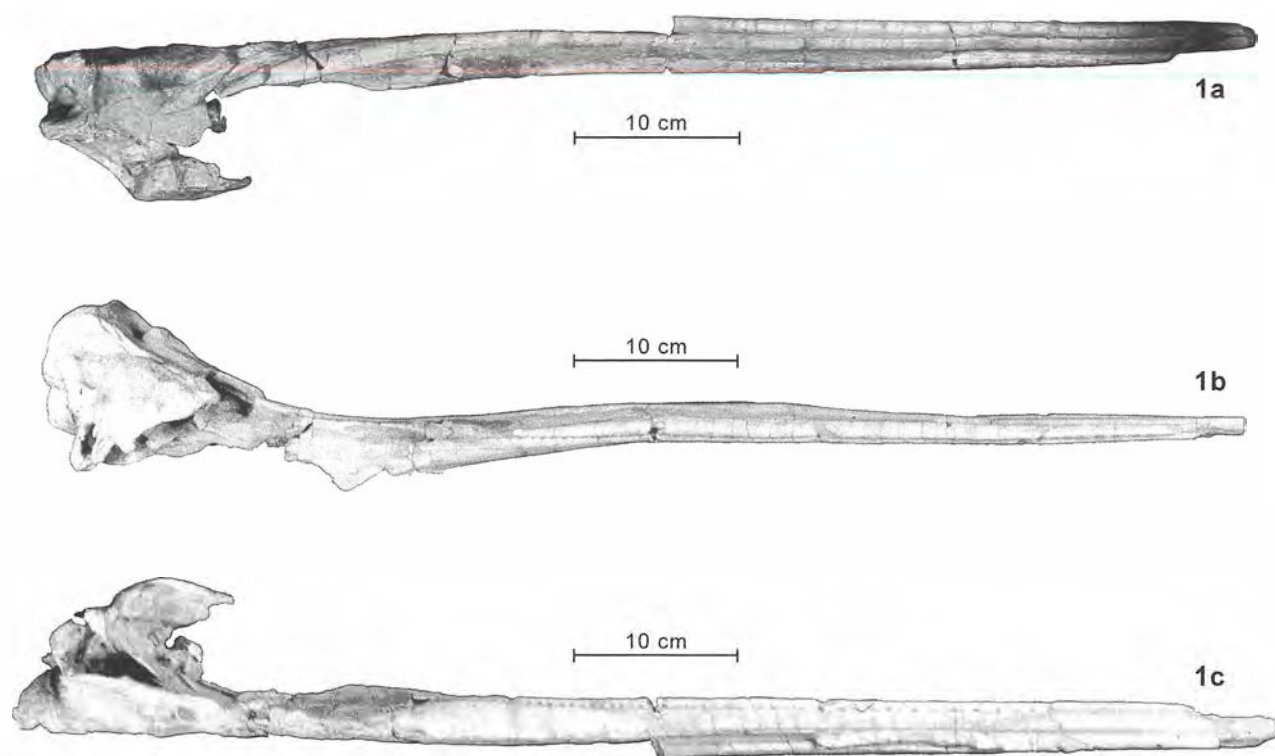
Fig. 1: Prepotatodelphis korneburgensis , new genus and species, holotype skull, NHMW 2002z0001/0000; 1a: dorsal view; 1b: right lateral view; 1c: ventral view.
