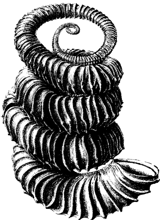
Figure 1. Restoration of Didymoceras binodosum (KENNEDY and COBBAN, 1993). Drawing by John R. STACY is based on specimens from the Pierre Shale of South Dakota and is approximately natural size. Figure supplied by Dr. W.A. COBBAN (Denver).
