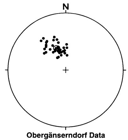
Fig. 2: Characteristic remanence directions of samples from the Obergänsersdorf sandpit. No tilt correction because of horizontal bedding. Equal area projection with full symbols for lower hemisphere. Square represents mean value with \alpha_{95} confidence circle.
