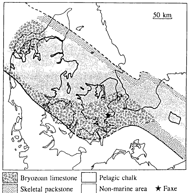
Figure 1: Simplified palaeogeography and facies distribution in the Danish area in late Middle Danian time; asterisk indicating the location of Faxe Quarry (in part based on HÅKANSSON & THOMSEN (1974) and THOMSEN (1989)).
