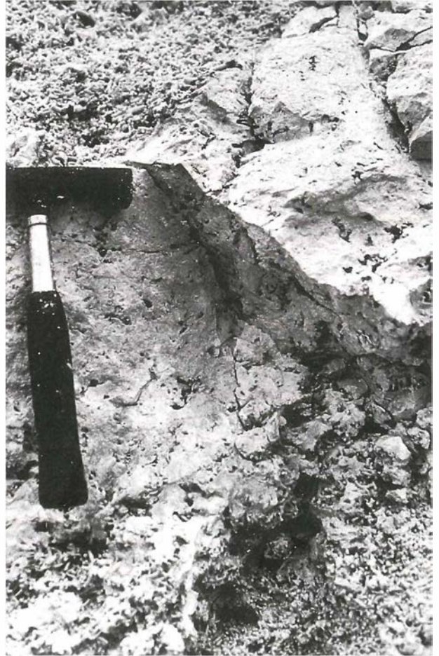
Figure 4: A single depositional unit of mound phase A, steeply inclined towards the left. At the hammerhead the sharp upper surface of the upper matrix-rich part is in direct contact with the matrix-poor lower part of the next depositional unit, which is constituted by virtually matrix-free coral sticks. The highly irregular and gradual change from matrix-rich to matrix-poor coral limestone is characteristic of this mound phase. Length of hammer is 30 cm
