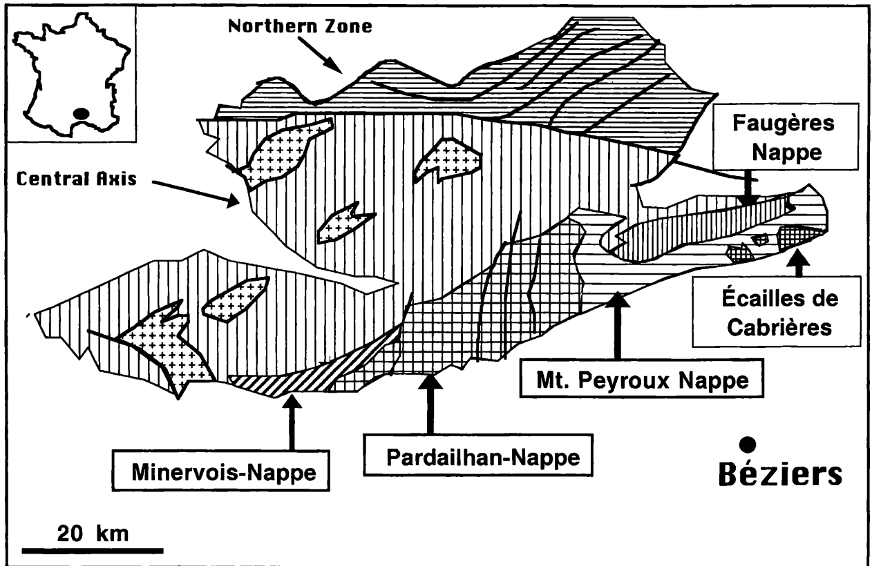
Figure 1: Main structural units of the Montagne Noire. Arrows on labels "Mt. Peyroux Nappe" and "Minervoïis Nappe" point to working areas (from FLAJS & HÜSSNER, 1993).
