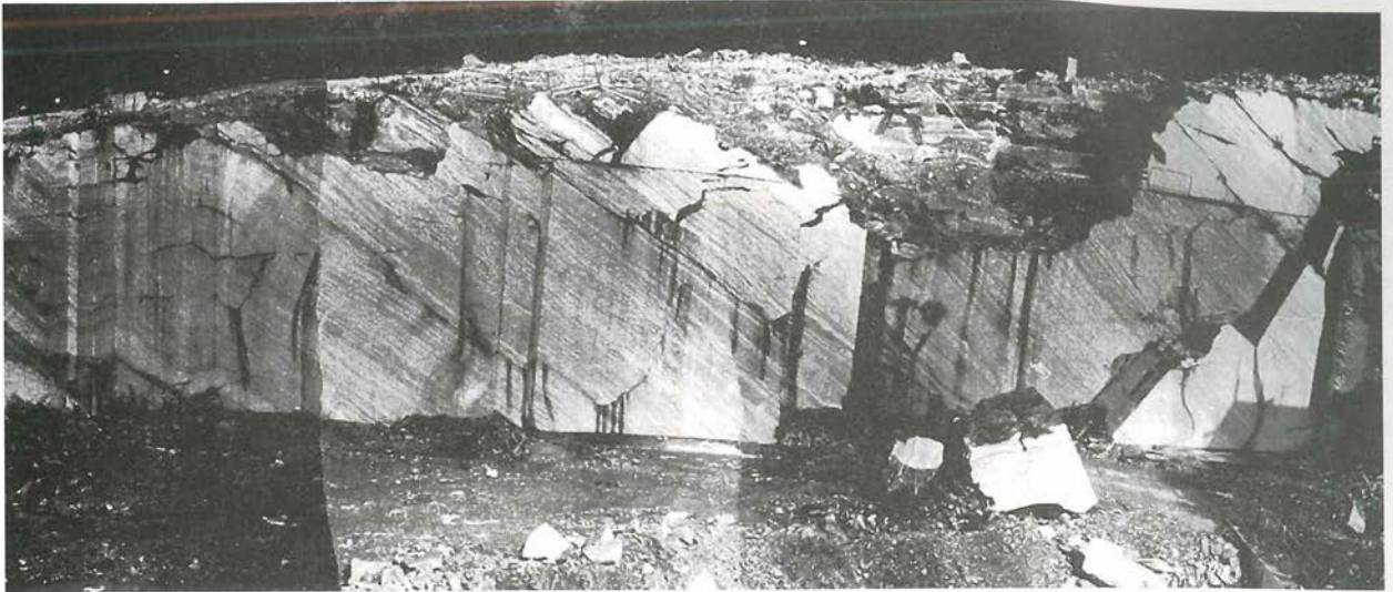
Figure 2: Northern wall of the Rocamat Quarry NE of the village of Caunes/Minervois. Photograph taken in spring 1992. Note alternations of red biomicrite and white stromatactis structures. Stromatactis layers are arranged in bundles. Length of quarry wall is approx. 50 m.
