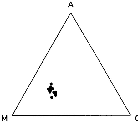
Fig. 47. Triangular diagrams of aragonite (A) – Mg-calcite (M) – calcite (C) of the mud fraction related to bottom facies.
