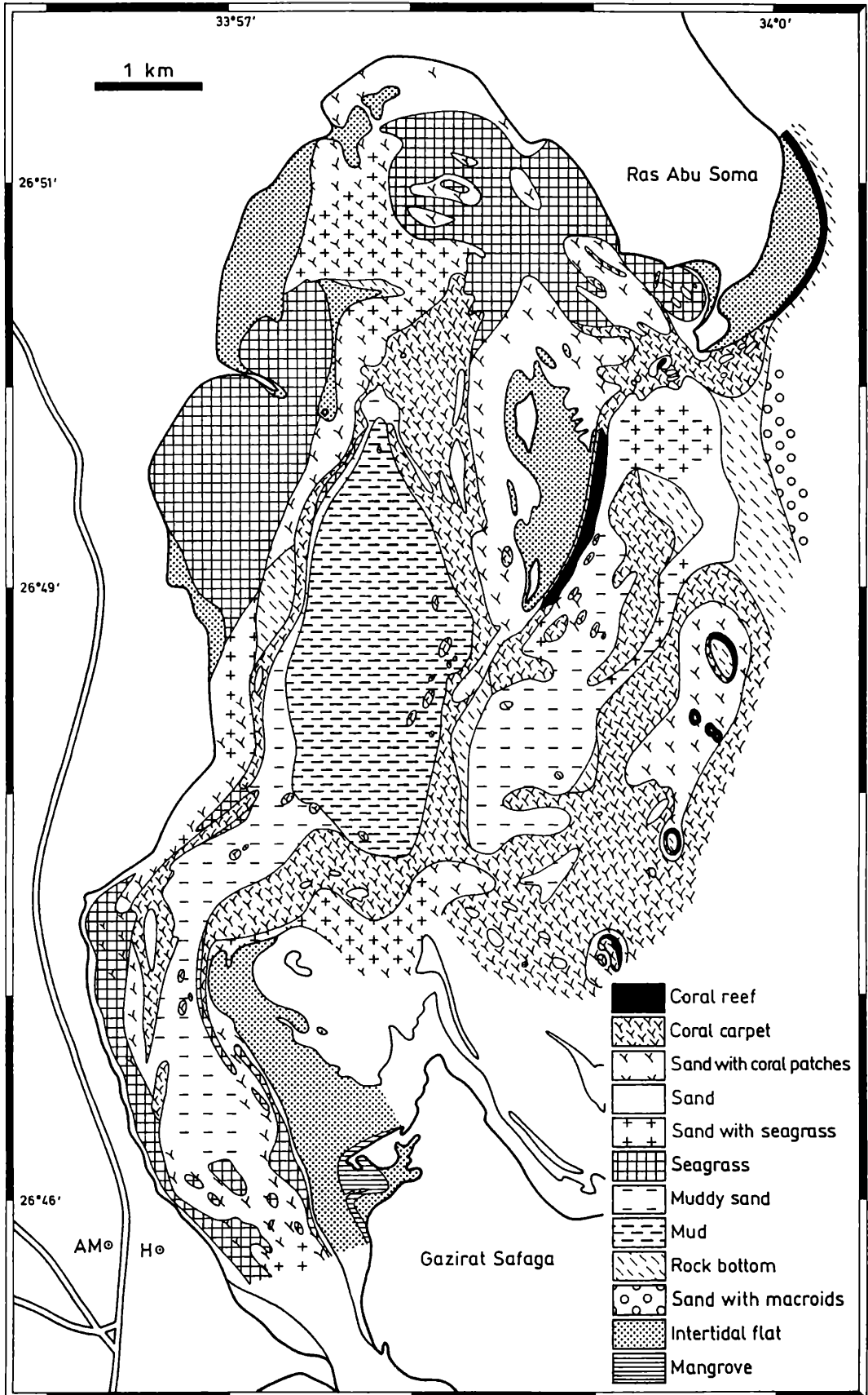
Fig. 54. Distribution of bottom facies (according to PILLER & PERVESLER, 1989).
