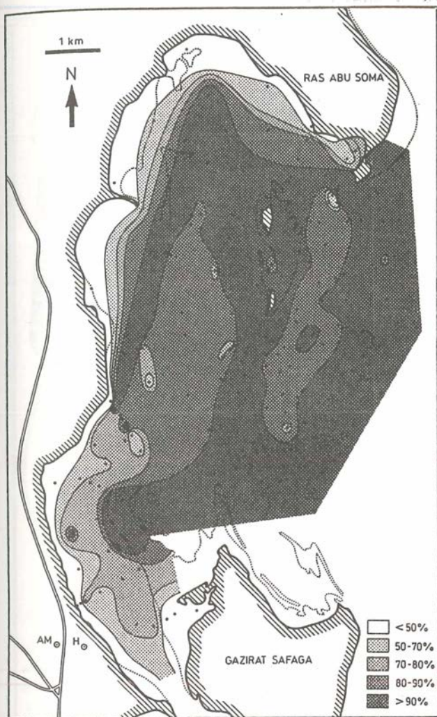
Fig. 31. Distribution of carbonate in the total samples.
