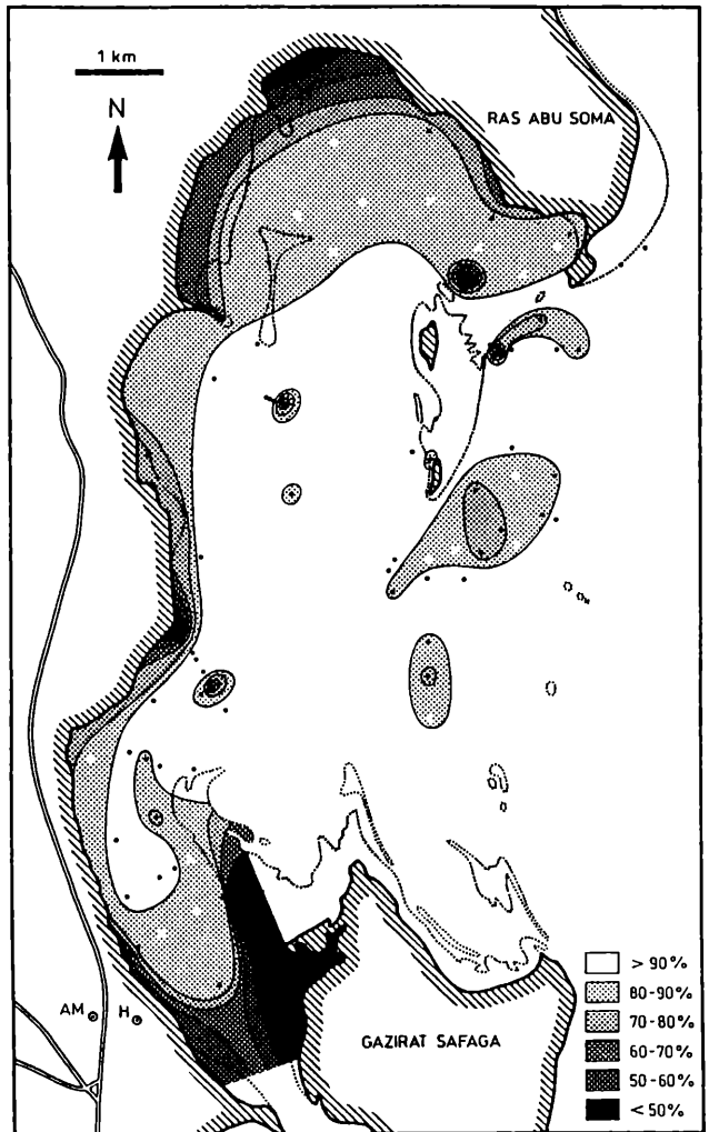
Fig. 17. Frequency distribution of skeletal components ( > 250 \mu\text{m} ).
