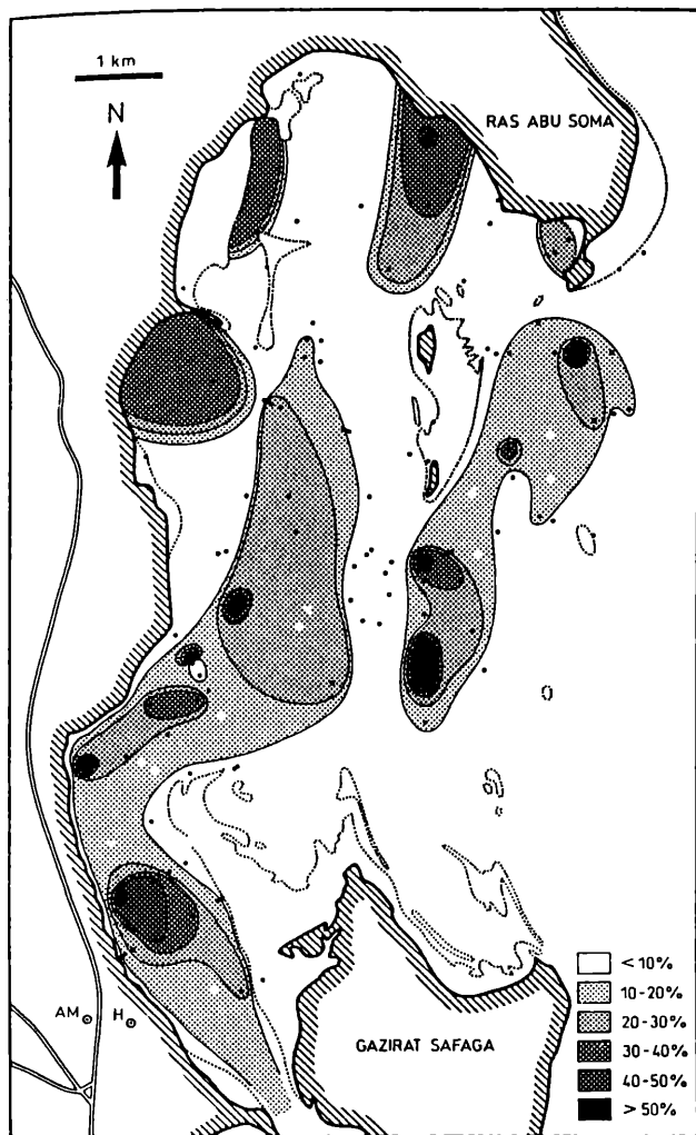
Fig. 18. Frequency distribution of foraminifers (> 250 \mu\text{m} ).
