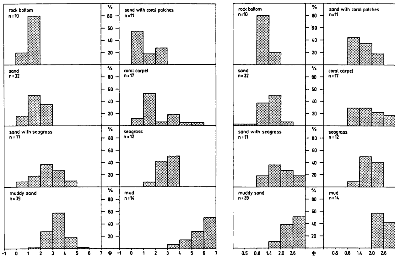
Fig. 12. Distribution of mean grain size ( M_Z ) related to bottom facies. Fig. 13. Distribution of sorting (2nd moment) related to bottom facies.
