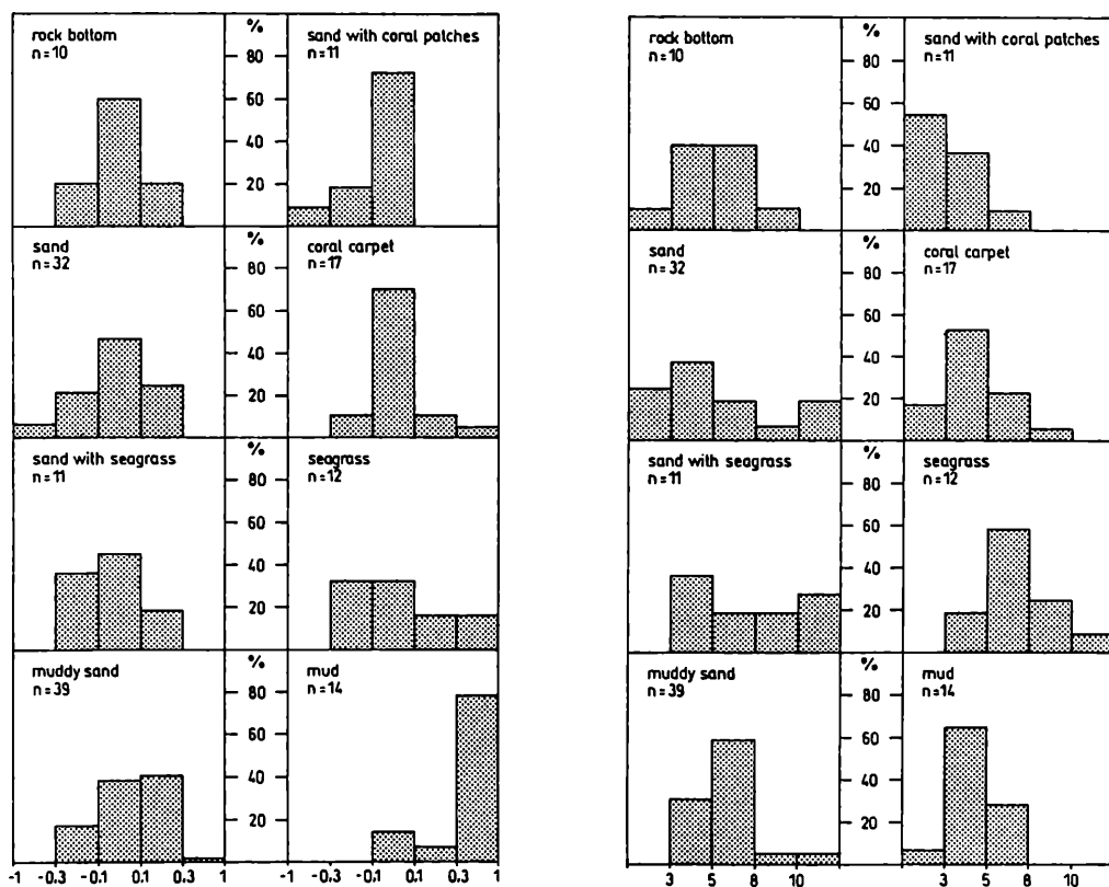
Fig. 14. Distribution of skewness ( SK_I ) related to bottom facies. Fig. 15. Distribution of kurtosis (4th moment) related to bottom facies.
