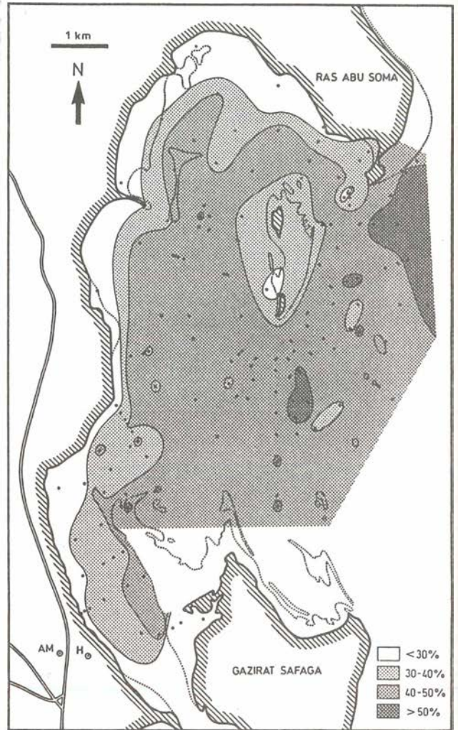
Fig. 34. Distribution of Mg-calcite in the total samples (related to the total mineral content).
