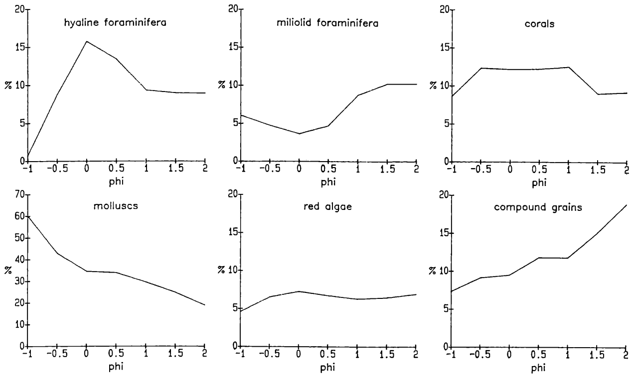
Fig. 28. Distributions of the 6 most abundant component categories in grain size fractions.
