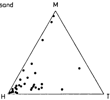
Fig. 30. Triangular diagrams of hyaline - miliolid - agglutinated foraminifers related to bottom facies.
