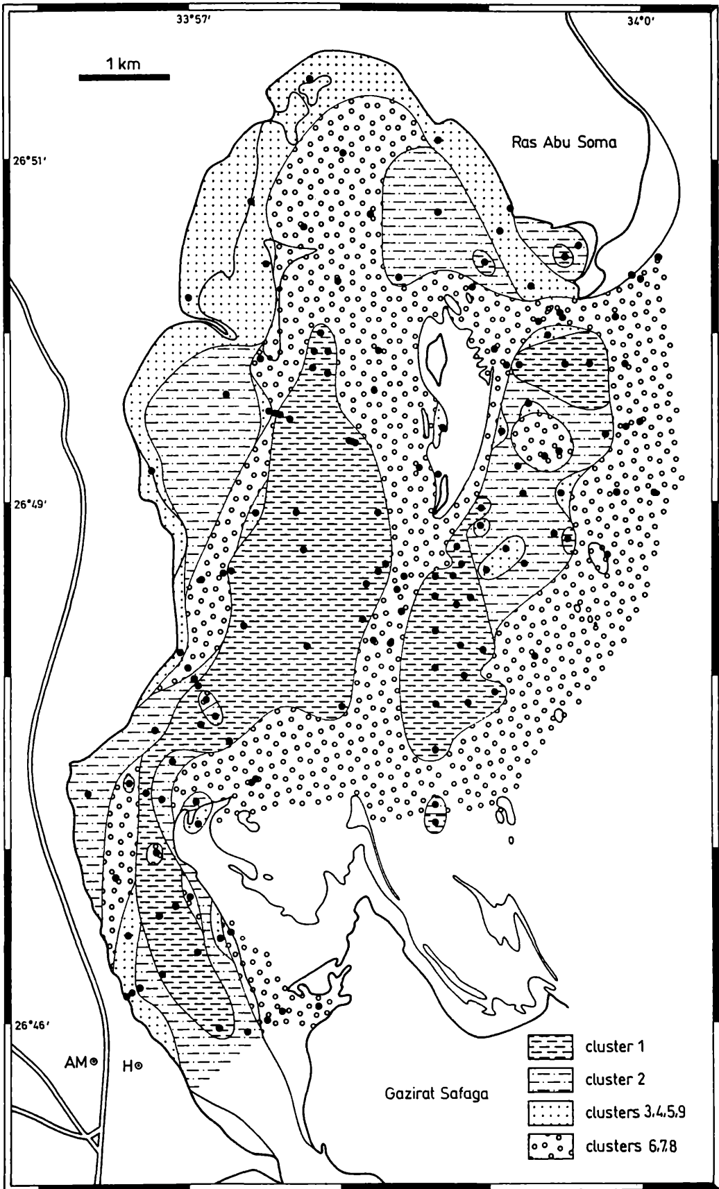
Fig. 8. Distribution of the clusters at a correlation coefficient of 0.85 of the cluster analysis of grain size data.
