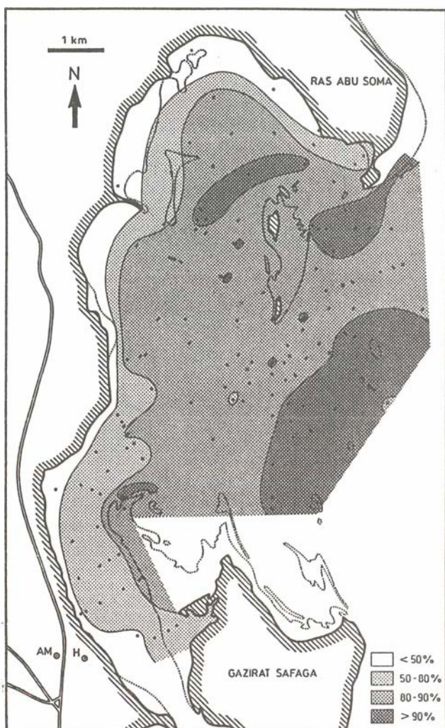
Fig. 32. Distribution of carbonate in the mud fraction.
