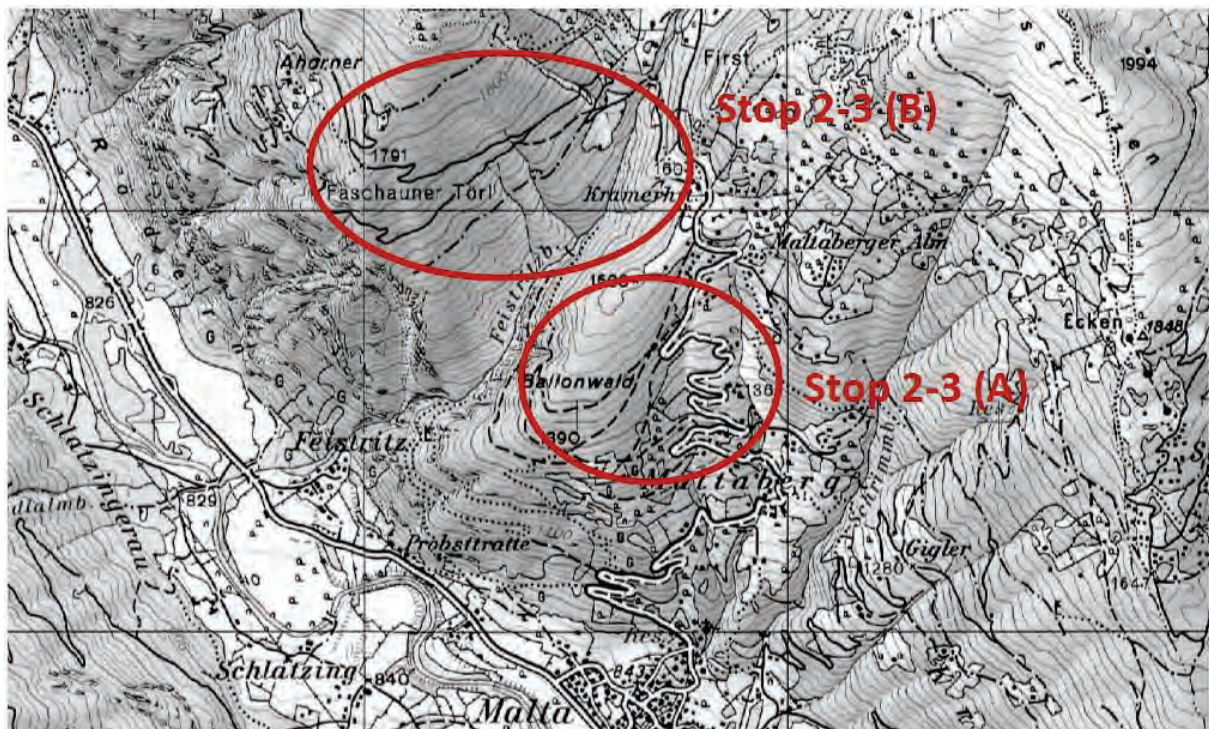
Figure 23: Location of Stops 3 (A) and 3 (B)
