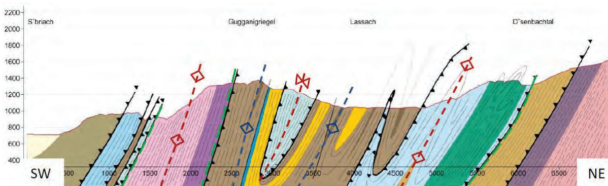
Figure 16: Profile 1 (trace and legend in Figure 26) near the Kaponig Valley: D5 folds marked in red, axial traces of D3 in blue, D4 roof thrust of the Venediger Duplex in green dashed lines.
