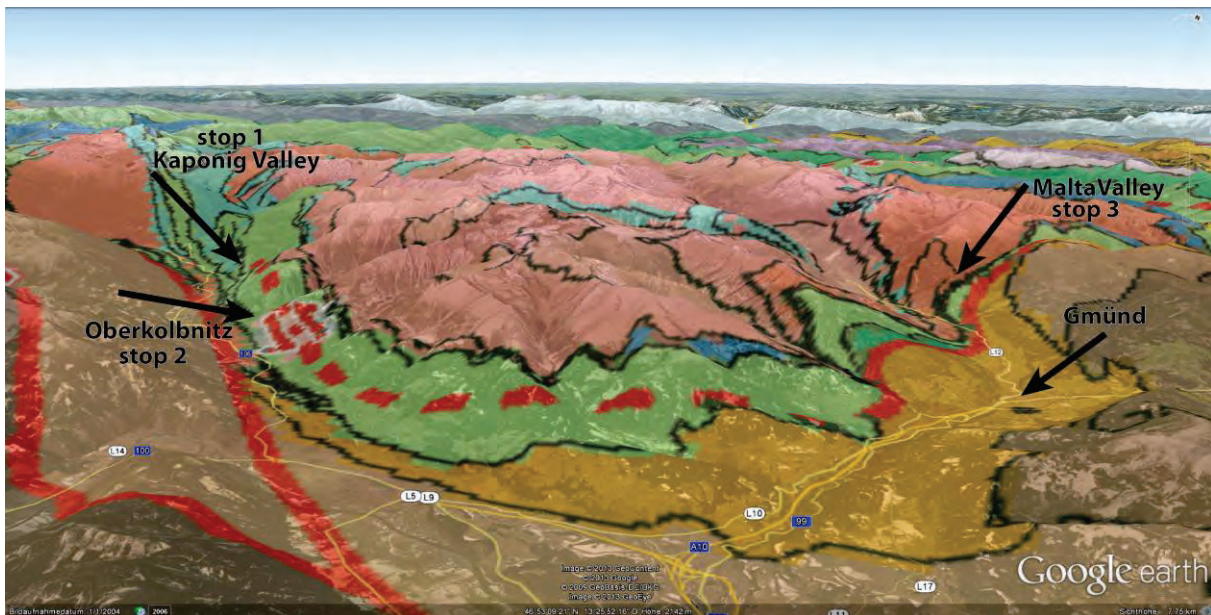
Figure 10: Google Earth image with superposed tectonic map of the southeastern end of the Tauern Window as viewed to the NNW. Black arrows indicate the stops described below and show the town of Gmünd, where we will spend a night. Symbols as in the tectonic map of the Tauern Window (Fig. 11, 27).
