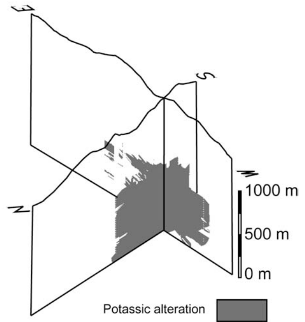
Fig. 5. Spatial distribution of potassic alteration at Red Mountain.
