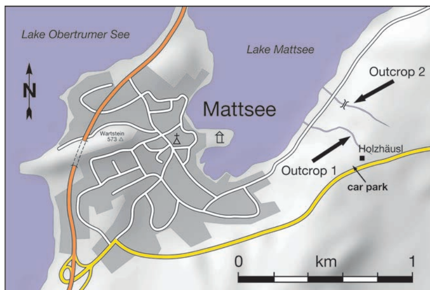
Figure A2.2 ▲ Locations of outcrops near Holzhäusl
