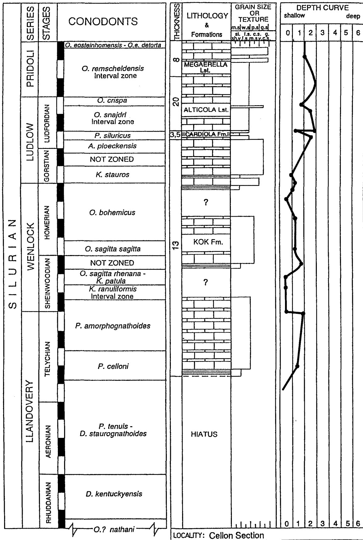
Fig. 3. Conodont stratigraphy, lithology, grain size and depth curve of the Silurian portion of the Cellon section (CI - condensed interval, EHST - early highstand system tract, LHST - late highstand (regressive) system tract, RST - regressive system tract, TST - transgressive system tract, SB - sequence boundary).
