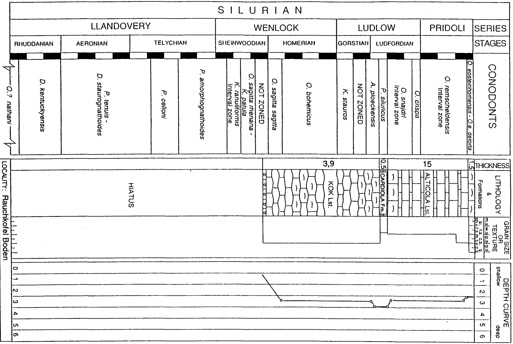
Fig. 6. The Silurian part of the Rauchkofel Boden section with indication of conodont stratigraphy, lithology, grain size and depth curve.
