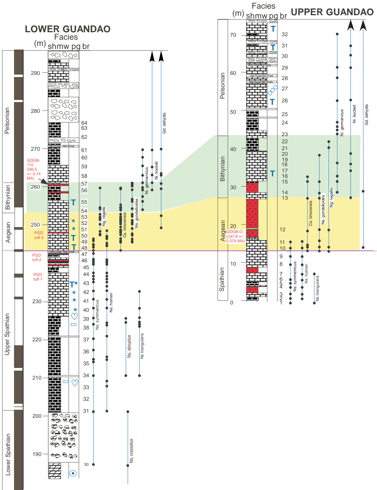
Figure 17: Olenekian-Anisian boundary section in basin margin facies in Lower Guandao and Upper Guandao sections (see figures 9 and 10 for locations). Lithology and grain type symbols are the same as those shown in figures 13 and 14. Magnetic reversal stratigraphy (black is normal polarity) is shown at left of Lower Guandao section. Conodont biostratigraphy and preliminary U-Pb age dates of volcanic ash layers are shown for both sections. We emphasize that the U-Pb age dates are still preliminary and should not be cited as certain boundary ages until the data is sufficiently refined. Further discussion of the biostratigraphy, geochronology, and magnetostratigraphy is provided in the stop descriptions of the field guide in this volume.
