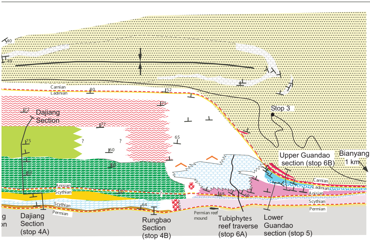
Figure 9: Geological map of the eastern limb of the Bianyang syncline (from Lehmann, 1993). Location of map area is the eastern limb of the syncline shown in figure 8. Stops for the field excursion and stratigraphic sections discussed in the text are shown.
