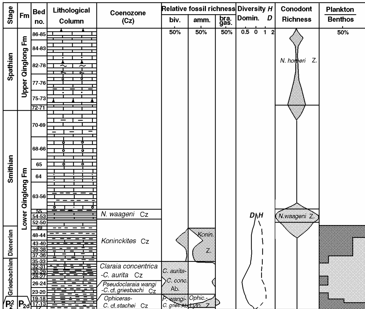
Figure 9. Lower Triassic stratigraphical sequence of the Hushan Section
