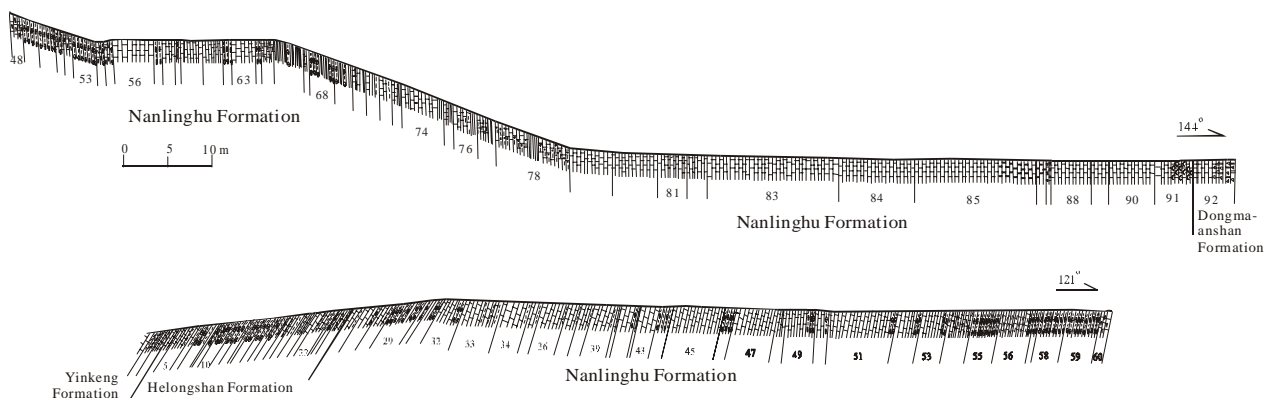
Figure 9. Lower Triassic profile of the South Majiashan Section
