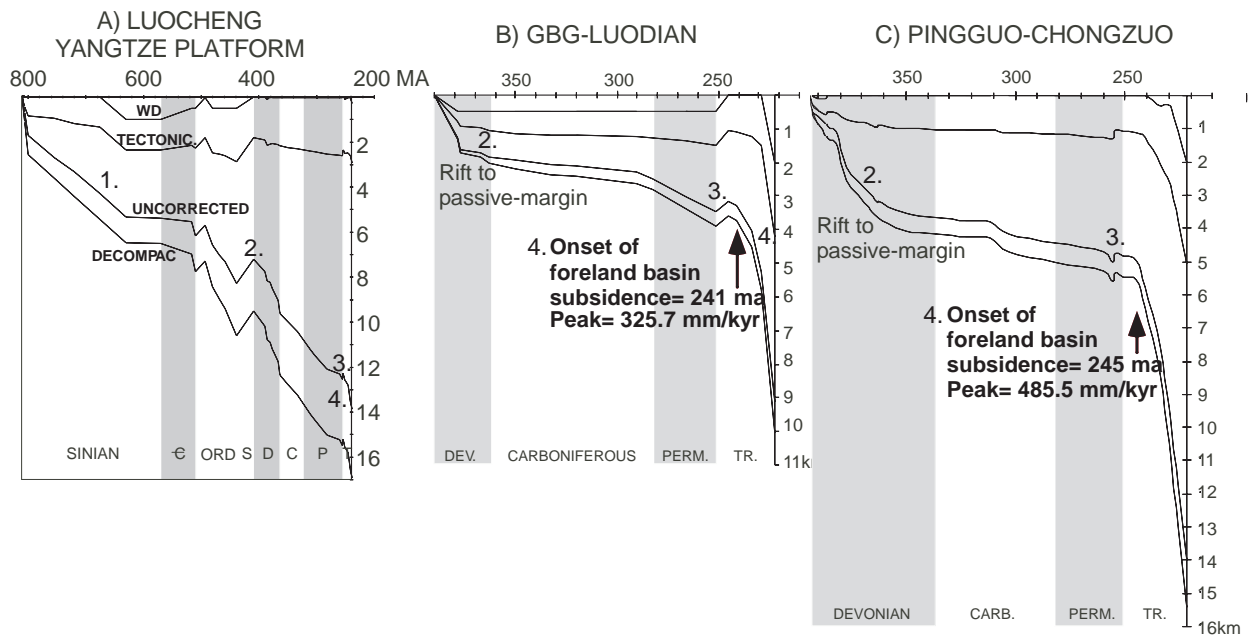
Figure 6: Subsidence histories. Subsidence curves were compiled from unpublished composite stratigraphic sections, biostratigraphy, lithofacies and interpreted water depths provided by the Guizhou Bureau of Geology and Geological Survey of Guangxi. Subsidence analyses (backstripping) were performed with a program provided by M. A. Kominz using the decompaction and tectonic subsidence algorithms of Bond and Kominz (1984). A) Proterozoic through Triassic subsidence history from Loucheng of central Guangxi. B) Devonian through Triassic subsidence history from GBG-Luodian area southern Guizhou. C) Devonian through Triassic subsidence history from Chongzuo-Pingguo platform, southern Guangxi. Tectonic events indicated numerically: 1 - Late Proterozoic to Early Paleozoic stabilization of Yangtze craton and passive-margin development. 2 -Guangxi orogeny, Devonian rifting of south China block from Gondwana. 3 - “Dongwu movement” Late Permian extension associated with Emeishan volcanism. 4. Indosinian orogeny, Triassic foreland basin development and accelerating subsidence. See text for discussion of tectonic history.
