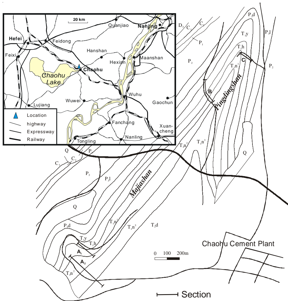
Figure 2. Location map of Chaohu and geological map of Mt. Pingdingshan-Mt. Majiashan D 3 -Upper Devonian, C 1 -Lower Carboniferous, C 2 -Upper Carboniferous, P 1 -Lower Permian, P 2 -Middle Permian, P 3l -Upper Permian Longtan Formation, P 3d -Upper Permian Dalong Formation, T y -Lower Triassic Yinkeng Formation, T h -Lower Triassic Helongshan Formation, T n1 , T n2 , T n3 -Lower, Middle, Upper Member of Lower Triassic Nanlinghu Formation, T 2d -Middle Triassic Dongmaanshan Formation, Q-Quaternary; A 1 +A 2 -South Majiashan Section, B-West Pingdingshan Section, C-North Pingdingshan Section
