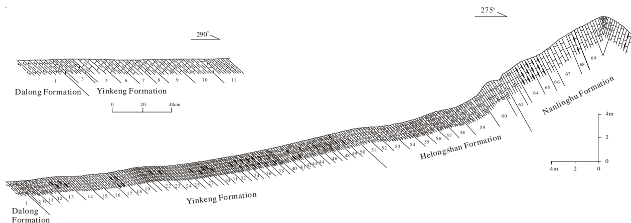
Figure 4. Lower Triassic profile of the North Pingdingshan Section
