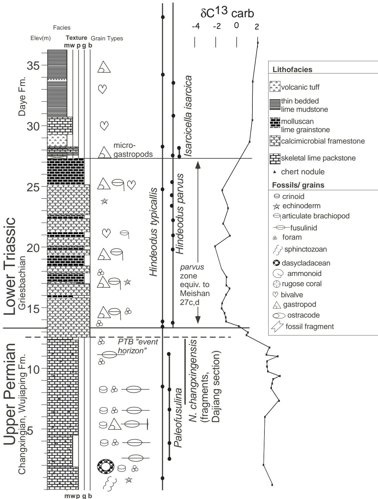
Figure 11: Permian-Triassic boundary section at Heping (1 km south of Daijiang) with biostratigraphic and carbon isotope data. The PTB event horizon is marked by the last occurrence of diverse Permian fossils at the top of skeletal packstone of the Wujiaping Formation. The biostratigraphic Permian-Triassic boundary is defined by the first appearance of Hindeodus parvus slightly higher, in the lower part of the calcimicrobial framestone. See figures 9 and 10 for location.
