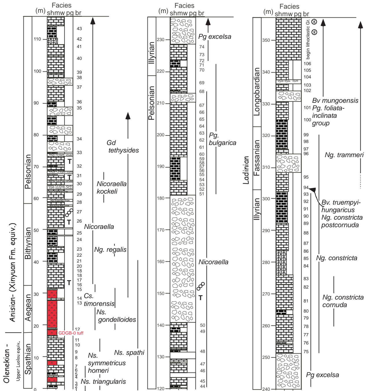
Figure 14: Lower Triassic (Spathian) through Middle Triassic (Ladinian) strata at upper Guandao section. Facies are from the basin-margin slope succession on the northern margin of the GBG. See figures 9 and 10 for location. Lithology and grain type symbols are the same as those shown in figures 13. Conodont biostratigraphy and volcanic ash horizons are indicated. U-Pb dates of volcanic ash layers are shown in fig. 17.
