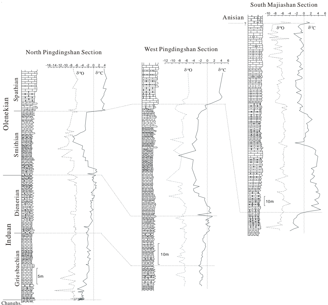
Figure 10. Lower Triassic carbon and oxygen isotopes in Chaohu and the correlation
