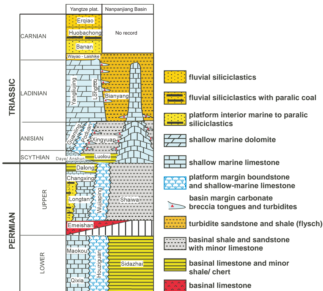
Figure 7: Schematic stratigraphic column illustrating the Permian and Triassic Formations of the Yangtze platform and GBG in southern Guizhou.
