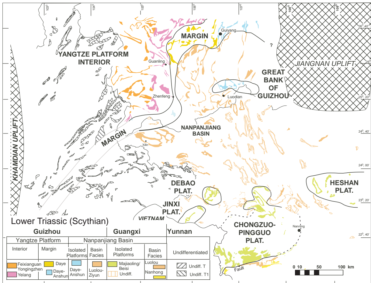
Figure 3: Lower Triassic (Scythian) lithofacies and interpreted paleogeography of the Nanpanjiang basin and Yangtze platform in Guizhou, Guangxi, and Yunnan. Compilation data and methods are given in caption for figure 2.
