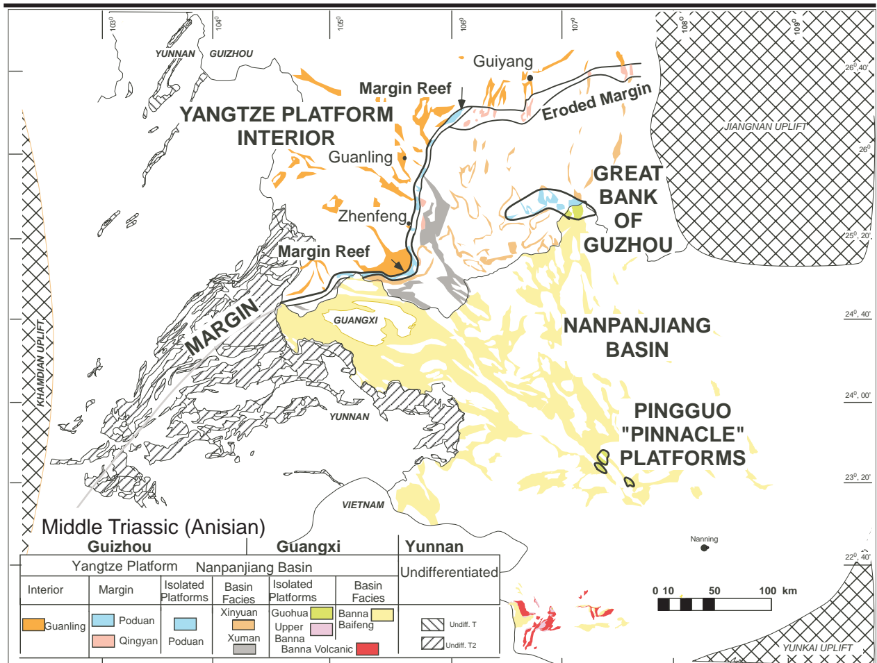
Figure 4: Middle Triassic (Anisian) lithofacies and interpreted paleogeography of the Nanpanjiang basin and Yangtze platform in Guizhou, Guangxi, and Yunnan. Compilation data and methods are given in caption for figure 2.
