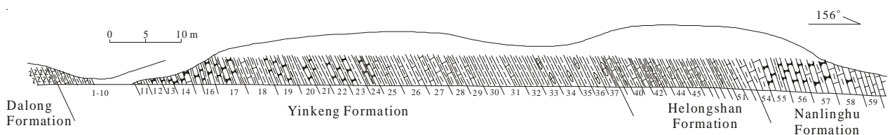
Figure 6. Lower Triassic profile of the West Pingdingshan Section
