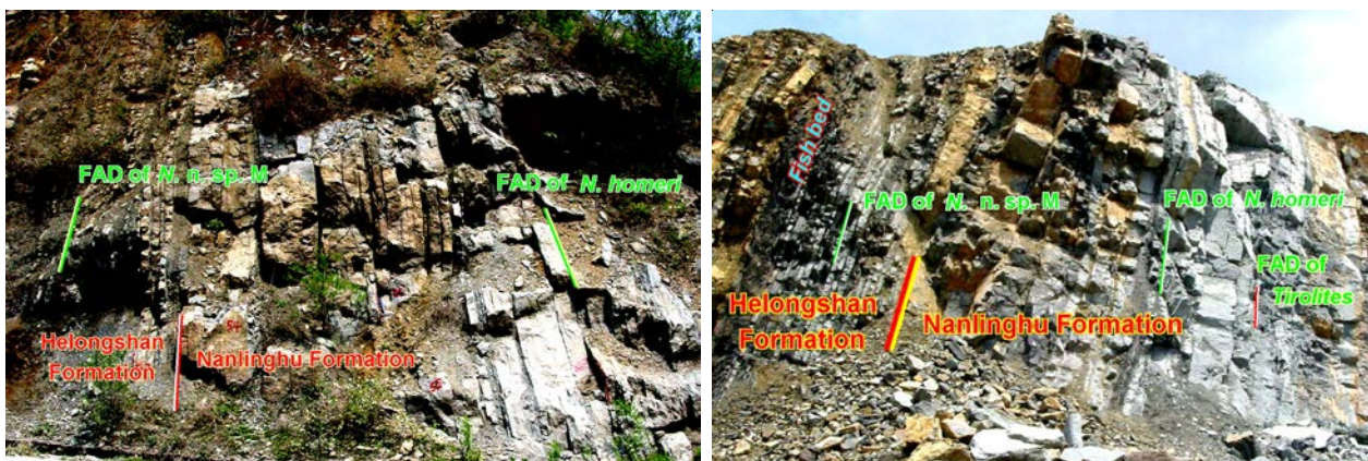
Figure 8. Smithian-Spathian boundary at the West Pingdingshan Section (a) and South Majiashan Section (b)
