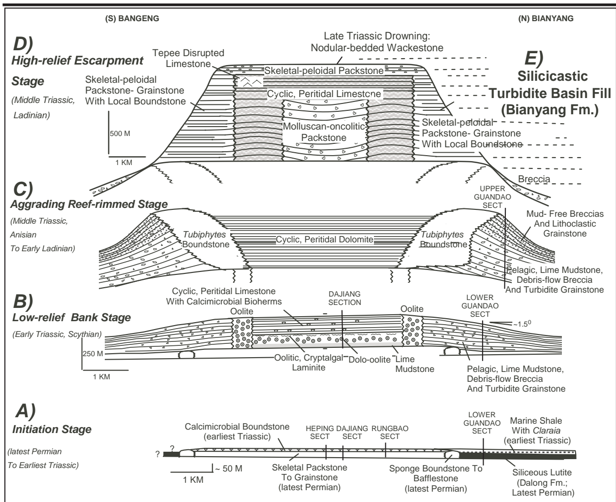
Figure 10: Restored cross-sections of the GBG illustrating Late Permian through Late Triassic evolution. Sections are from the Bianyang syncline and correspond to field trip localities (see figure 9). A) Upper Permian to basal Triassic: Initiation stage, B) Lower Triassic: Low-relief bank stage, C) Middle Triassic Anisian-Early Ladinian: Aggrading reef-rimmed stage, D) Ladinian: High-relief escarpment stage, E) Late Triassic Carnian: Termination (drowning). Fossil abundance decreases and remains low ( \ll 1\% ) through several tens of meters of lime mudstone (fig. 11).
