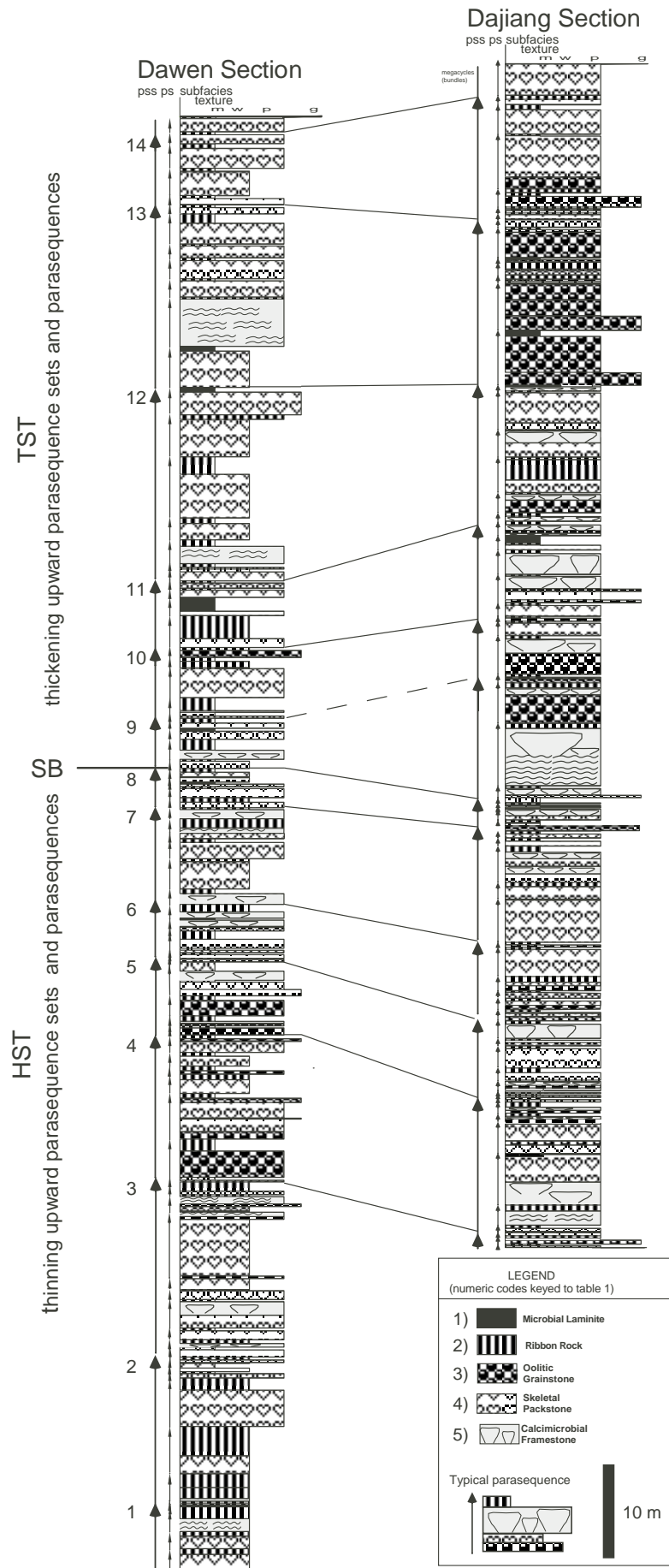
Figure 12: Lower Triassic peritidal cyclic limestone in Dawen and Dajiang sections. The locations of the sections are keyed to figures 9 and 10. Numbered arrows to the left of sections indicate 4th order parasequence sets. Unnumbered arrows immediately left of the columns denote 5th order parasequences. Systems tracts and 3rd order sequence boundary are indicated to the left of Dawen section. TST = transgressive systems tract, HST = highstand systems tract, SB = sequence boundary. The typical or most common parasequence type ("ideal cycle") is indicated on the lower right.
