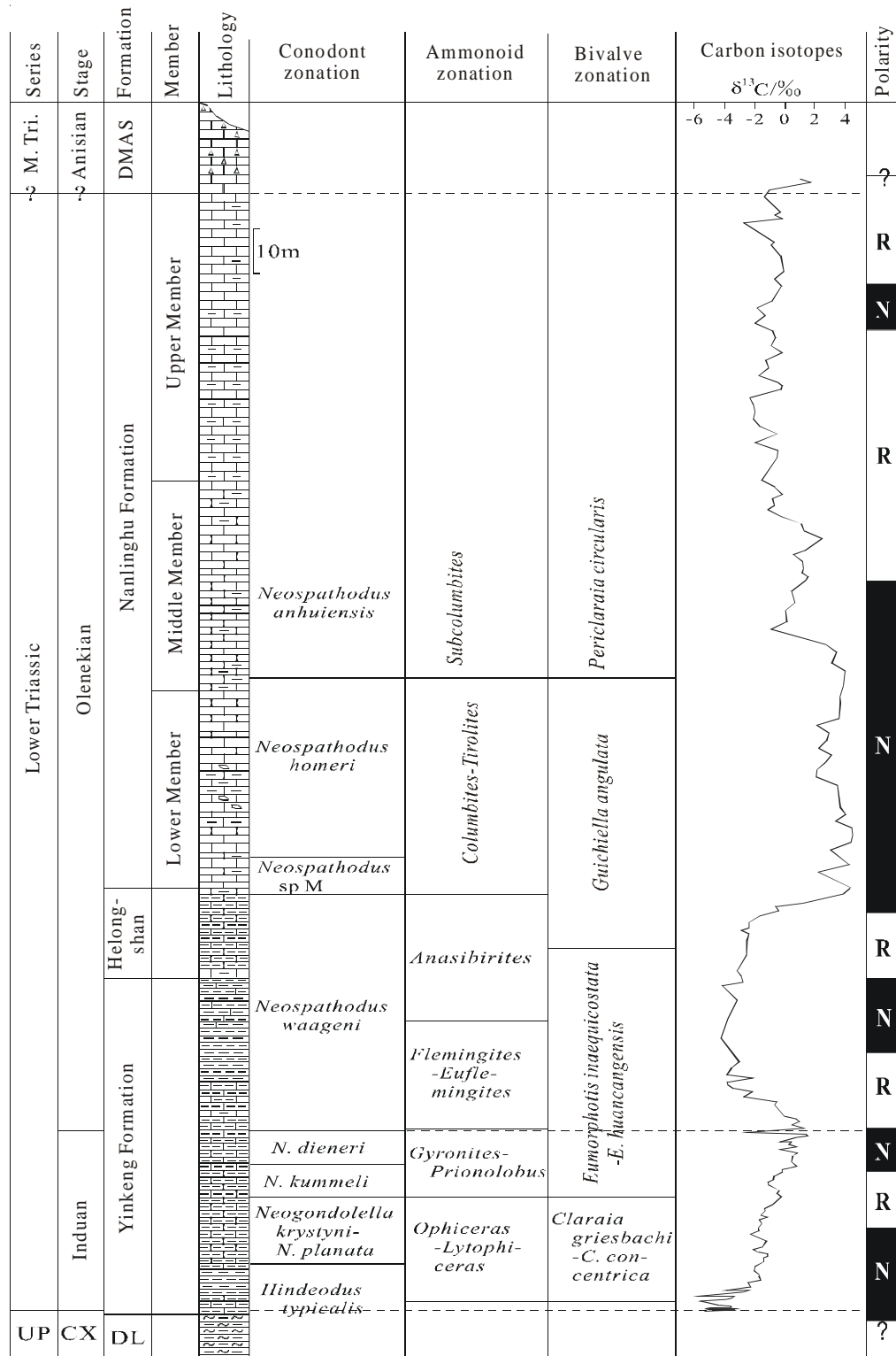
Figure 3. Integrated Lower Triassic sequence of Chaohu, Anhui Province (From Tong et al., 2005b) UP-Upper Permian, CX-Changhsingian, DL-Dalong Formation, DMAS-Dongmaanshan Formation; N-normal polarity zone, R-reversal polarity zone
