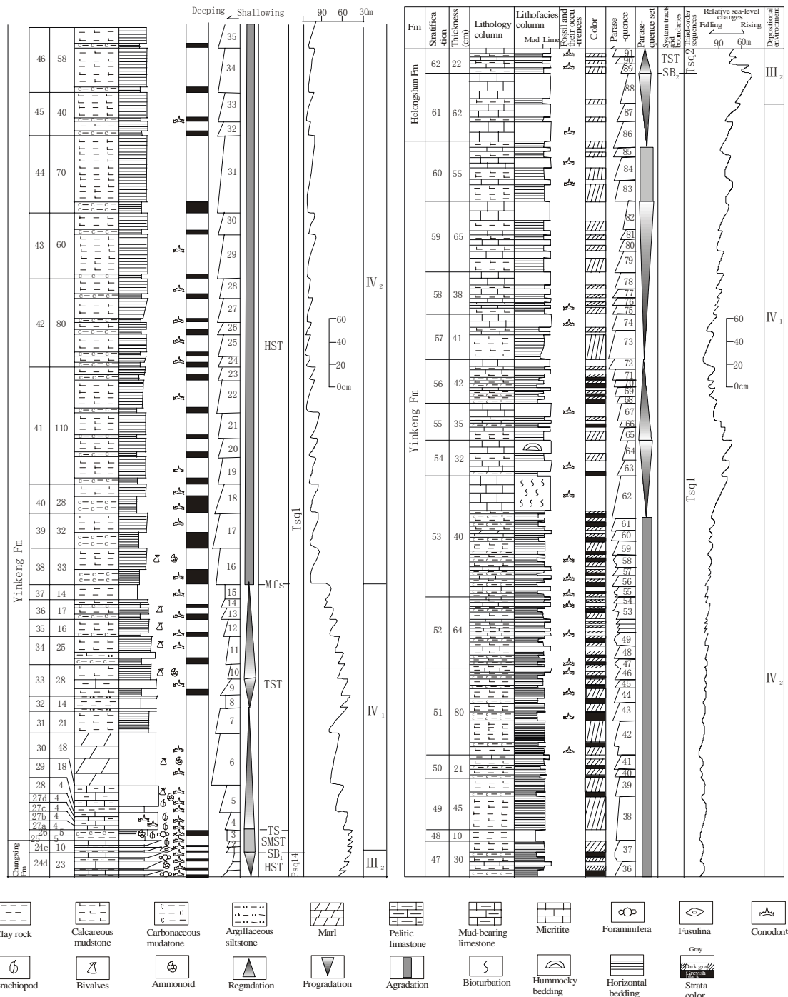
Figure 8. High-frequency cycles and sequence stratigraphy of the Yinkeng Formation at Meishan Section D
