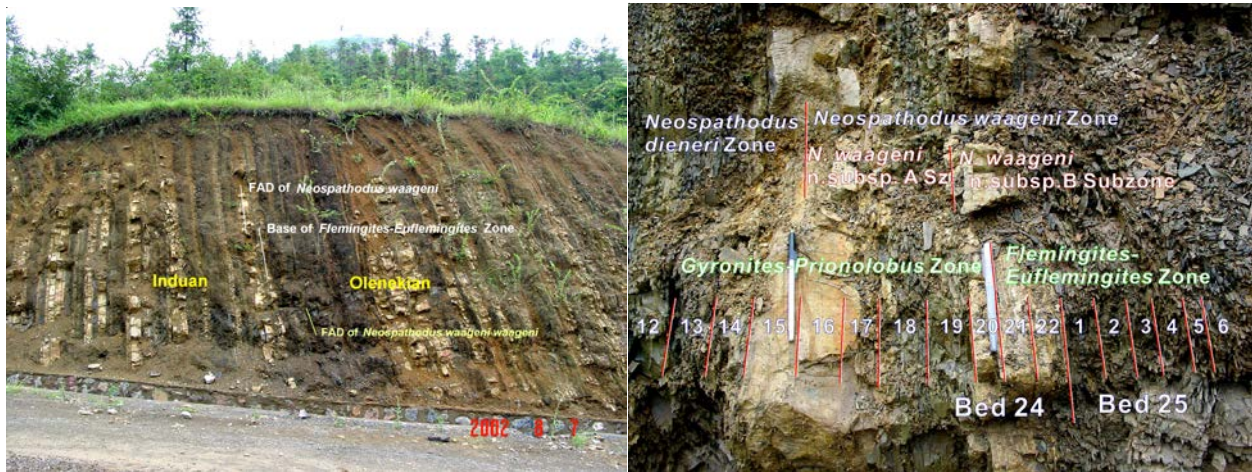
Figure 7. Induan-Olenekian boundary at the West Pingdingshan Section
