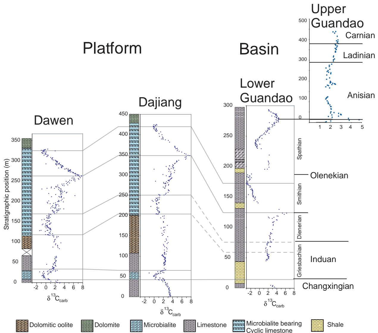
Figure 18: Carbonate isotope data from Upper Permian through Upper Triassic (Carnian) of the GBG (from Payne et al., 2004). Dawen and Dajiang sections are from the platform interior and lower and upper Guandao sections are from the basin margin (see figures 9 and 10 for section locations). Age correlations are based on conodont biostratigraphy from Guandao section and correlation of carbon isotope excursions.
