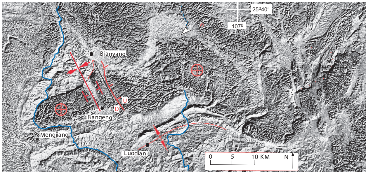
Figure 8: Landsat image of the Great Bank of Guizhou. The Bianyang syncline dissects the platform from Bianyang to Bangeng. Geological map of the east limb of the Bianyang syncline is shown in figure 9.
