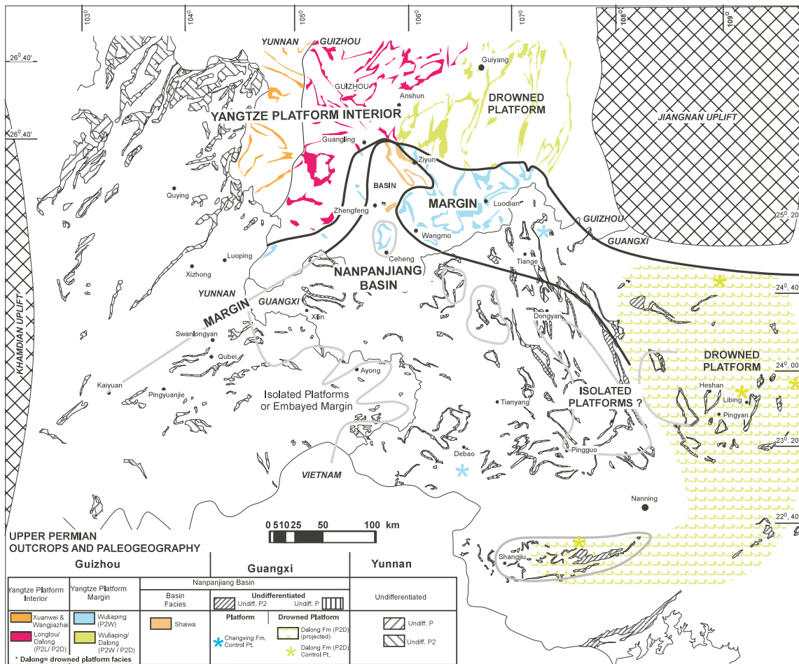
Figure 2: Upper Permian lithofacies and interpreted paleogeography of the Nanpanjiang basin and Yangtze platform in Guizhou, Guangxi, and Yunnan. Compiled from regional geologic maps of the Yunnan Bureau of Geology, 1984; Guangxi Bureau of Geology, 1985, and Guizhou Bureau of Geology, 1987. Maps have been modified and updated with results from our regional mapping. Data control (colored facies polygons) is the distribution of surface exposure of various facies (Formations) indicated in the legend.
