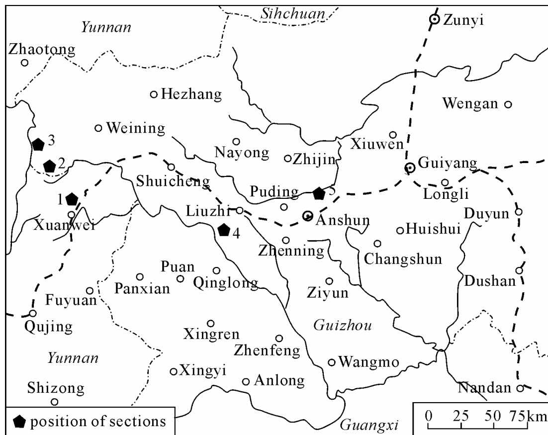
Figure 1. Location map of the field excursion and PTB sections 1-Laibin section, 2-Zhejue section, 3-Chahe section, 4-Zhongzai section, 5-Jiaozishan section; Sections 1, 2 and 3- terrestrial facies, Section 4-neritic clastic facies, Section 5-neritic carbonate facies. Sections 3 and 4 will be examined in this field excursion.
