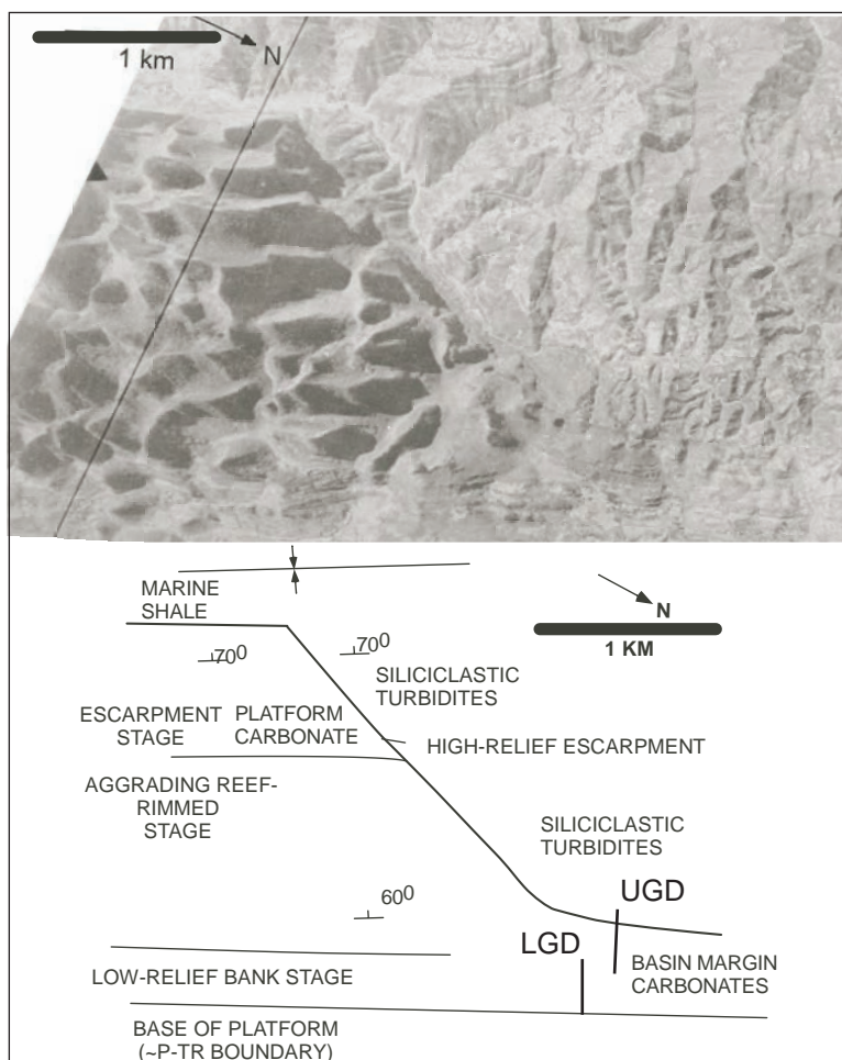
Figure 15: Air photo and sketch map of platform margin relationships on the northern margin in the Bianyang syncline (northern margin in figure 9). The air photo illustrates the sharp contact between carbonate strata of the high-relief Ladinian escarpment and onlapping Carnian siliciclastic turbidites. LGD = Lower Guandao section. UGD = Upper Guandao section. See text for details.
