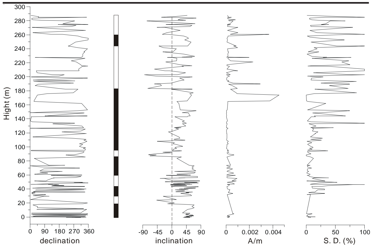
Figure 11. Stratigraphical plot of magnetic vectors and the corresponding interpreted polarity pattern
