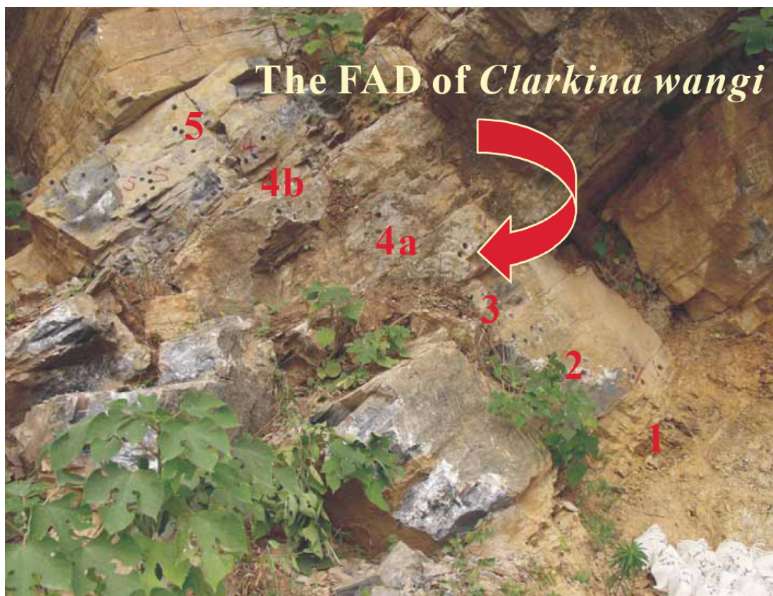
Figure 2. Proposed GSSP for the base of the Changhsingian at Meishan Section D
