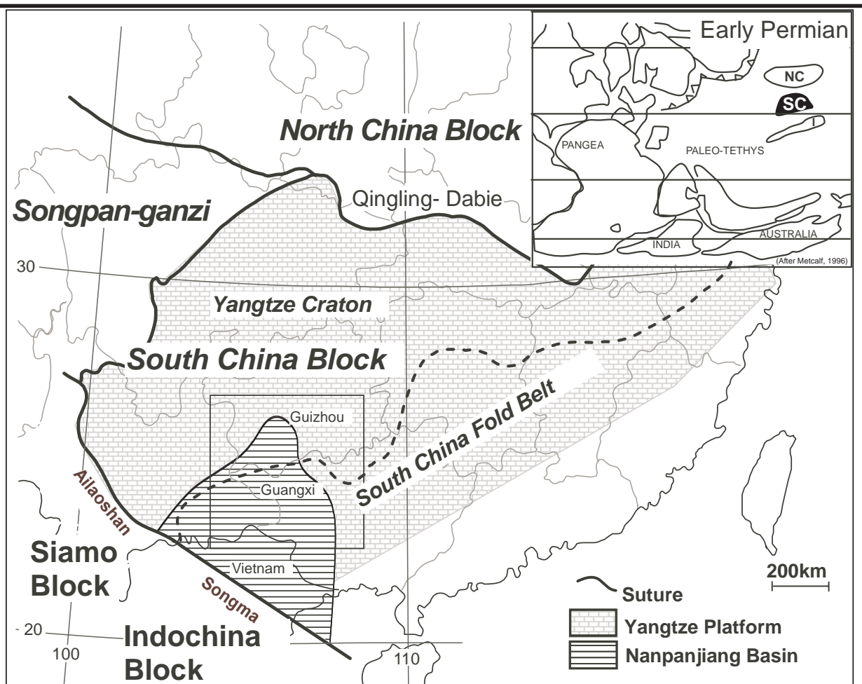
Figure 1: Tectonic map illustrating cratonic blocks (plates) of south China, interpreted suture zones and extent of the Nanpanjiang basin and Yangtze platform. South China block includes Yangtze craton and south China fold belt. Modified from Sun Shu et al., 1989. Inset, upper right illustrates global plate reconstruction and position of south China block (SC) in Early Permian. Modified from Metcalf, 1996.
