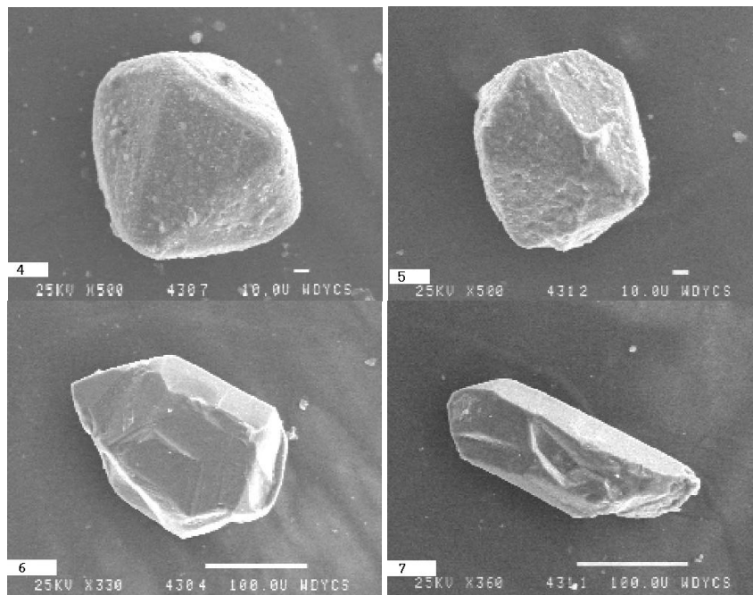
Figure 4 Volcanogenic minerals of the boundary claybeds 4 GWC-66f, \beta quartz; 5 GWC-68a, \beta quartz; 6 GWC-66f, zircon; 7 GWC-68a, zircon
