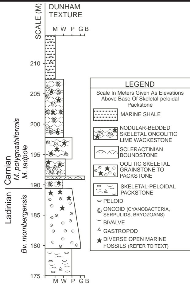
Figure 16: Stratigraphic section of the Ladinian-Carnian platform termination succession at the top of Bangeng section, in the axis of the Bianyang syncline. See figure 9 for location. See text and stop 2 of the field guide for further details.
