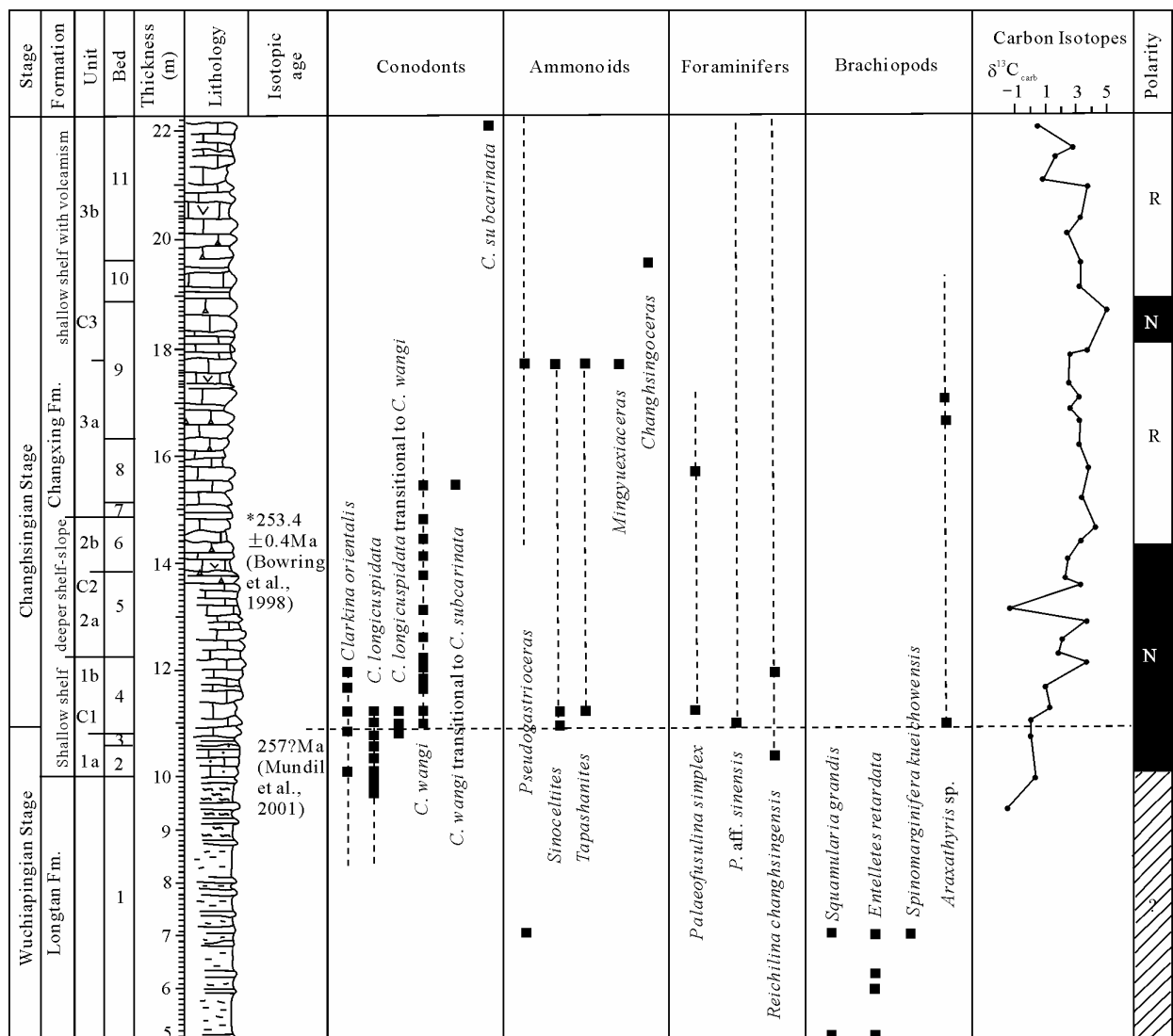
Figure 3. Integrated stratigraphic sequences around the Wuchiapingian-Changhsingian boundary in Meishan and the distribution of various fossil groups, carbon isotopes, geochronologic ages, and magnetic reversals. Note that the lithologic succession is subdivided into both beds and units. The beds are based on historical usage and are depicted to allow comparison with the literature. It is recognized that these beds are actually bedsets or parasequences except in the case of the ash beds, which represent true beds. The units are based on distinctive lithologic changes that reflect interpreted changes in depositional environment.
