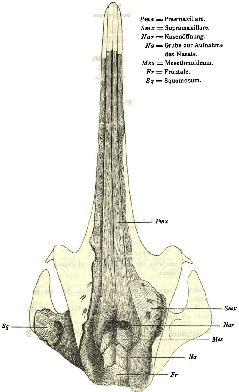
Saurodelphis argentinus Burmeister 1891.
