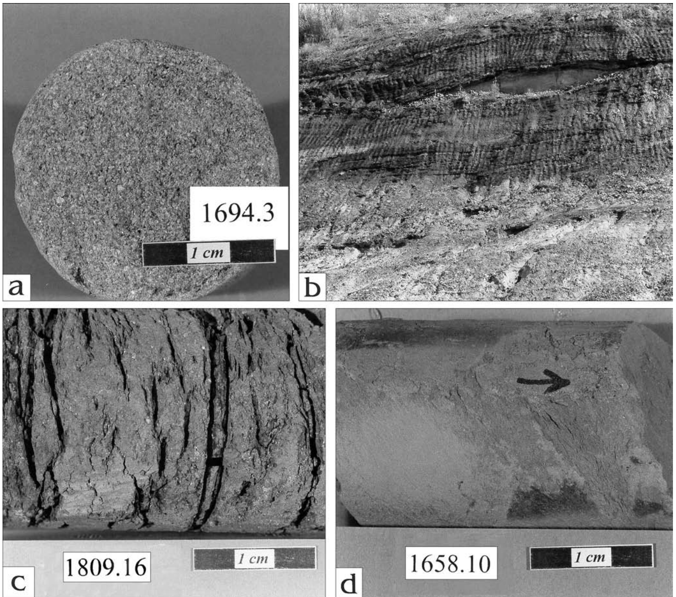
Text-Fig. 4. a) Core cross-section of well sorted fluviatile channel sands. b) Overbank sediments in the Piberstein-Lankowitz Depression with different types of intersected channels (for explanation see text). c) Typical core section from the overbank environment; medium-sorted silty sands (including organic debris) alternating with thin lignite layers. d) Silt-clay rhythmites from the Obergraden depression (arrow shows upwards core direction). Visibility of wave-like structures is better in wet fresh cores.
