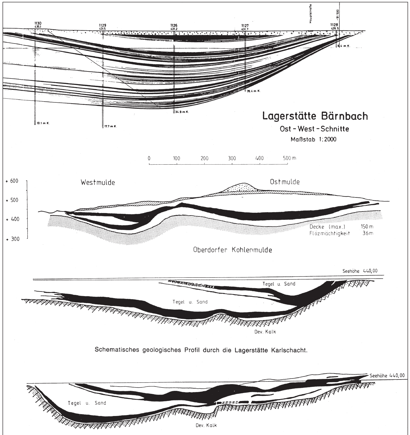
Text-Fig. 6. General sections through the Piberbach-Bärnbach Depression (above), the Oberdorf Depression (middle) and the Obergraden Depression (lowermost two).
