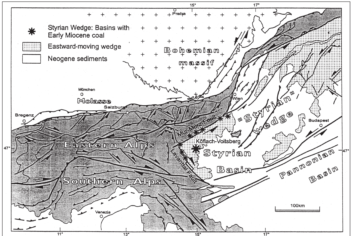
Text-Fig. 2. Tectonic sketch of the Styrian Wedge within the Eastern Alps and the Pannonian Basin. After HAAS et al. (1998) and PERESSON & DECKER (1997).
