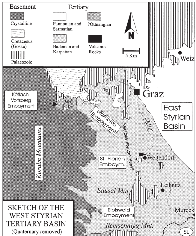
Text-Fig. 1. General sketch of the West Styrian Basin and position of the Köflach-Voitsberg Embayment.
