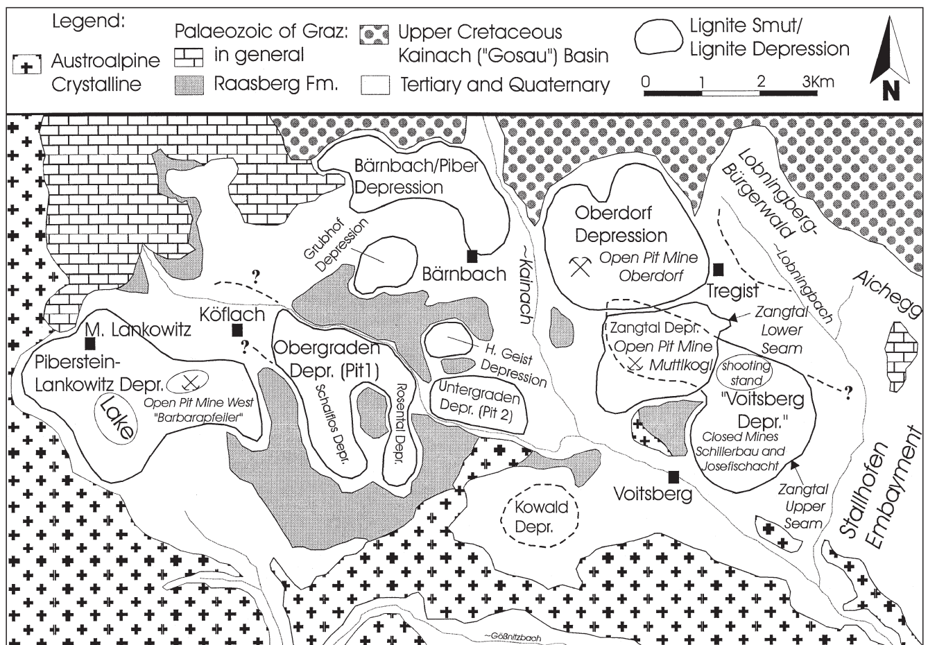
Text-Fig. 3. Basement lithologies and lignite depressions of the Köflach-Voitsberg Embayment.
