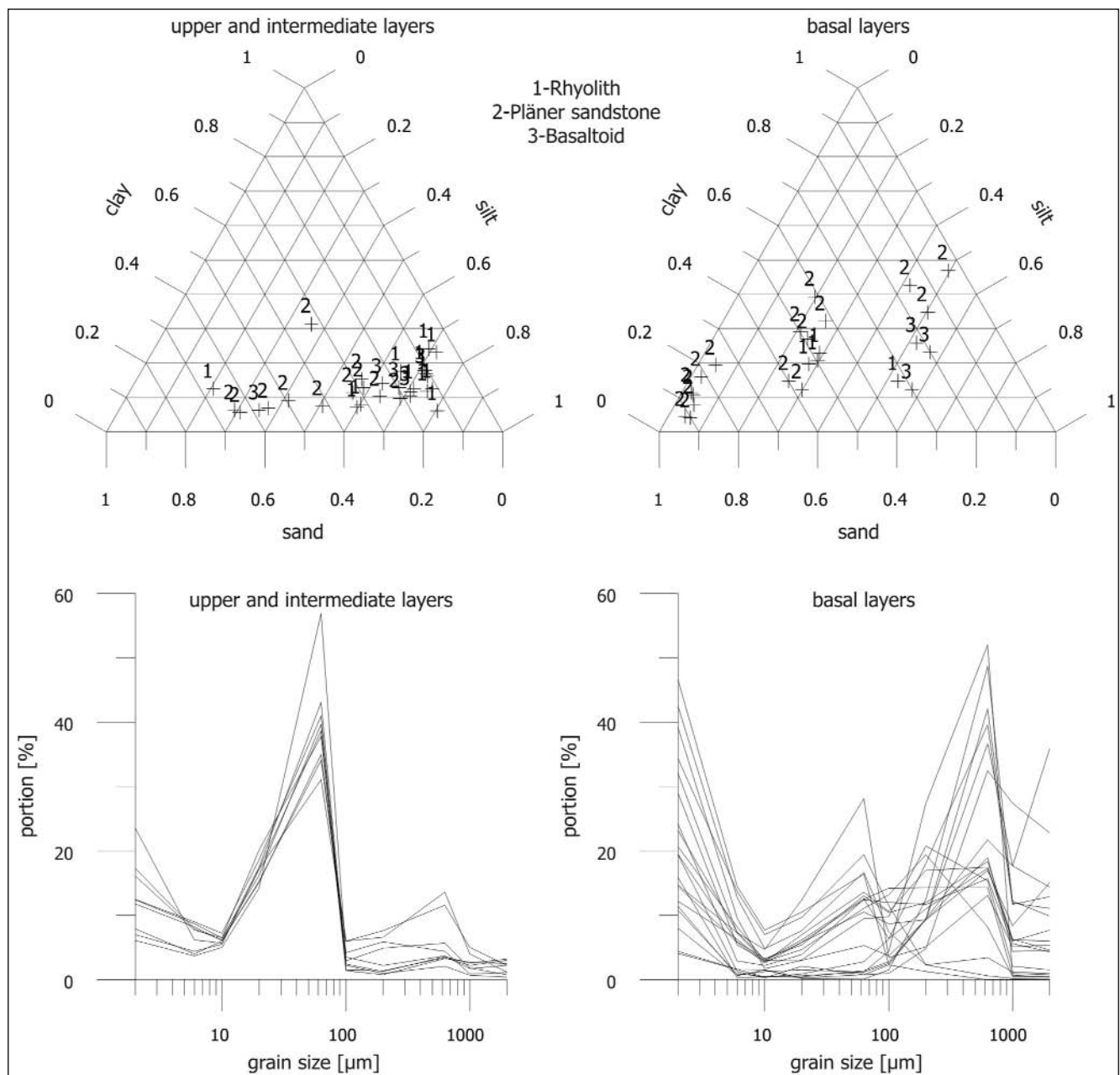
Text-Fig. 3. Comparison of grain size fractions of samples from distinct periglacial layers with respect to bedrock material. The loess-influenced upper and intermediate layers show no clear relationship to parent rock type but are dominated by grain sizes between 30 and 80 µm while basal layers can be grouped by their parent rock material and have a much more irregular grain size distribution. Original measurements of some granulometries are taken from TACHIVA (1996).
