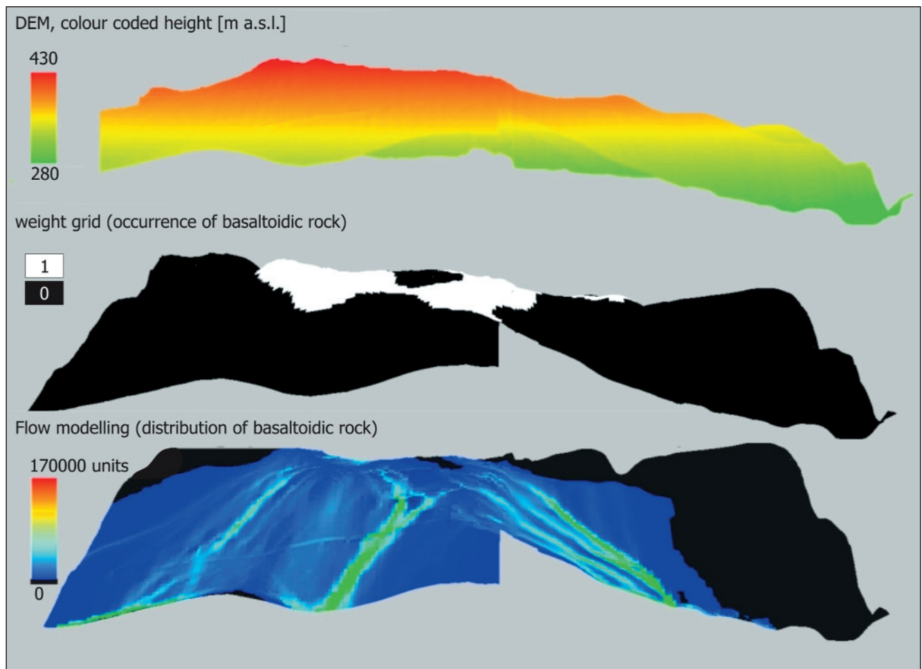
Text-Fig. 2. Model approach to describe topography-controlled downslope displacement of individual rock types. A modified flow distribution model (FREEMAN, 1991; OLAYA, 2004) uses digital elevation model data and weight grids representing initial locations of rock types to create solifluidal-like patterns of material redistribution.
