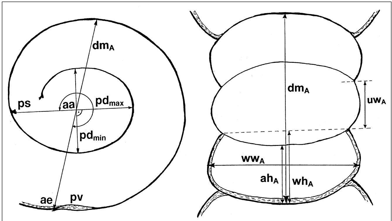
Text-Fig. 2. ▲ ▲ ▲ Schematic drawing of an ammonitella median section (left side) and a cross section (right side) with the measured parameters. The nacrosepta and the siphon are left out. aa = ammonitella angle; ae = ammonitella edge; ah A = apertural height of the ammonitella; dm A = ammonitella diameter; pd max = maximum protoconch diameter; pd min = minimum protoconch diameter; ps = proseptum; pv = primary varix; uw A = umbilical width of the ammonitella; wh A = whorl height of the ammonitella; ww A = whorl width of the ammonitella.
