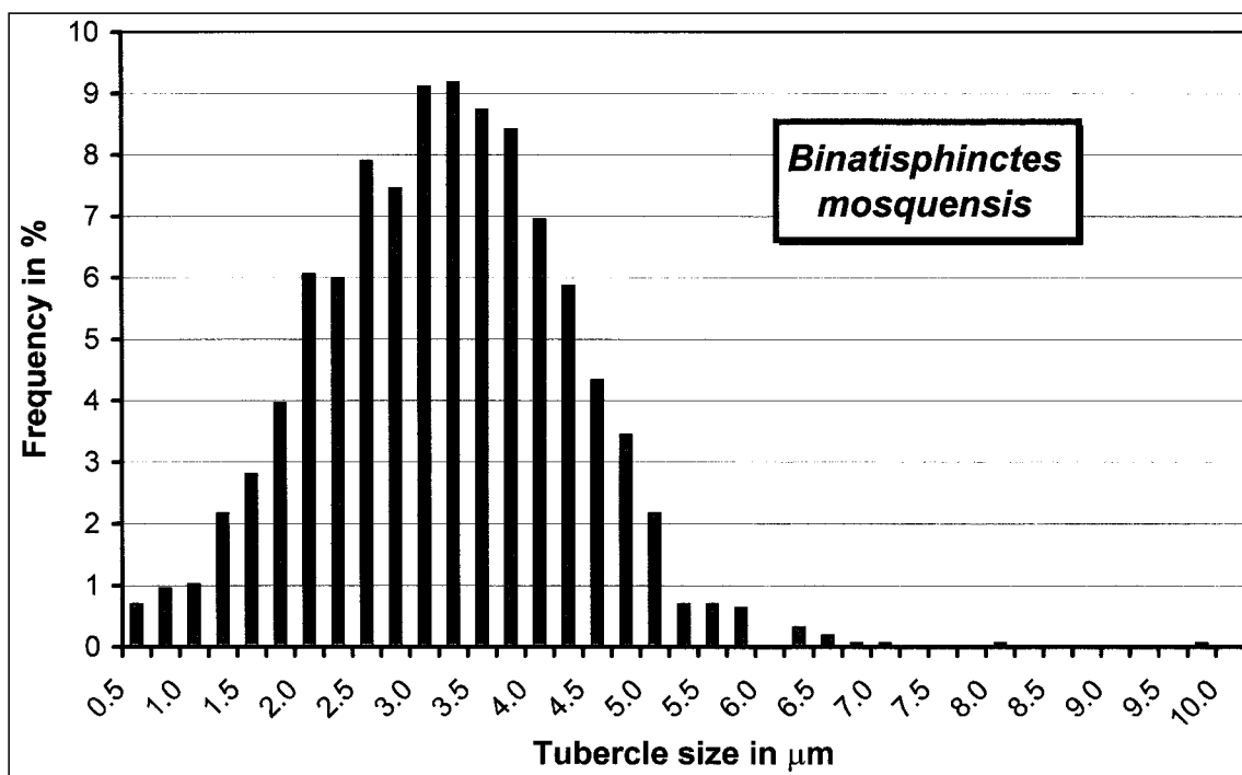
Text-Fig. 9. Frequency histogram of the tubercle size in the umbilical area of Binatisphinctes mosquensis .
