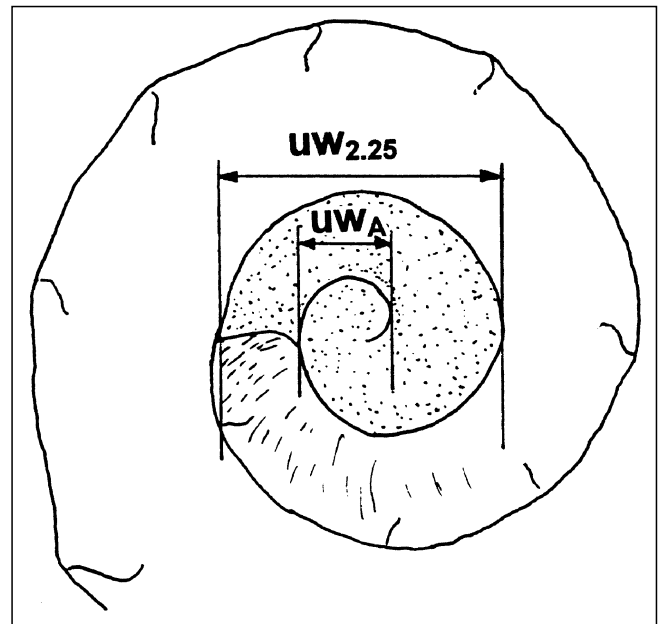
Text-Fig. 1. Definition of the distances measured in the centre of the umbilicus. uw_A = umbilical width of the ammonitella; uw_{2.25} = umbilical width of the juvenile stage with one additional whorl.
