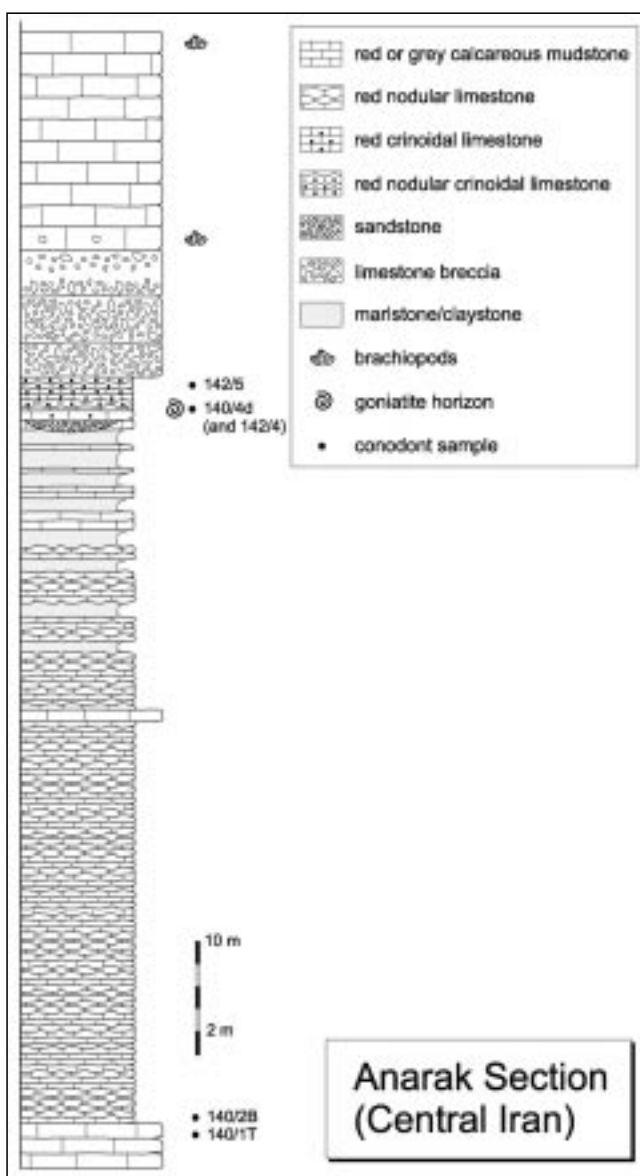
Text-Fig. 1. The Anarak section and the position of the goniatite-bearing horizons.
