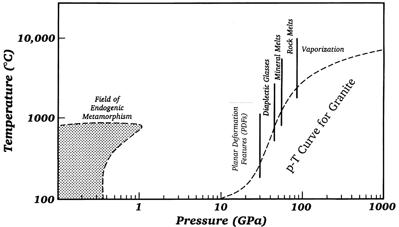
Text-Fig. 4. Pressure-temperature regime of endogenic metamorphism compared to shock metamorphism. Also indicated are the onset pressures of various irreversible structural changes in the rocks due to shock metamorphism. The dashed curve in the right part of the diagram shows the relation between pressure and post-shock temperature for shock metamorphism of granitic rocks. After GRIEVE (1987).
