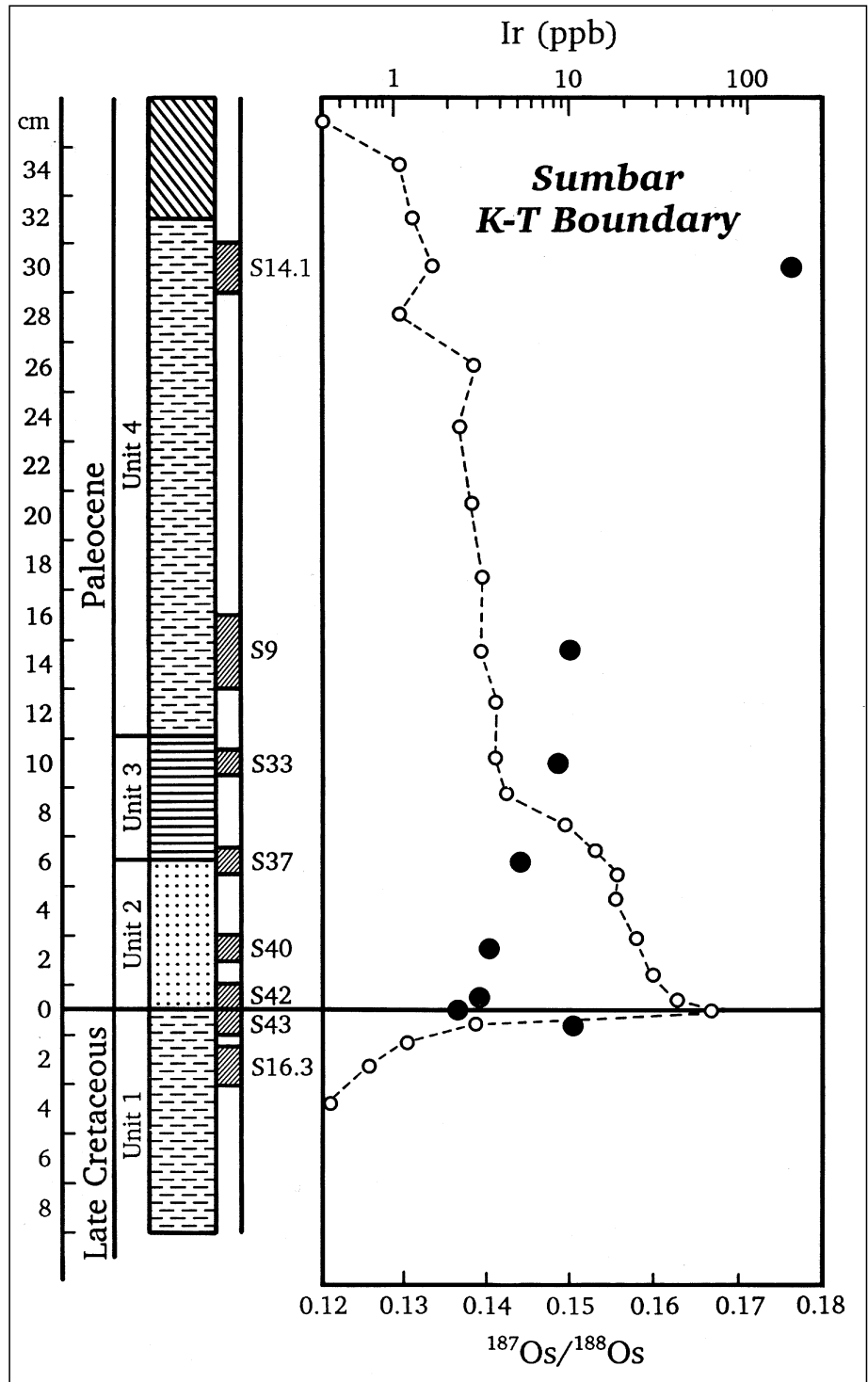
Text-Fig. 9. Profile of the distribution of Ir and the variation of the Os-isotopic composition across a K-T boundary profile in Sumbar, Turkmenistan. After MEISEL et al. (1993, 1995).
