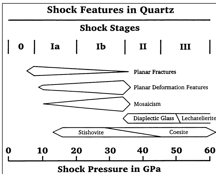
Text-Fig. 8. Pressure dependency of various characteristic shock indicators in quartz, and relation to shock stages. After STÖFFLER & LANGENHORST (1994).
