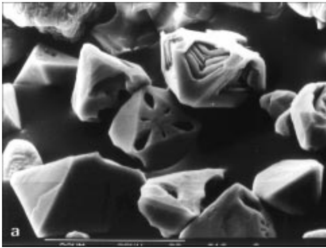
Text-Fig. 11. SEM images of spinel (magnesian ferrite) at the K-T boundary, which are interpreted as condensation products from meteoritic vapor or direct ablation products from the meteoritic bolide. a = Assemblage of magnesian ferrite grains from the Caravaca (Spain) K-T boundary; scale bar on bottom: 20 \mu\text{m} ; b = large single magnesian ferrite grain from the SDP Site 596 (SW Pacific) K-T boundary; grain diameter = 45 \mu\text{m} . Courtesy B. BOHOR (U.S. Geological Survey).
