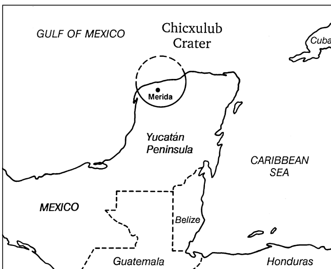
Text-Fig. 12. Geographical location of the Chicxulub impact structure on the NE part of the Yucatán (Mexico) peninsula. After KOEBERL (1993).
