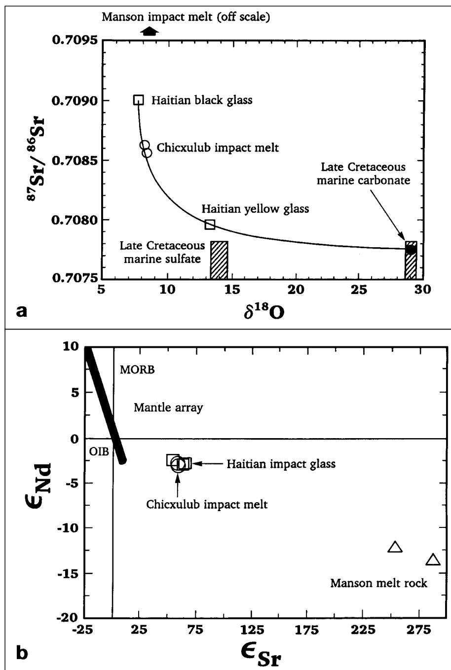
Text-Fig. 18. Isotope plots for Chicxulub melt rocks (after BLUM et al., 1993).
