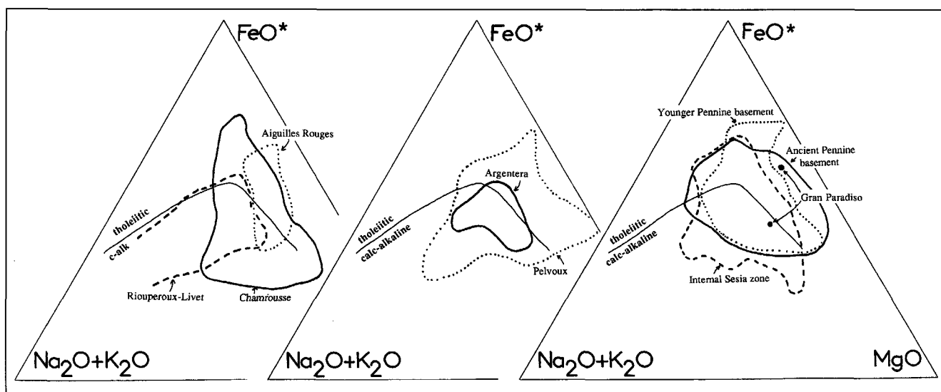
Fig. 3. AFM diagram for West-Alpine metabasites. Data from: MICHEL, 1953; VITERBO-BASSANI & BLACKBURN (1968); PÉCHER (1970); LEFORT (1973); LIÉBEAUX (1975); REINSCH (1977); LIÉGEOIS & DUCHESNE (1981); BODINIER et al. (1986); MÉNOT (1987); BIINO & POGNANTE (1989); DESMONS & PLOQUIN (1989); PAQUETTE et al. (1989b). Boundary curve between tholeiitic and calc-alkaline trends according to IRVINE & BARAGAR (1971).
