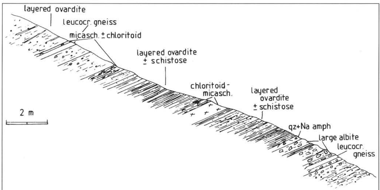
Fig. 2. Example of lithostratigraphic section through a banded metabasic outcrop (chlorite-epidote-albite-actinolite rock, possible meta-pyroclastite) in the Briançon zone, Ruitor massif, Valgrisanche (NW Italy). Note the interlayered mica-schists ± chloritoid.
