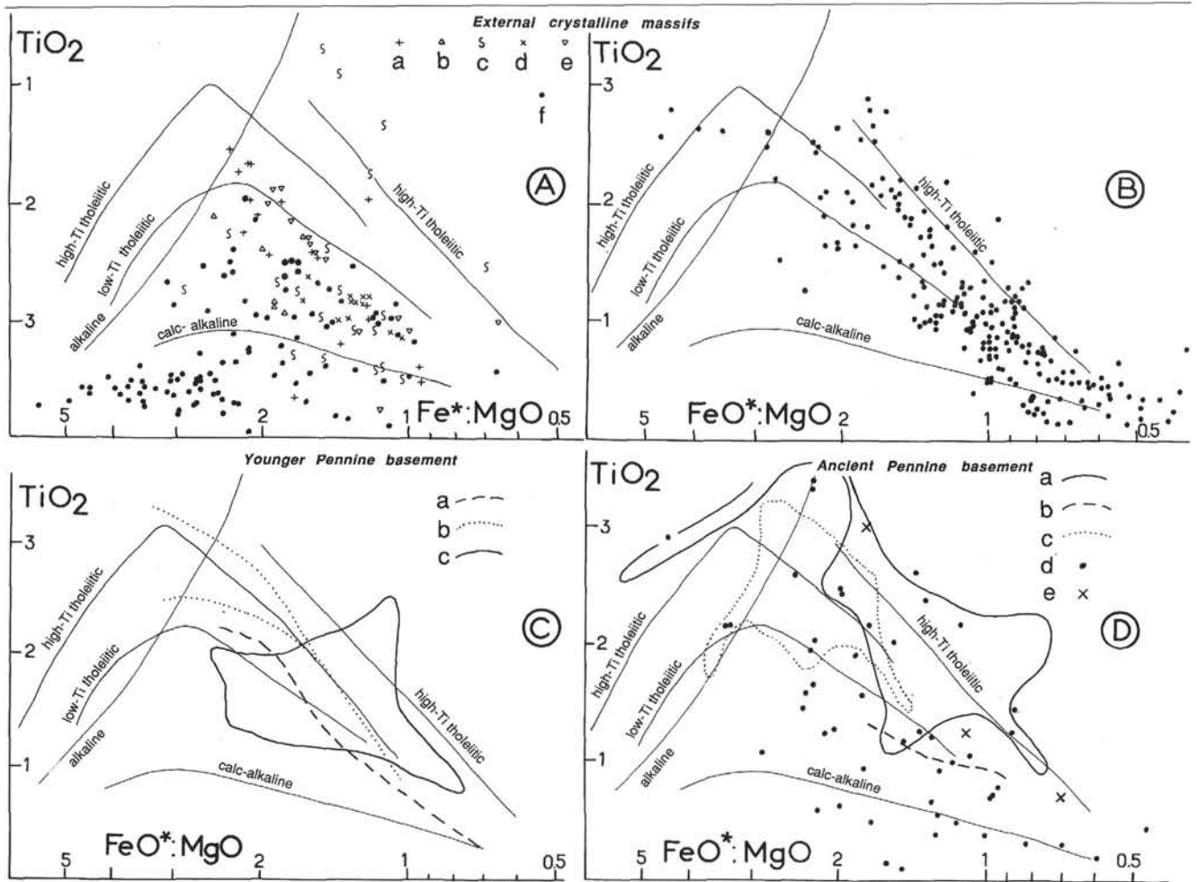
Fig. 4. \text{TiO}_2 - \text{FeO}^*/\text{MgO} diagram. A) (a) Aiguilles Rouges, (b) NE Belledonne, (c) eastern Pelvoux (core), (d) western Pelvoux (Chaillol series), (e) Argentera, (f) Riouperoux-Livet formation. B: Chamrousse metabasalt and metagabbro. C: Younger Pennine basement: (a) plutonic-volcanic body of the lower Bellecôte unit, (b) sills of the upper Bellecôte unit, (c) Ambin formation and Acceglio. D: Ancient Pennine basement: (a) Ruitor and Pontis, (b) Siviez-Mischabel, including Barneuzza; (c) Chasseforêt, southern Vanoise, (d) Sesia zone, (e) Gran Paradiso. Data source listed in Fig. 3. Reference trends (MORB-type high-Ti tholeiite, island-arc-type low-Ti tholeiite, calc-alkaline and alkaline) are as delineated by PLOQUIN, cf. GUILLLOT et al. (1986).
