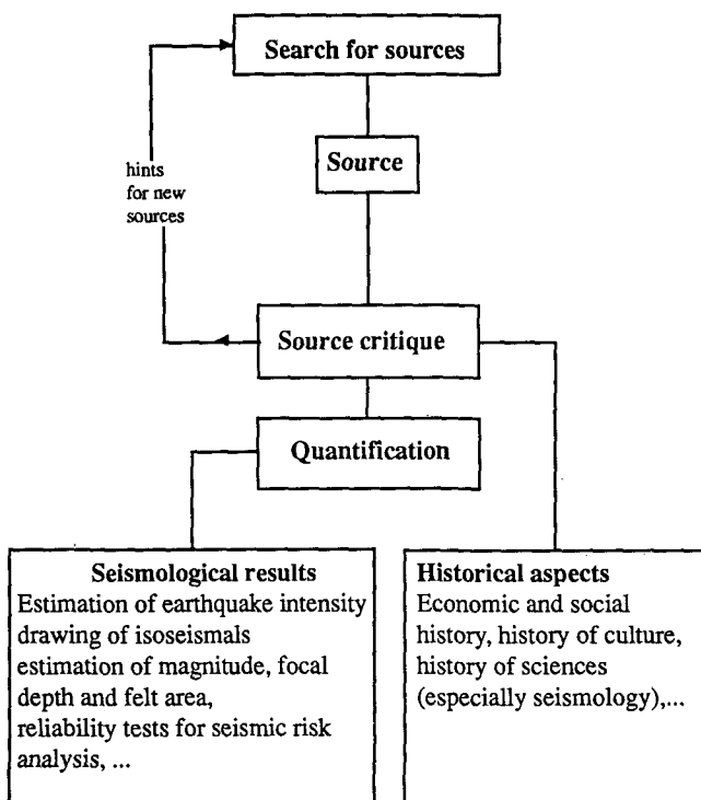
Figure 3. Flow chart of methods of Historical Earthquake Research.
