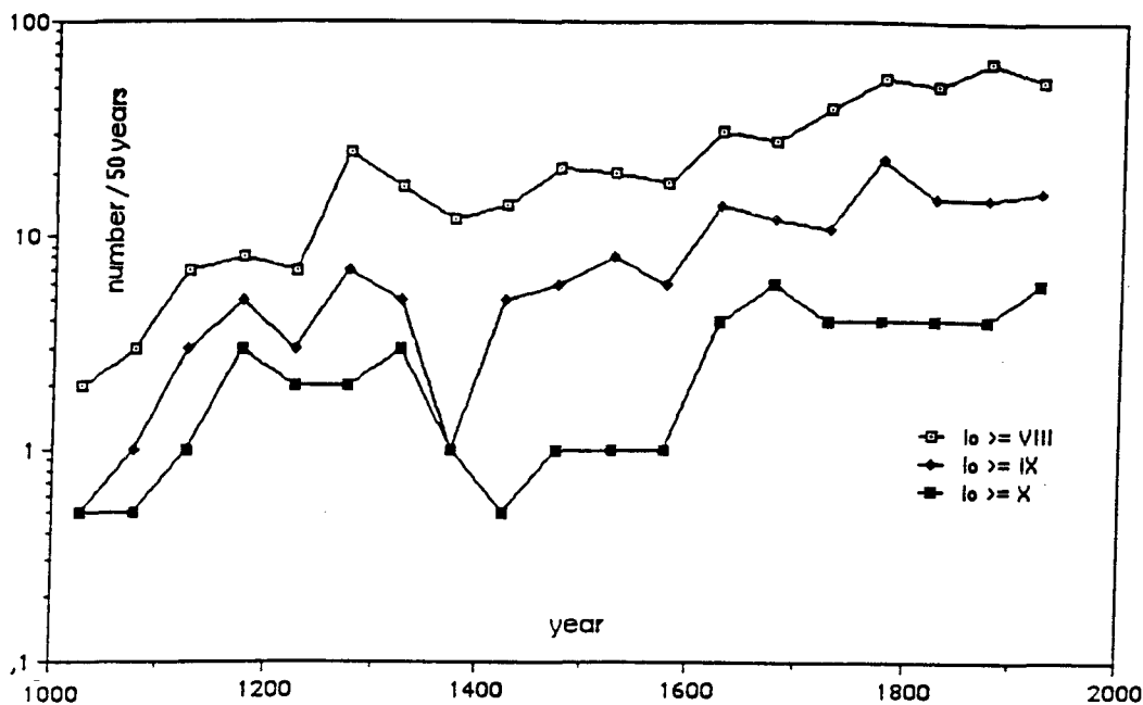
Figure 9. Number of earthquakes per 50 years in Italy. After POSTPISCHIL et. al. (1985). 1 = maximum intensity \geq VIII^\circ ; 2 = maximum intensity \geq IX^\circ ; 3 = maximum intensity \geq X^\circ .
