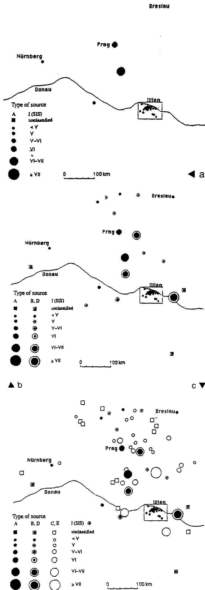
Figure 5. Spatial distribution of reports of the earthquake Sept. 15.–16., 1590.
