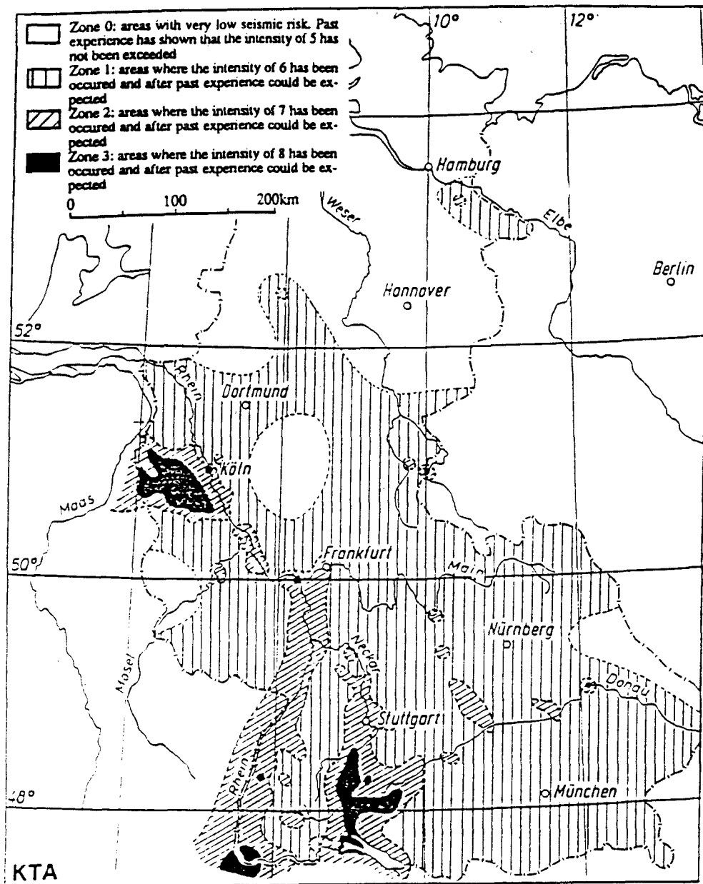
Figure 2. Zones of probable maximal intensities in the FRG, based on earthquake data from the last 1000 years. The number of big earthquakes is too small for a statistical covered conclusion about the seismic hazard. The high intensity values in SW-Germany come from the only big earthquake happened 1356 next to Basel. Today this map is regarded as a first information only. In every case of risk assessment a thorough study of seismic and tectonic situation of the site is needed.
