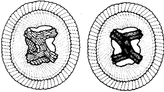
Fig. 3: Chiasmolithus bidens .
