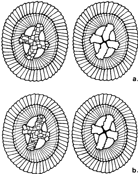
Fig. 6a-b: Chiasmolithus edwardsii nov. comb.
