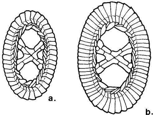
Fig. 14 a) Neochiastozygus saepeus , early form. b) Neochiastozygus saepeus , late form.
