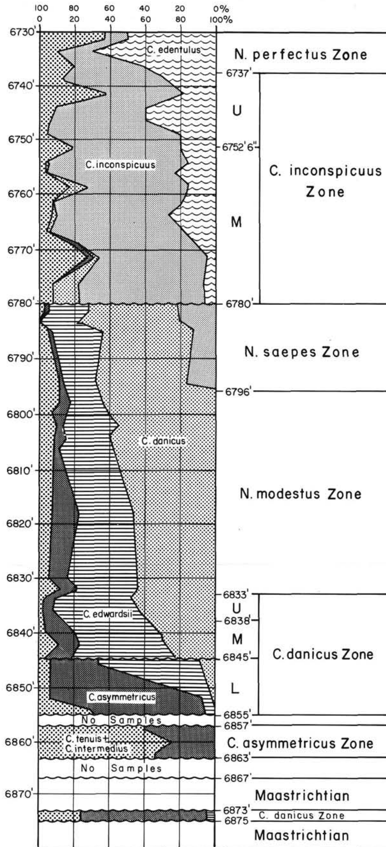
Fig. 20: Quantitative development of the „C-2“ assemblage in Danish North Sea well E-1X.
