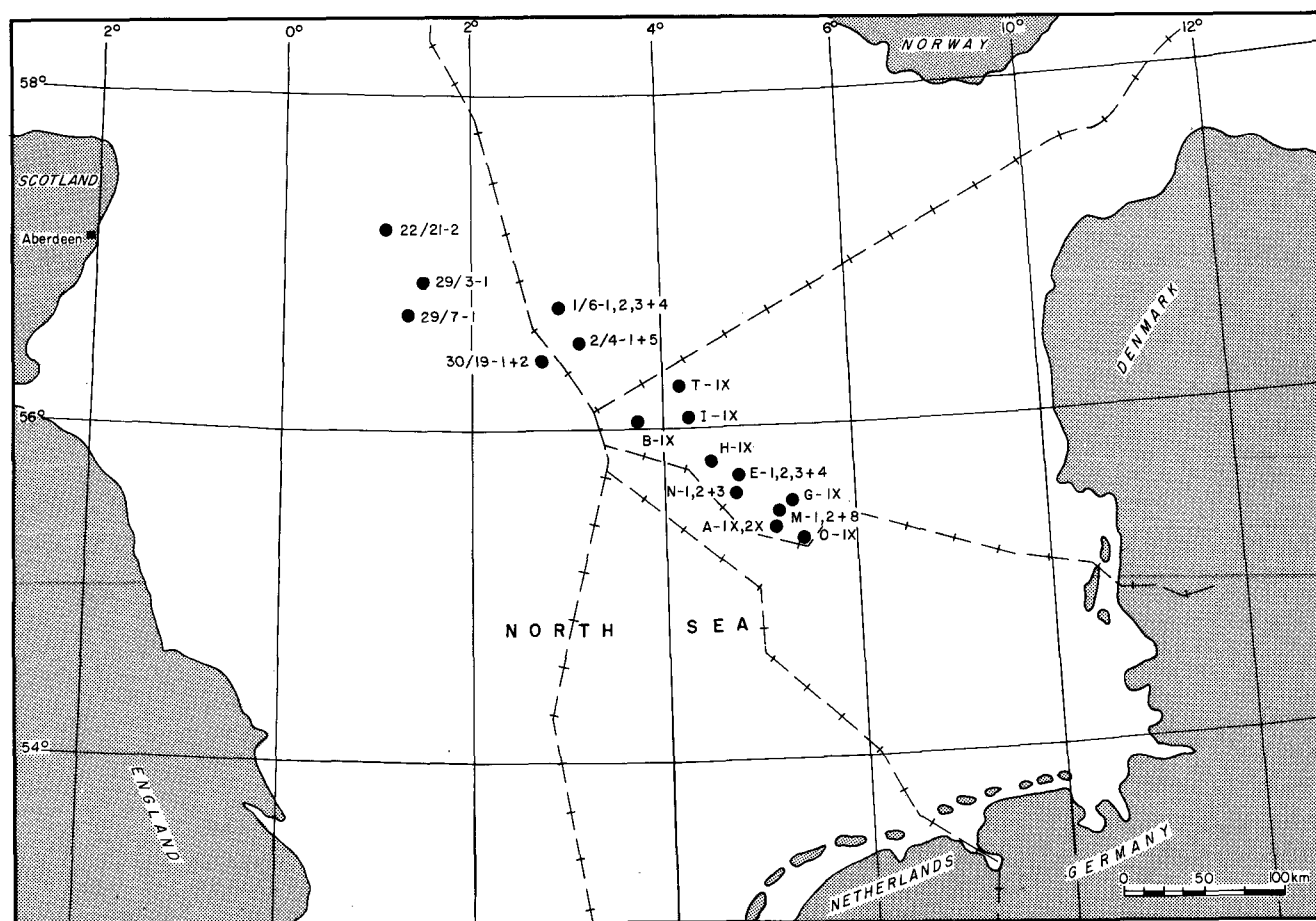
Fig. 1: Locations of the wells in the Central North Sea from which the Danian Chalk has been studied.
