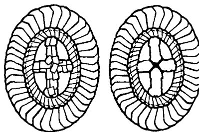
Fig. 10: Cruciplacolithus primus .
