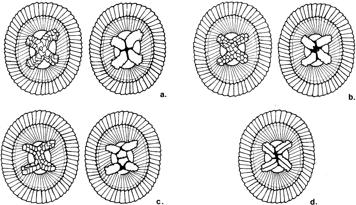
Fig. 4a–d: Chiasmolithus danicus .
