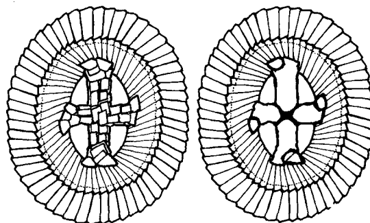
Fig. 11: Cruciplacolithus tenuis .
