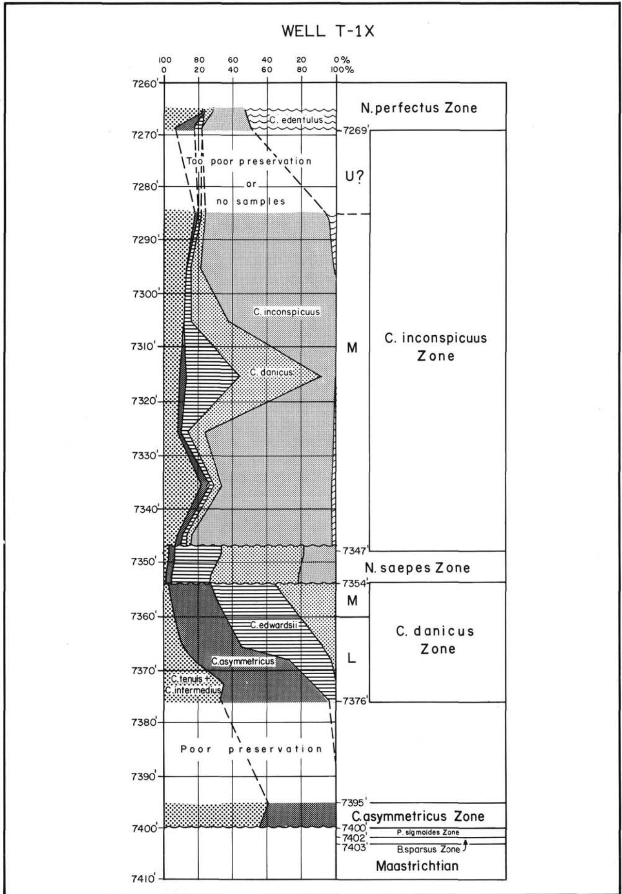
Fig. 18: Quantitative development of the „C-2“ assemblage in Danish North Sea well T-1X.
