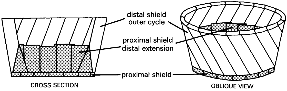
Fig. 2: Schematic diagram illustrating the characteristic features of the loxolith and protolith rim structure groups.
