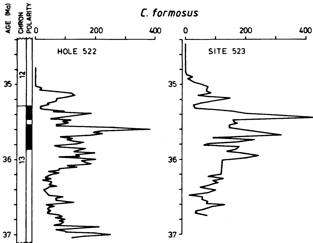
Fig. 2: Plots of the abundance of C. formosus versus age in Hole 522 and Site 523. The abundance scale is expressed as number of specimens per square mm times the accumulation rate (cm/1000 years).
