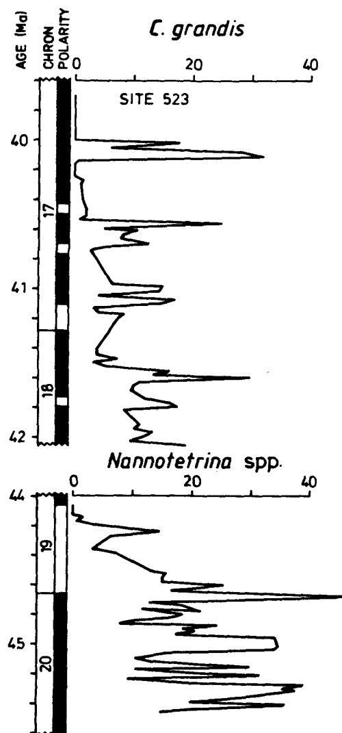
Fig. 9: Plots of the abundance of C. grandis and Nannotetrina spp. versus age in Site 523.
