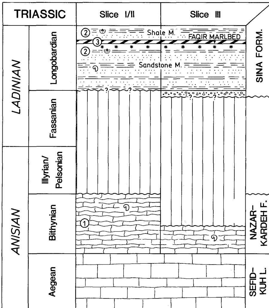
Text-Fig. 2. Middle Triassic stratigraphy of Aghdarband showing the positions of fossil levels 1 + 3. Note the presumed gap in the Upper Anisian and the Lower Ladinian.
