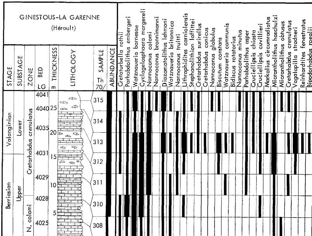
Fig. 4. Distribution of calcareous nannofossils in the section of Ginestous-La Garenne (Hérault).
