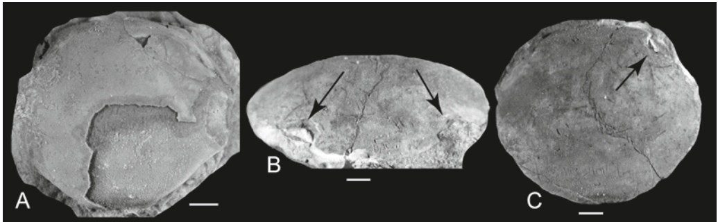
Fig. 6. Braggiarpilius wanzenboecki new species. A , paratype NHMW-Geo 2022/0289/0027, dorsal carapace; B , cast (NHMW-Geo 2022/0289/0026) of the holotype, anterior view of front and orbits; C , cast (NHMW-Geo 2022/0289/0026) of the holotype, dorsal view. Arrows indicate orbits. Scale bars equal 1 mm.
