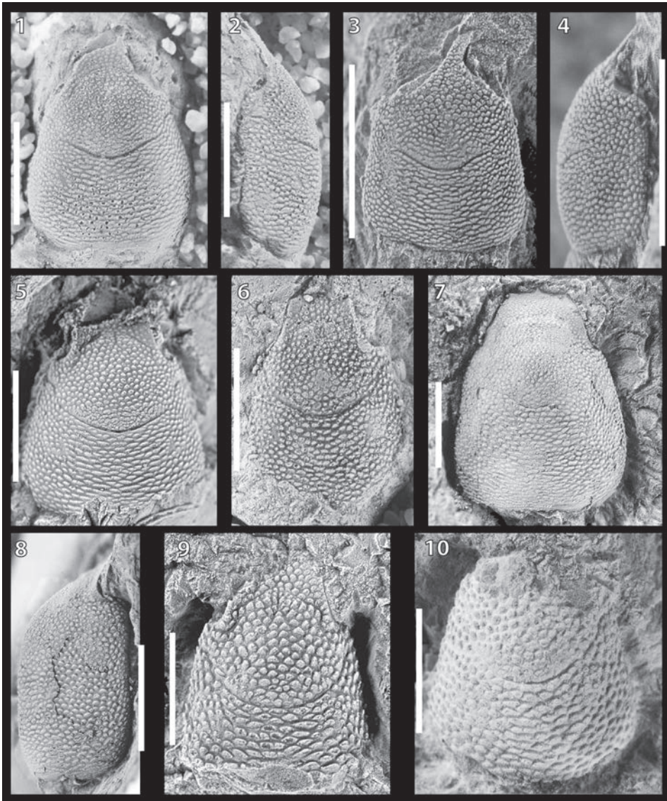
Fig. 3. 1–2: Cast of the lectotype of Paragalathea verrucosa (MOERICKE, 1889) from the Štramberk Limestones of Wilamowice, Poland (KSU D635). 1: dorsal view; 2: side view. 3: Paragalathea verrucosa (NHMW 2007z0149/0067) from the Ernstbrunn Limestones. 4–5: Specimen of Paragalathea verrucosa (NHMW 2007z0149/0071) from the Ernstbrunn Limestones. 4: dorsal view; 5: side view. 6: Cast of the holotype of P. ornatissima PATRULIUS, 1966 (KSU D472) from Woźniki, Poland. 7–8: Holotype of Paragalathea arcella nov. spec. (NHMW 2007z0149/0072) from the Ernstbrunn Limestones. 7: dorsal view; 8: side view. 9: Holotype of Paragalathea crenarvina nov. spec. (NHMW 2007z0149/0069) from the Ernstbrunn Limestones. 10: Paratype of Paragalathea crenarvina nov. spec. (two numbers: P129/54 and 11866) from the Štramberk Limestones. This specimen was whitened, but not dyed, prior to the photograph. Scale bars for 1–3 and 6–10 equal 5 mm, those for 4–5 equal 2 mm.
