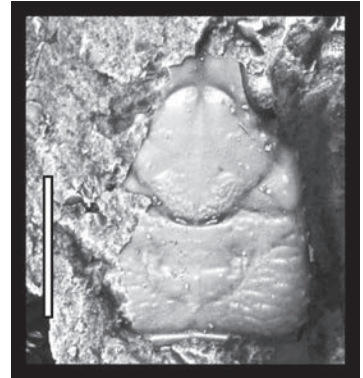
Fig. 13. Holotype of Hispanigalatea tithonia (NHMW 2007z0149/0438) from the Ernstbrunn Limestones. Scale bar equals 5 mm.
