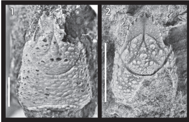
Fig. 18. 1: Holotype (MGSB 28118) and 2: an additional individual (MAB k2977) of Serraphylctaena multisquamata (VIA BOADA, 1981) nov. gen. The individual shown in 2 was also illustrated in KLOMPMAKER et al. (2012: p. 135, fig. 6A). Scale bars equal 2 mm.
