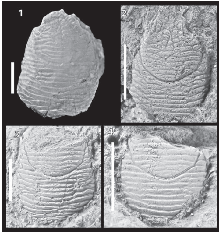
Fig. 8. 1: Lectotype of Discutiolira eutecta (MOERICKE, 1889) nov. comb. (BSP AS III 318) from the Štramberk Limestones of Myslowice, Poland. 2: Holotype of Galathea substriata BLASCHKE, 1911 nov. syn. (NHMW 1910/0005/0035) from the Štramberk Limestones, which should be considered the junior synonym of Discutiolira eutecta nov. comb. 3–4: Examples of Discutiolira eutecta nov. comb. from the Štramberk Limestones of the Kotouč Quarry in Štramberk, Czech Republic (3: NHMW 2012/0129/0001; 4: NHMW 2012/0129/0002). All scale bars equal 5 mm.
