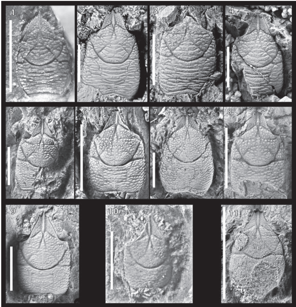
Fig. 12. 1: Lectotype of Galatheites zitteli (MOERICKE, 1889; BSP ASIII308) from the Štramberk Limestones of Wiślica, Poland. Photo courtesy of A. KLOMPMAKER. 2: Example of Galatheites zitteli (NHMW 2007z0149/0414). 3: Example of Galatheites zitteli (NHMW 2007z0149/0416). 4: Example of Galatheites zitteli (NHMW 2007z0149/0415). 5: Paratype of Galatheites aiola nov. spec. (NHMW 2007z0149/0440), showing strong groove structure and a three-pronged rostrum. 6: Paratype of Galatheites aiola nov. spec. (NHMW 2007z0149/0441), showing a presumed three-prong rostrum, well-developed groove structure, and a well preserved posterior carapace. 7: Paratype of Galatheites aiola nov. spec. (NHMW 2007z0149/0412), showing weak groove structure and a five-prong rostrum. 8: Holotype of Galatheites aiola nov. spec. (NHMW 2007z0149/0437), showing strong groove structure and a five-pronged rostrum. 9: Holotype (NHMW 2007z0149/0434) and 10: Paratype (NHMW 2007z0149/0163) of Galatheites diasema nov. spec. 11: Holotype of Galatheites obiecta nov. spec. (LPBIIIart134) from Purcăreni, Romania. All figured specimens except 1 and 11 are from the Ernstbrunn Limestones. Scale bars for 1–4, 6–8, and 11 equal 5 mm, those for 5 and 9–10 equal 2 mm.
