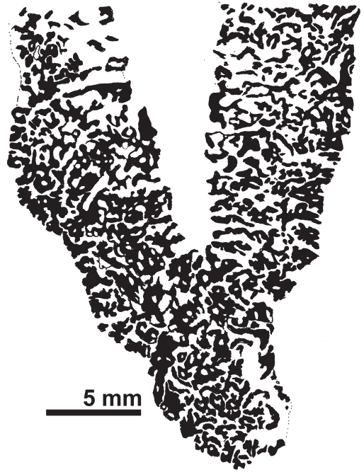
Fig. 9. Permocorynella cf. P. maxima SENOWBARI-DARYAN, SEYED-EMAMI & AGHANABATI, 1997. The longitudinal section shows the reticulate fiber skeleton of the wall and a few inhalant and exhalant canals within the wall (drawn from Pl. 6, Fig. C).
