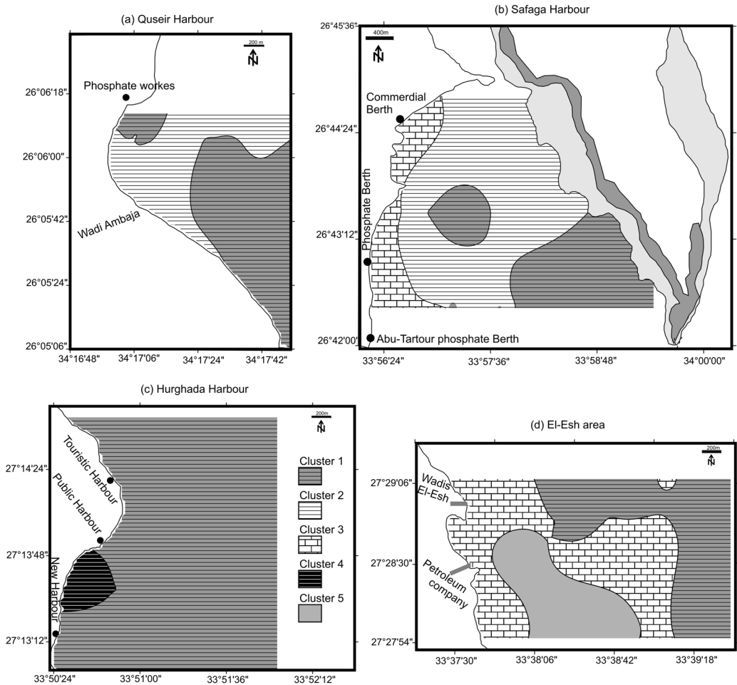
Fig. 8. Distribution of clusters according to trace metals of Harbours of (a) Quseir, (b) Safaga, (c) Hurgada and (d) El-Esh area.
