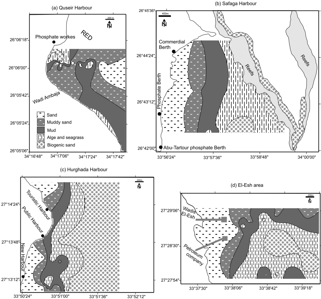
Fig. 3. Bottom facies maps of the Harbours of (a) Quseir, (b) Safaga, (c) Hurgada and (d) El-Esh area.
