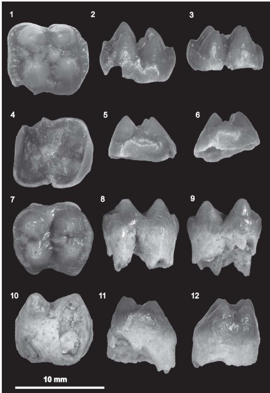
Fig. 3. Albanohyus cf. pygmaeus (DEPÉRET, 1892) from Atzelsdorf, Late Miocene (MN9). Scale bar equals 10 mm.
