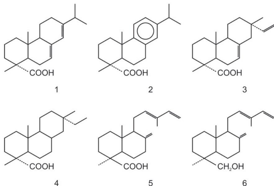
Fig. 2: Examples for diterpenoid resin acids and communol: (1) abietic acid, (2) dehydroabietic acid, (3) isopimaric acid, (4) sandaracopimaric acid, (5) communic acid, (6) communol.
