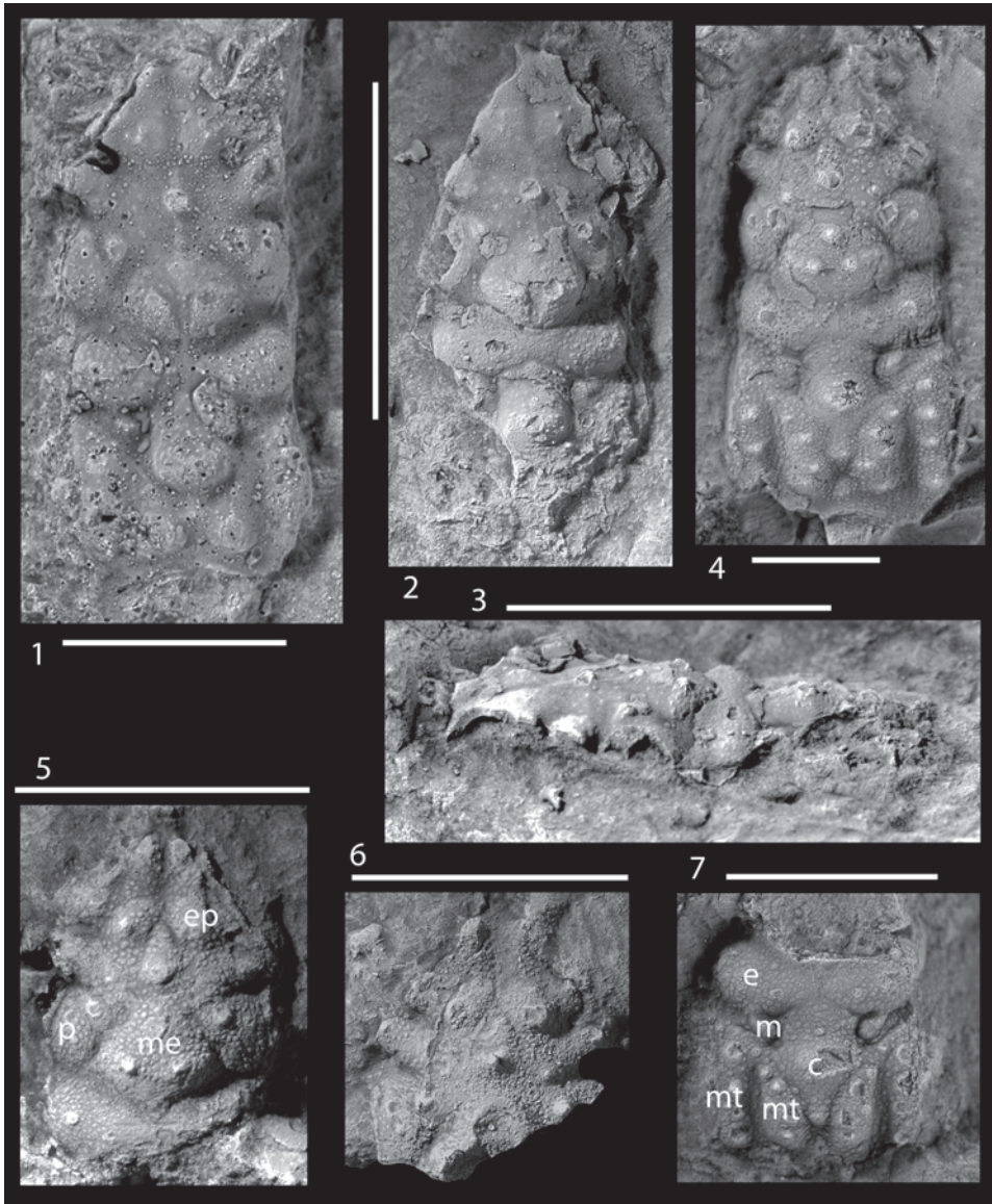
Fig. 5. Tenuihomola spp. 1-3, Tenuihomola longa (MOERICKE, 1897). 1, dorsal view of plaster cast of holotype, BSPAS III 321, from the Upper Jurassic Štrambersk Limestone, near Štrambersk, Czech Republic. 2, 3, Dorsal and lateral views of NHMW 1990z0041/0770, from the Ernstbrunn Limestone (Tithonian) from near Dörfles, Austria. 4-7, Tenuihomola ortwini nov. spec. from the Ernstbrunn Limestone (Tithonian) from near Dörfles, Austria. 4, dorsal view of holotype, NHMW 2007z0149/0017. 5, dorsal view of anterior part of carapace, paratype NHMW 1990z0041/0316, showing placement of anterior regions. ep = epigastric region; me = mesogastric region; p = protogastric region. 6, dorsal view of rostral area and left orbital region, paratype NHMW 1990z0041/2915. 7, dorsal view of posterior part of carapace, paratype NHMW 2007z0149/0016, showing placement of posterior regions. c = cardiac region; e = epibranchial region; m = mesobranchial region; mt = metabranchial region. Scale bars equal 5 mm.
